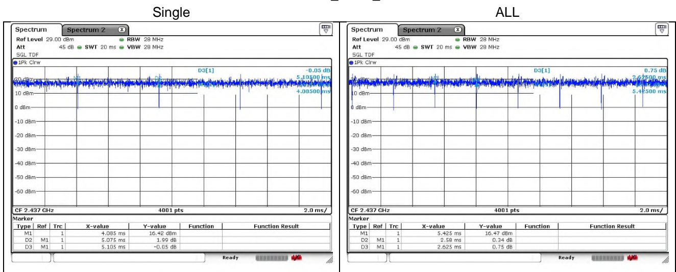
802.11ax_HE20_26T
