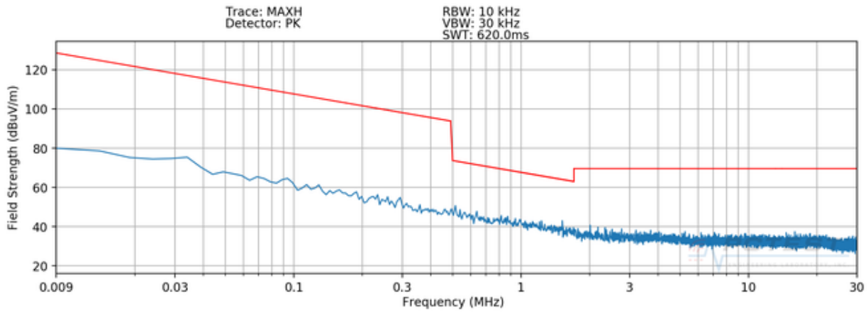
Plot 7-1. Radiated Spurious Plot 9kHz – 30MHz (Pol. X – Device to S-Pen WPT)
