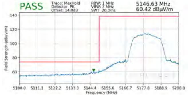
Plot 7-214. Radiated Lower Band Edge Plot MIMO (Peak – UNII Band 1)
