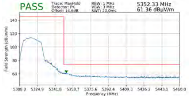
Plot 7-216. Radiated Upper Band Edge Plot MIMO (Peak – UNII Band 2A)
