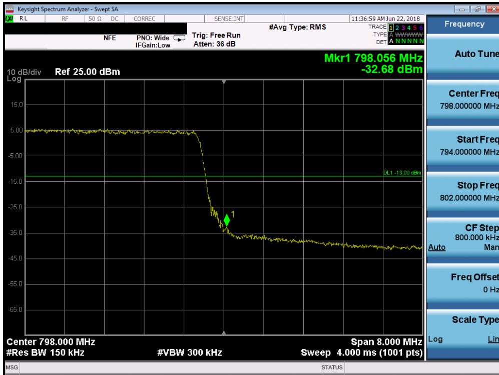
Plot 7-22. Upper Band Edge Plot (LTE Band 14, 10MHz QPSK – RB Size 50)
