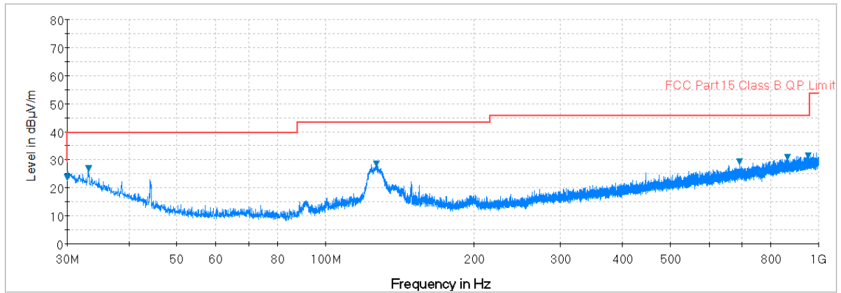
Plot 7-92. Radiated Spurious Plot below 1GHz (Pol. V)
