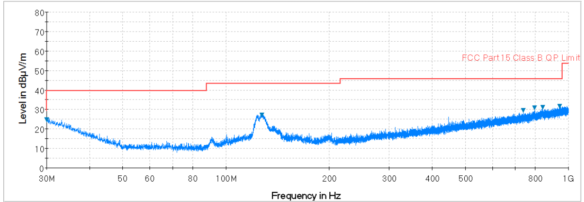
Plot 7-91. Radiated Spurious Plot below 1GHz (Pol. H)
