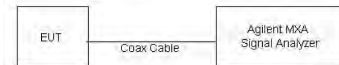
Figure 8-5 Power Measurement Setup for Bandwidths > 50 MHz
