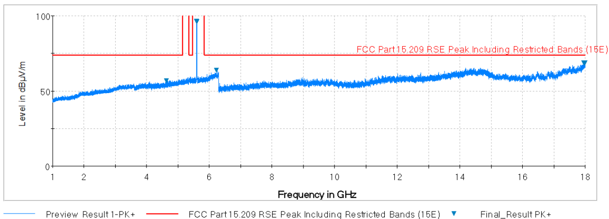
Plot 7-173. Radiated Spurious Plot above 1GHz (802.11a – U2C Ch. 120, Ant. Pol. H)
