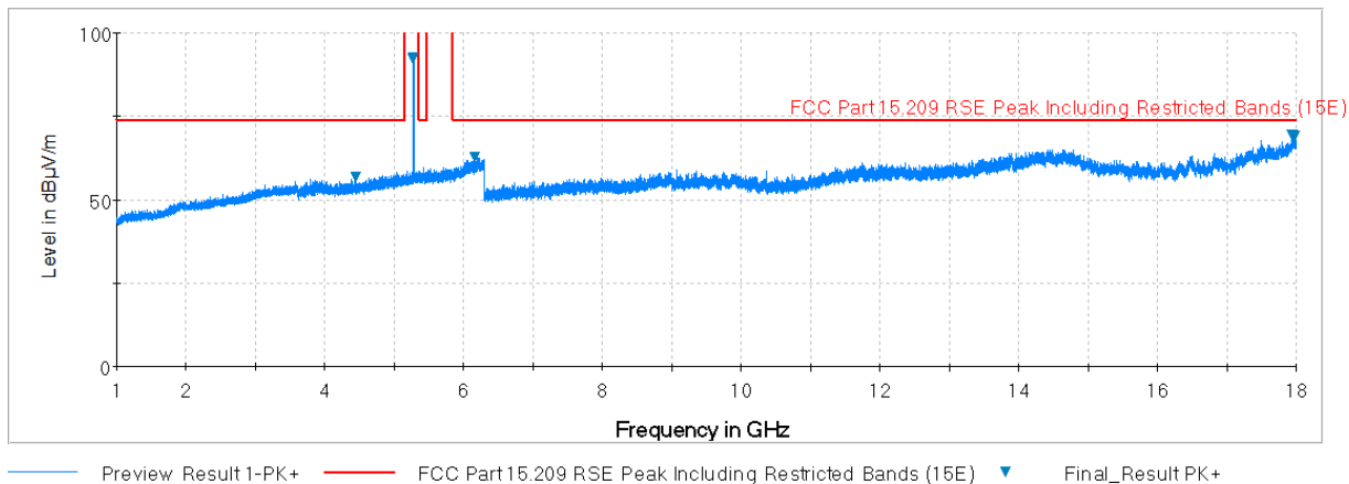
Plot 7-172. Radiated Spurious Plot above 1GHz (802.11a – U2A Ch. 56, Ant. Pol. V)
