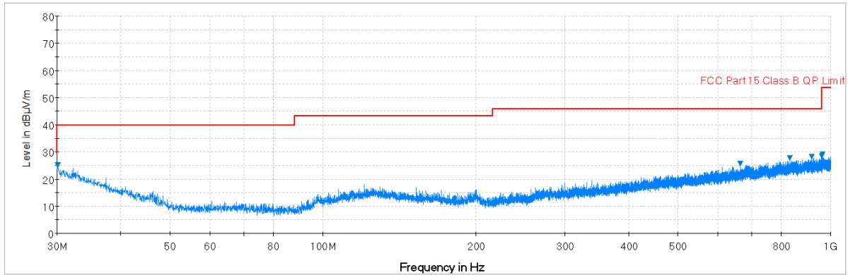
Plot 7-115. Radiated Spurious Plot below 1GHz (Pol. H)
