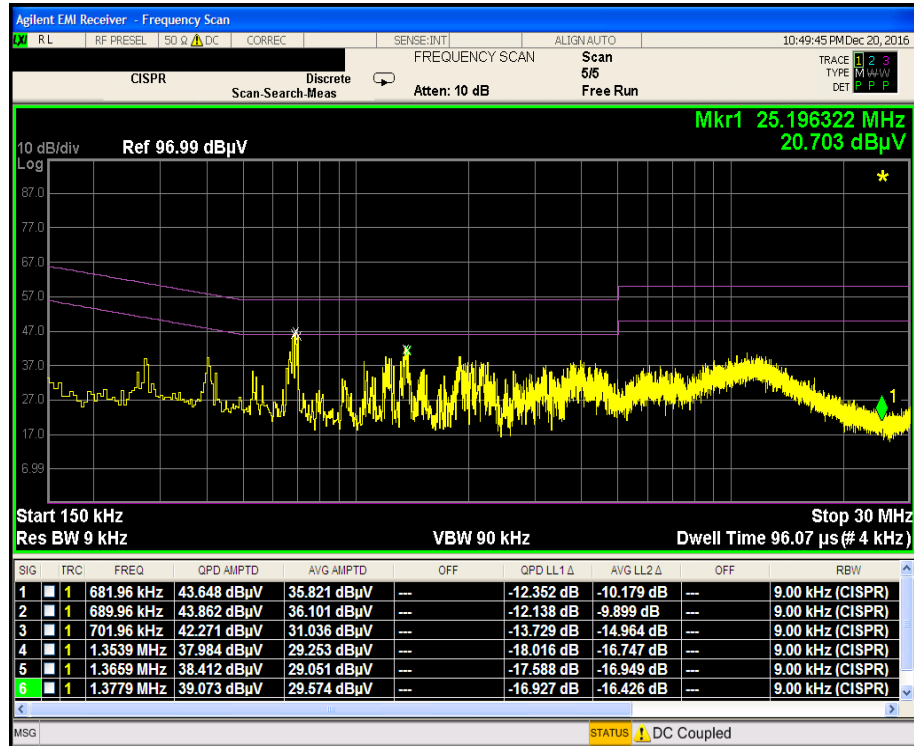
Plot 7-21. Line Conducted Plot with Bluetooth LE (N)
