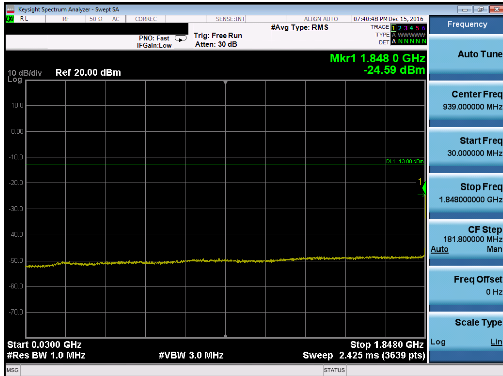
Plot 7-64. Conducted Spurious Plot (Band 2 – 3.0MHz QPSK – RB Size 1, RB Offset 0 – Low Channel)
