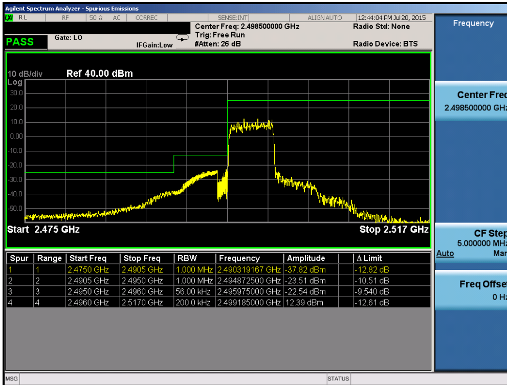
Plot 6-174. Lower ACP Plot (Band 41 – 5.0MHz QPSK – RB Size 25)
