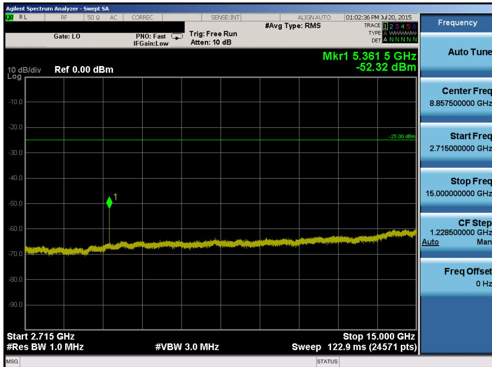
Plot 6-94. Conducted Spurious Plot (Band 41 – 10.0MHz QPSK – RB Size 1, RB Offset 0 – High Channel)
