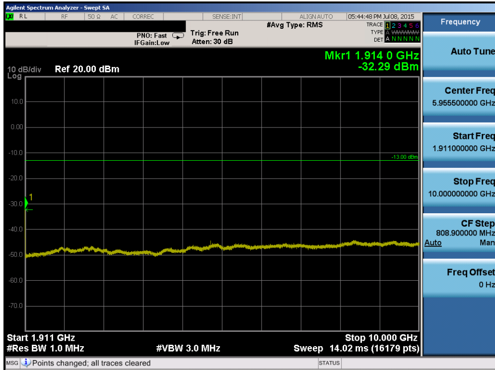
Plot 6-85. Conducted Spurious Plot (Band 2/25 – 5.0MHz QPSK – RB Size 1, RB Offset 0 – High Channel)
