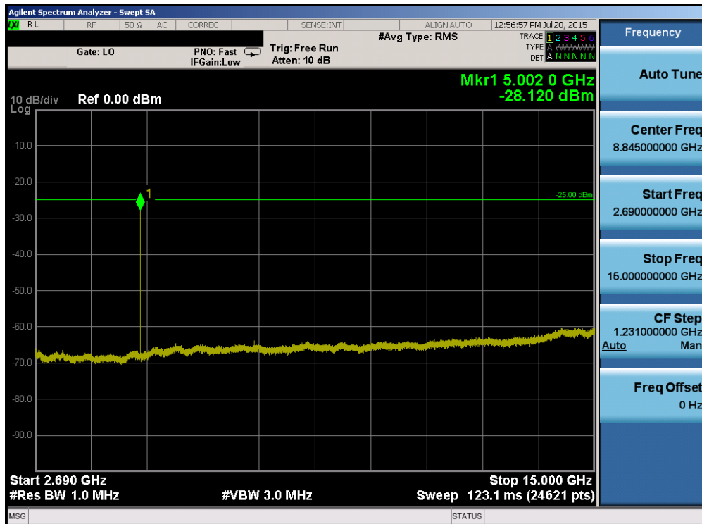
Plot 6-88. Conducted Spurious Plot (Band 41 – 10.0MHz QPSK – RB Size 1, RB Offset 0 – Low Channel)
