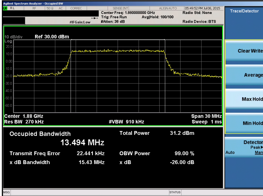
Plot 6-39. Occupied Bandwidth Plot (Band 2/25 – 15.0MHz QPSK – RB Size 75)
