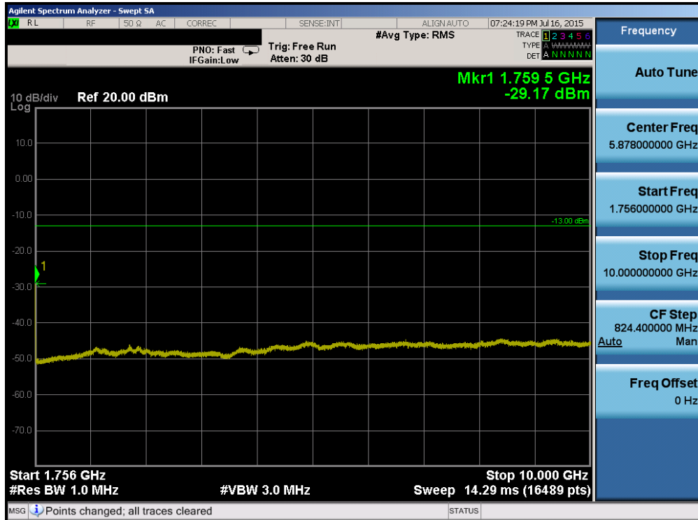
Plot 6-76. Conducted Spurious Plot (Band 4 – 5.0MHz QPSK – RB Size 1, RB Offset 0 – High Channel)
