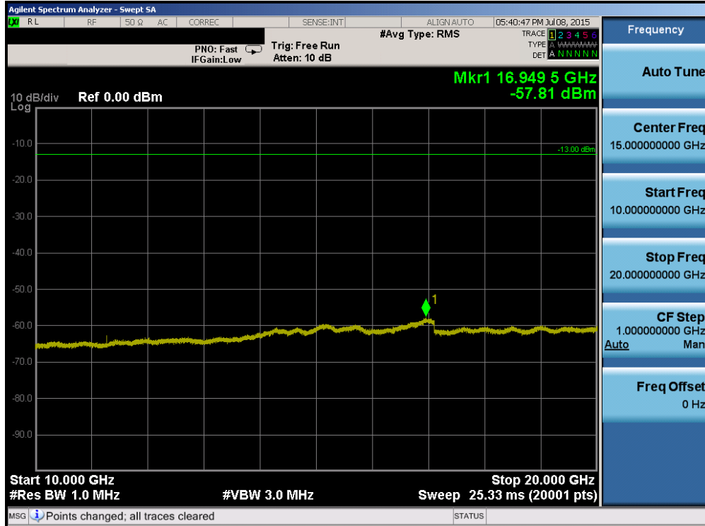
Plot 6-83. Conducted Spurious Plot (Band 2/25 – 5.0MHz QPSK – RB Size 1, RB Offset 0 – Mid Channel)
