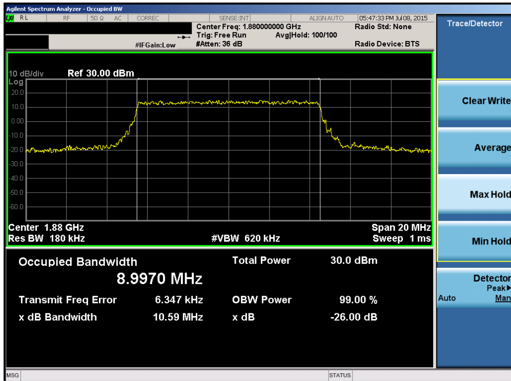
Plot 6-38. Occupied Bandwidth Plot (Band 2/25 – 10.0MHz 16-QAM – RB Size 50)
