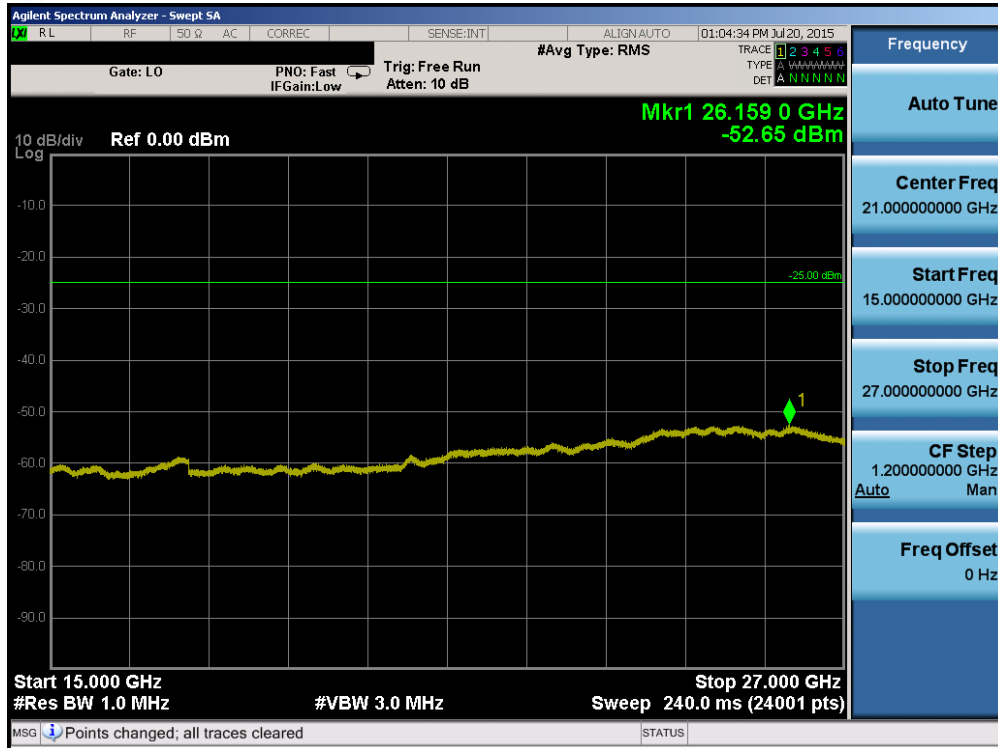
Plot 6-95. Conducted Spurious Plot (Band 41 – 10.0MHz QPSK – RB Size 1, RB Offset 0 – High Channel)
