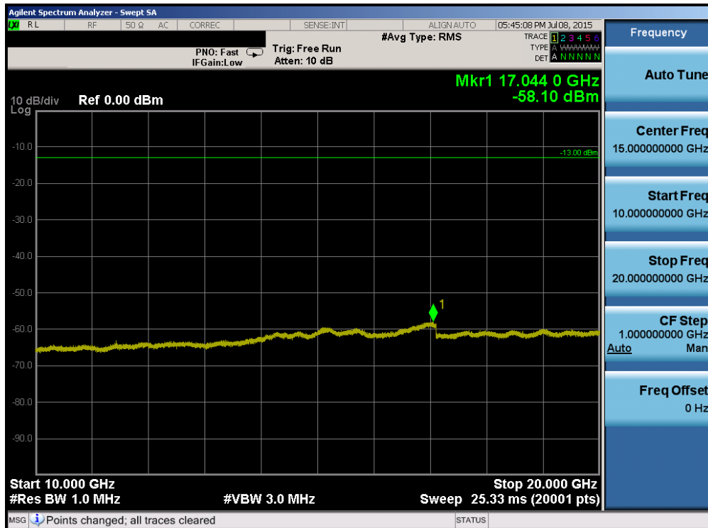
Plot 6-86. Conducted Spurious Plot (Band 2/25 – 5.0MHz QPSK – RB Size 1, RB Offset 0 – High Channel)
