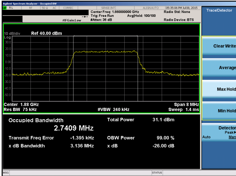
Plot 6-33. Occupied Bandwidth Plot (Band 2/25 – 3.0MHz QPSK – RB Size 15)
