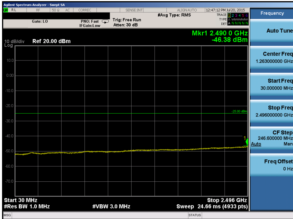
Plot 6-90. Conducted Spurious Plot (Band 41 – 10.0MHz QPSK – RB Size 1, RB Offset 0 – Mid Channel)
