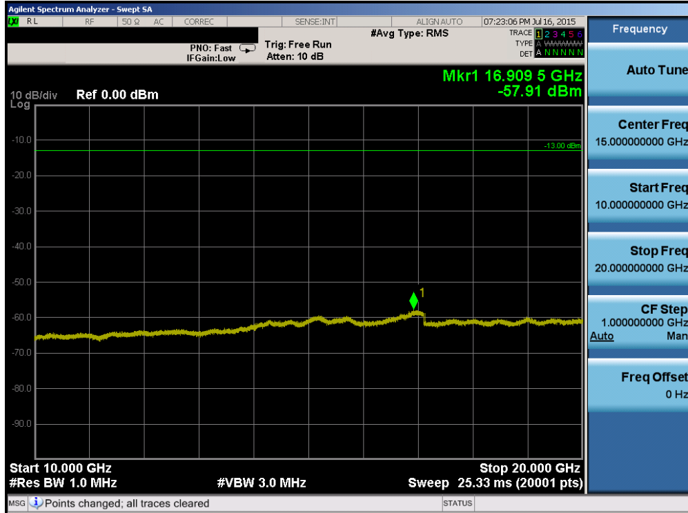
Plot 6-71. Conducted Spurious Plot (Band 4 – 5.0MHz QPSK – RB Size 1, RB Offset 0 – Low Channel)
