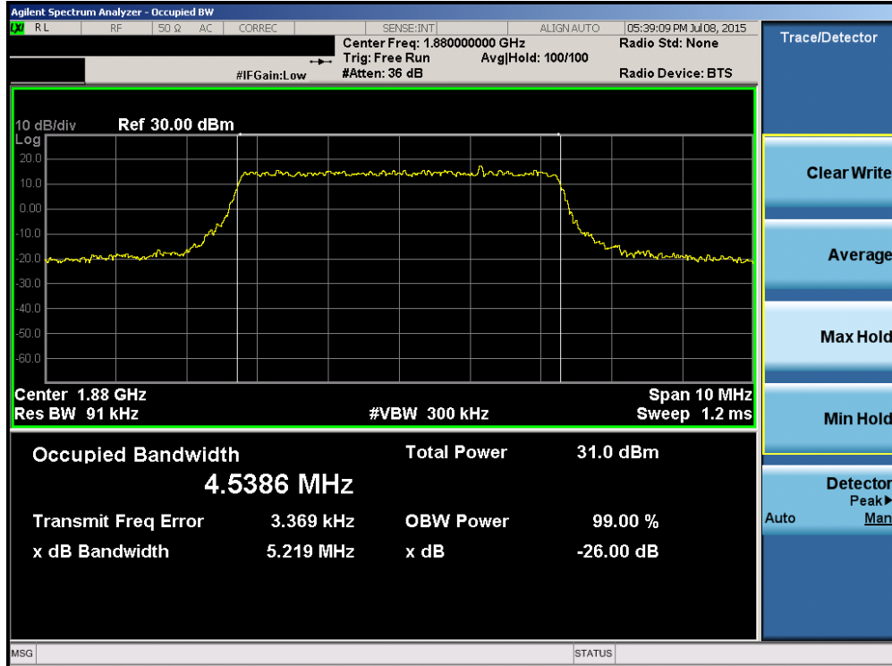
Plot 6-35. Occupied Bandwidth Plot (Band 2/25 – 5.0MHz QPSK – RB Size 25)
