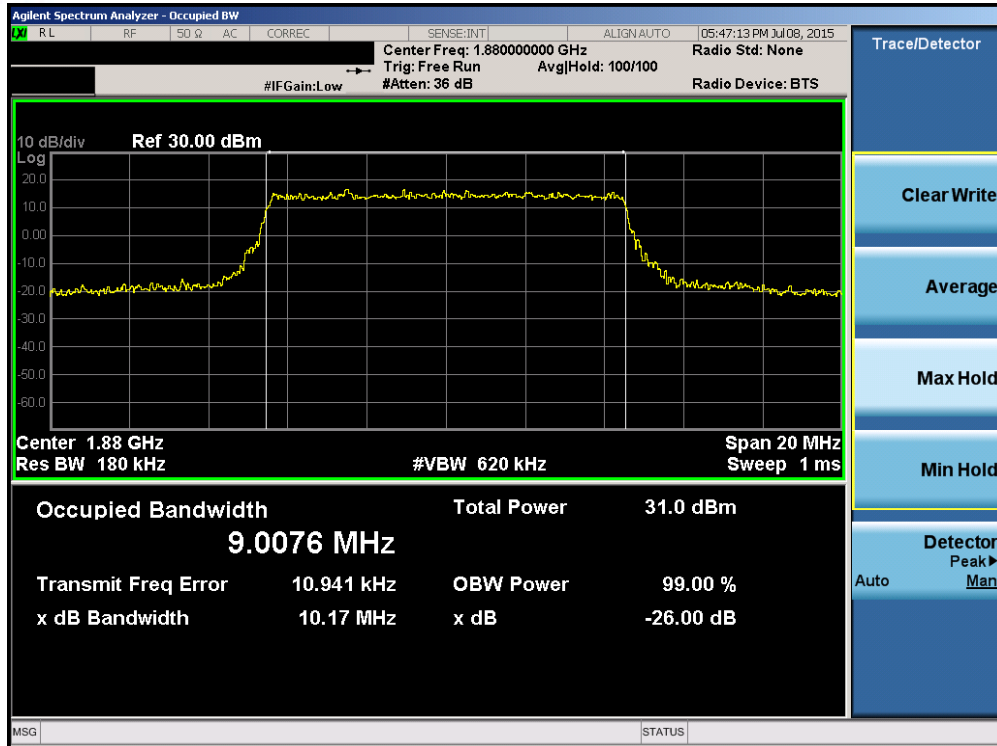
Plot 6-37. Occupied Bandwidth Plot (Band 2/25 – 10.0MHz QPSK – RB Size 50)
