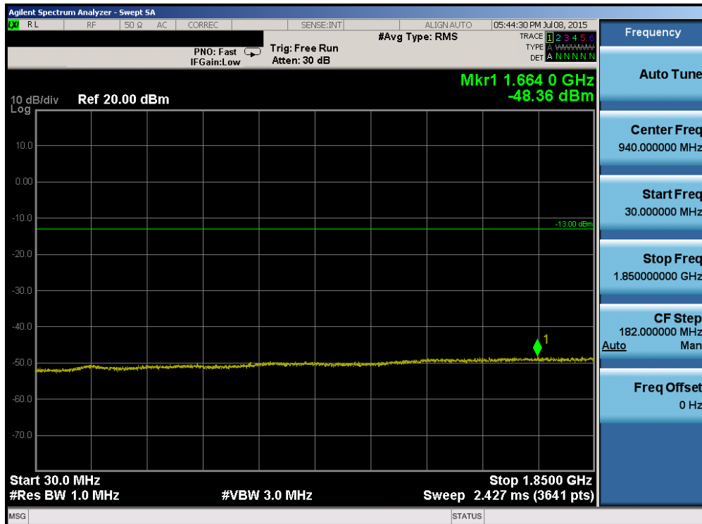
Plot 6-84. Conducted Spurious Plot (Band 2/25 – 5.0MHz QPSK – RB Size 1, RB Offset 0 – High Channel)
