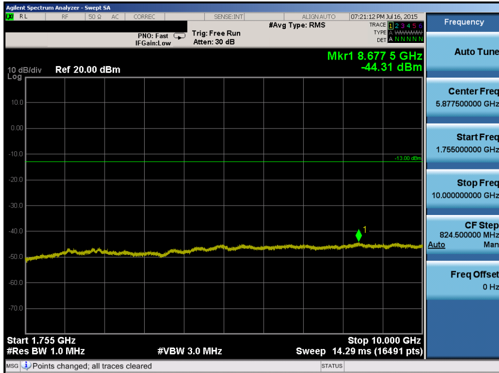
Plot 6-73. Conducted Spurious Plot (Band 4 – 5.0MHz QPSK – RB Size 1, RB Offset 0 – Mid Channel)
