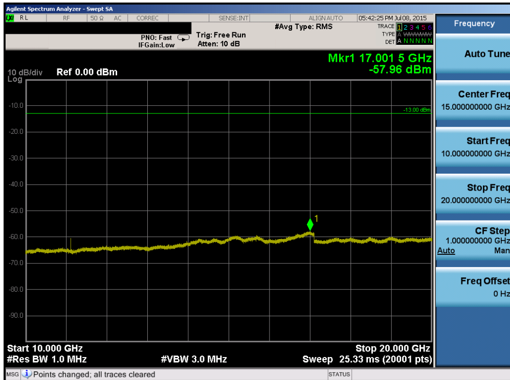
Plot 6-80. Conducted Spurious Plot (Band 2/25 – 5.0MHz QPSK – RB Size 1, RB Offset 0 – Low Channel)
