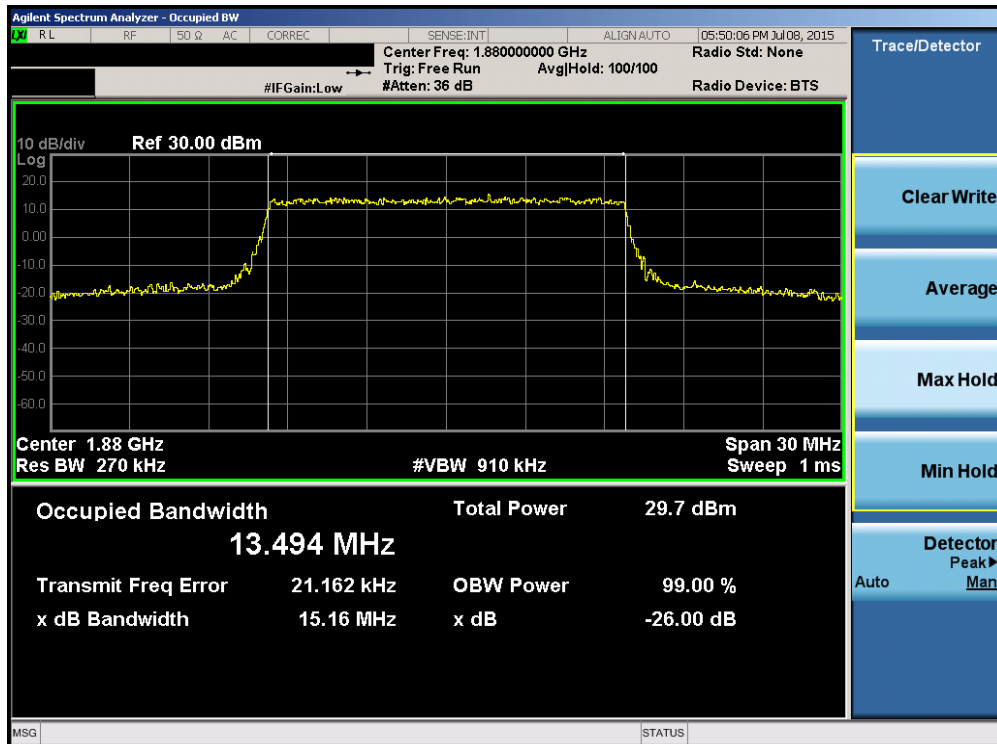
Plot 6-40. Occupied Bandwidth Plot (Band 2/25 – 15.0MHz 16-QAM – RB Size 75)
