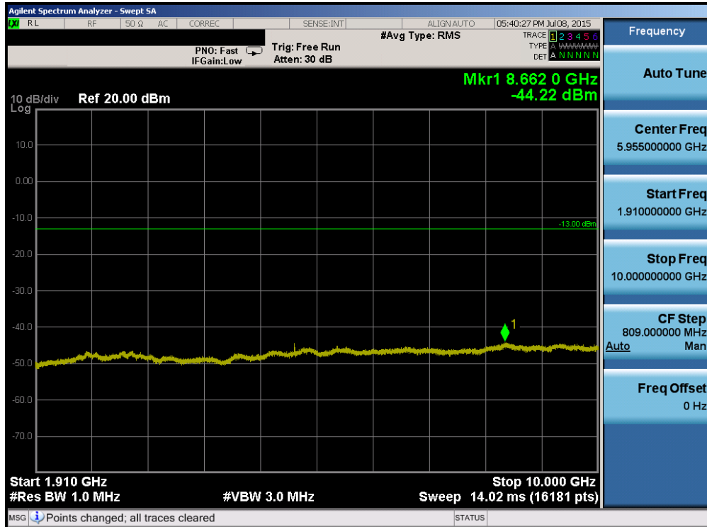
Plot 6-82. Conducted Spurious Plot (Band 2/25 – 5.0MHz QPSK – RB Size 1, RB Offset 0 – Mid Channel)
