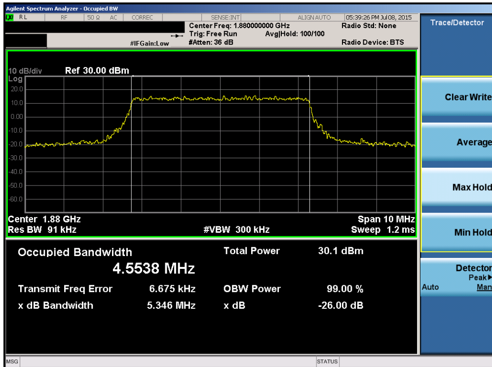
Plot 6-36. Occupied Bandwidth Plot (Band 2/25 – 5.0MHz 16-QAM – RB Size 25)
