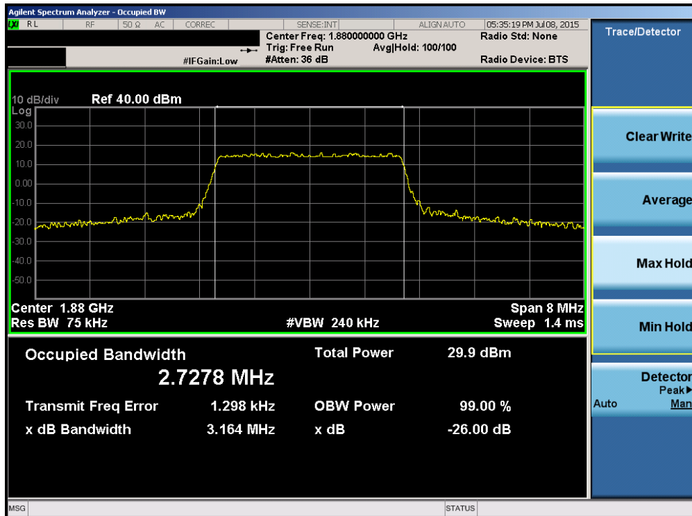
Plot 6-34. Occupied Bandwidth Plot (Band 2/25 – 3.0MHz 16-QAM – RB Size 15)
