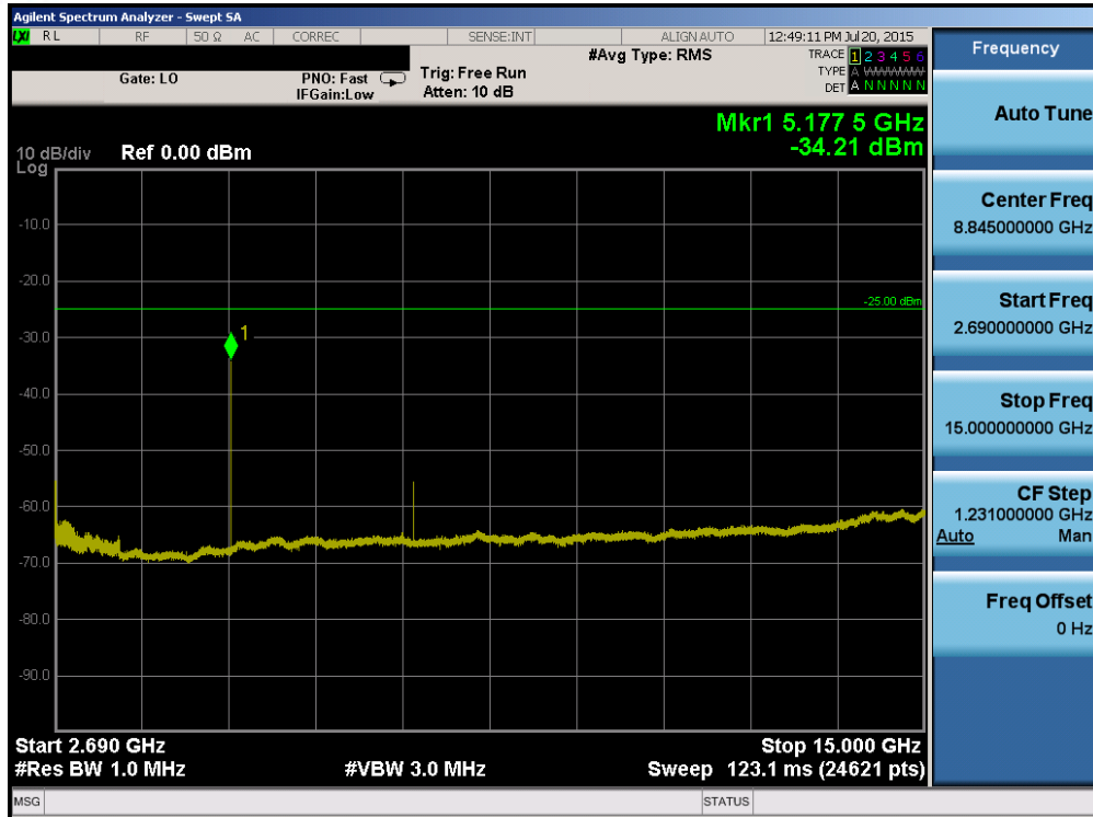
Plot 6-91. Conducted Spurious Plot (Band 41 – 10.0MHz QPSK – RB Size 1, RB Offset 0 – Mid Channel)
