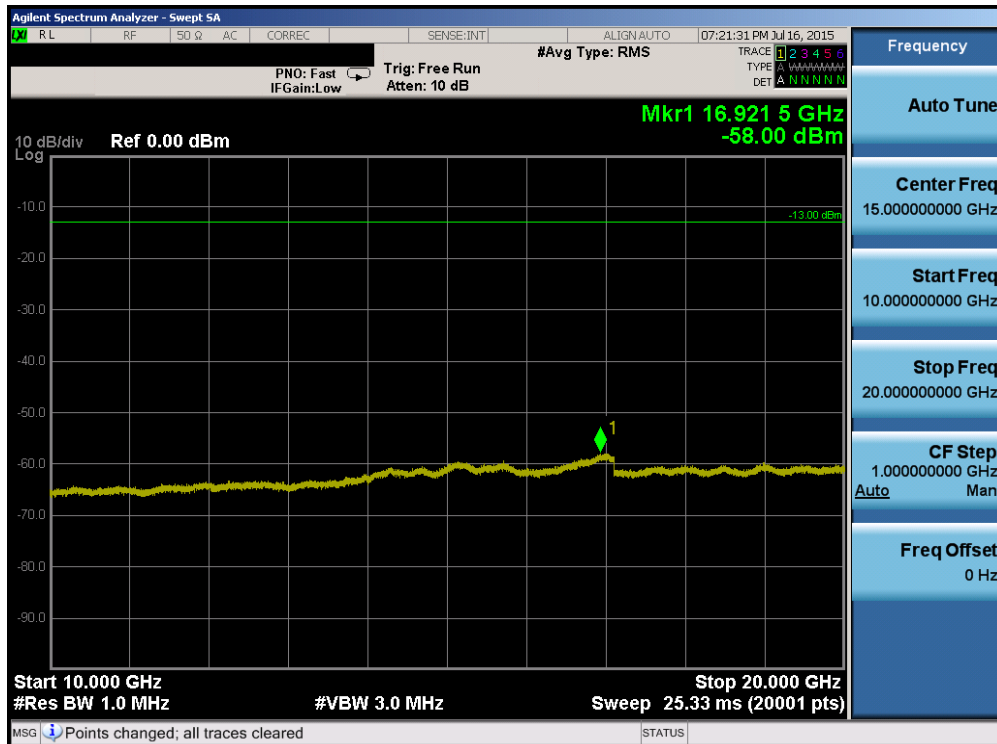
Plot 6-74. Conducted Spurious Plot (Band 4 – 5.0MHz QPSK – RB Size 1, RB Offset 0 – Mid Channel)
