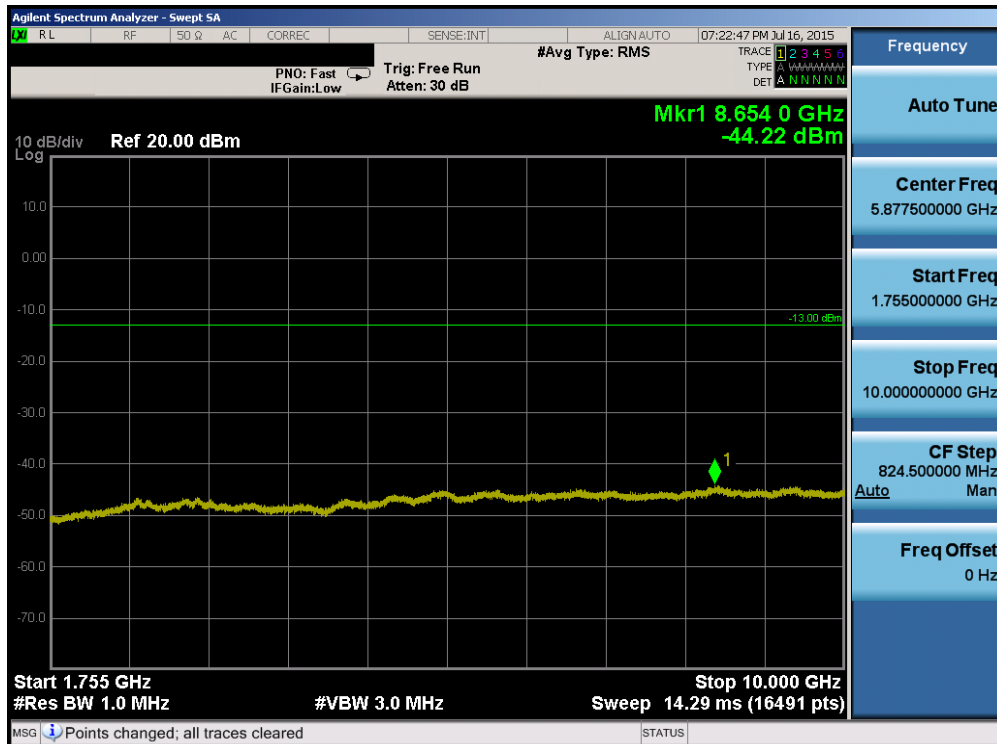
Plot 6-70. Conducted Spurious Plot (Band 4 – 5.0MHz QPSK – RB Size 1, RB Offset 0 – Low Channel)
