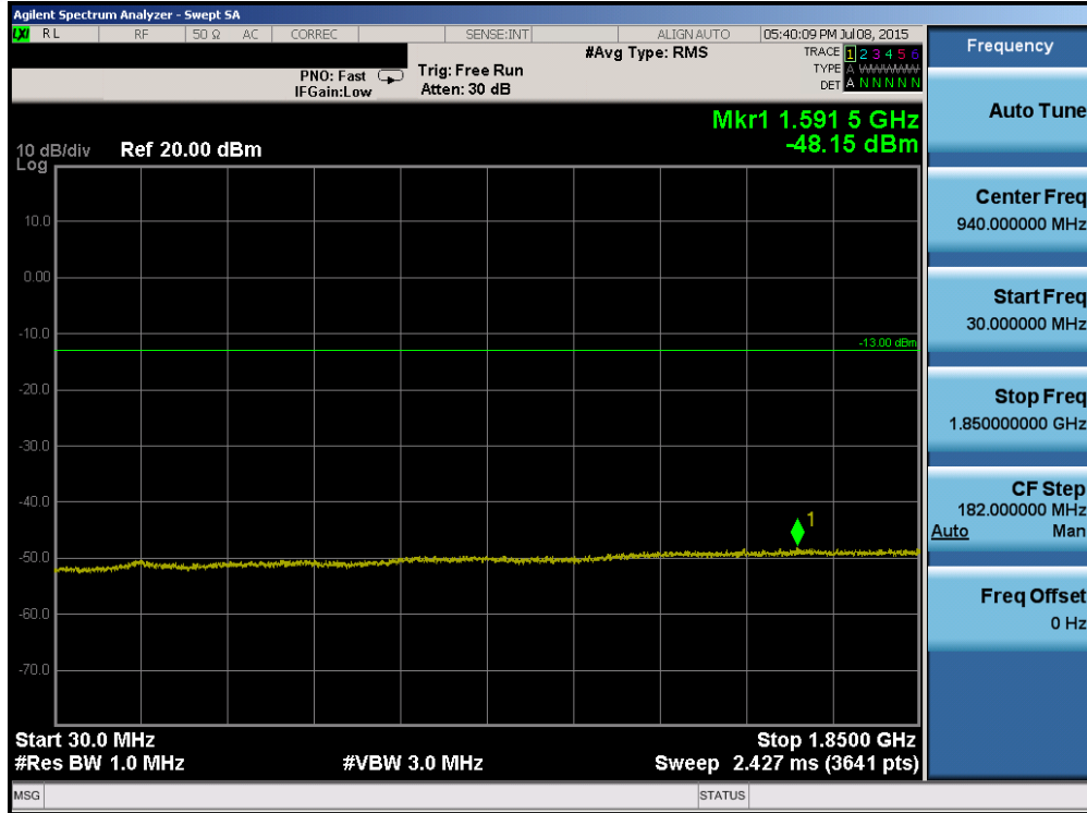
Plot 6-81. Conducted Spurious Plot (Band 2/25 – 5.0MHz QPSK – RB Size 1, RB Offset 0 – Mid Channel)
