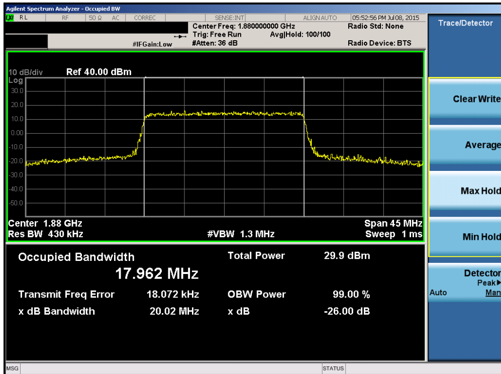
Plot 6-42. Occupied Bandwidth Plot (Band 2/25 – 20.0MHz 16-QAM – RB Size 100)
