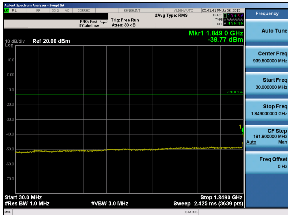
Plot 6-78. Conducted Spurious Plot (Band 2/25 – 5.0MHz QPSK – RB Size 1, RB Offset 0 – Low Channel)
