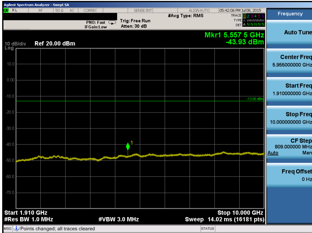
Plot 6-79. Conducted Spurious Plot (Band 2/25 – 5.0MHz QPSK – RB Size 1, RB Offset 0 – Low Channel)
