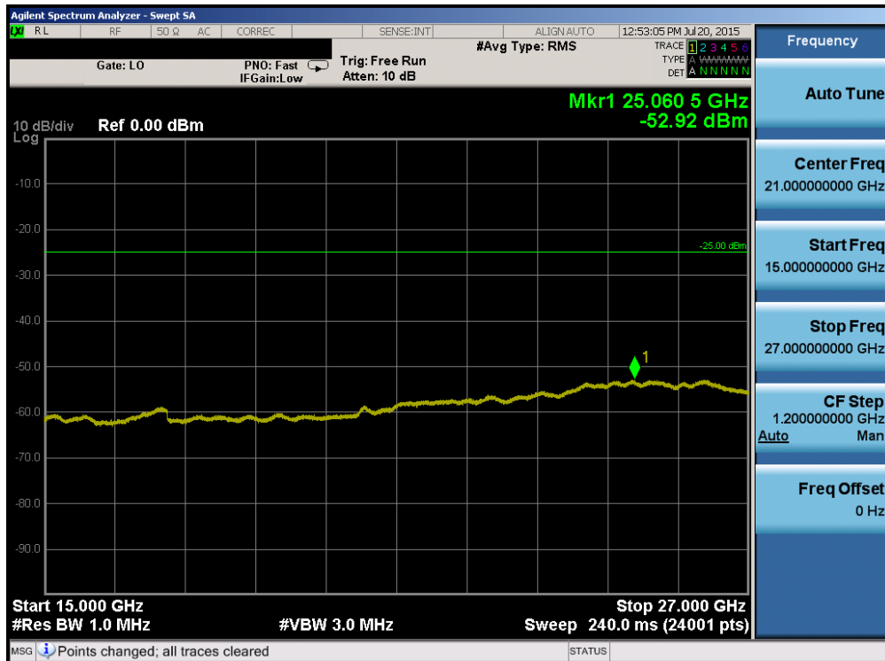
Plot 6-92. Conducted Spurious Plot (Band 41 – 10.0MHz QPSK – RB Size 1, RB Offset 0 – Mid Channel)
