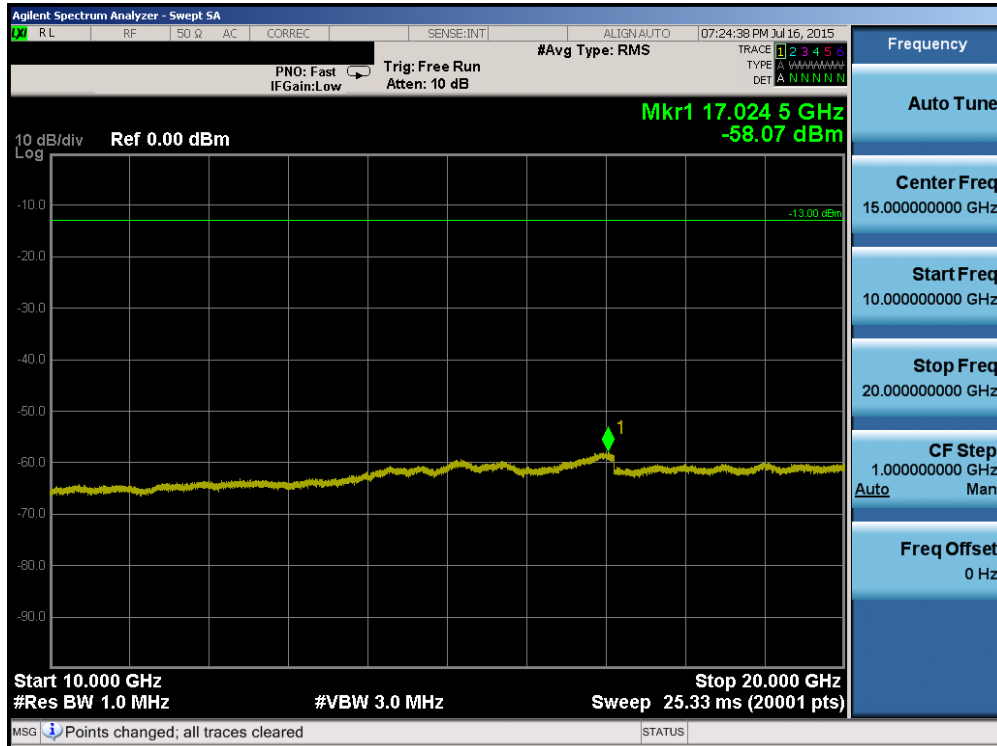
Plot 6-77. Conducted Spurious Plot (Band 4 – 5.0MHz QPSK – RB Size 1, RB Offset 0 – High Channel)
