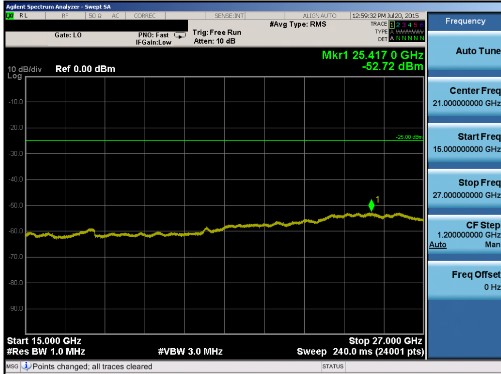
Plot 6-89. Conducted Spurious Plot (Band 41 – 10.0MHz QPSK – RB Size 1, RB Offset 0 – Low Channel)
