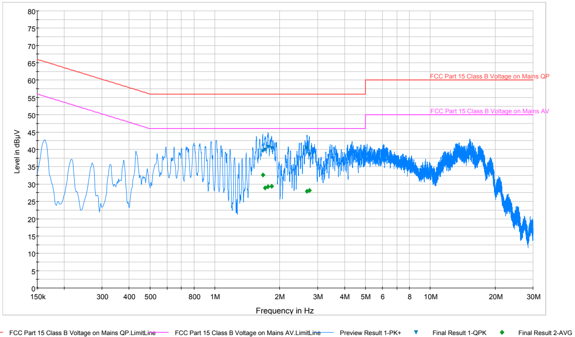
Plot 6-7. Line-Conducted Test Plot (N)
