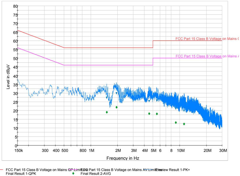
Plot 6-139. Line Conducted Plot with 802.11a (L1)
