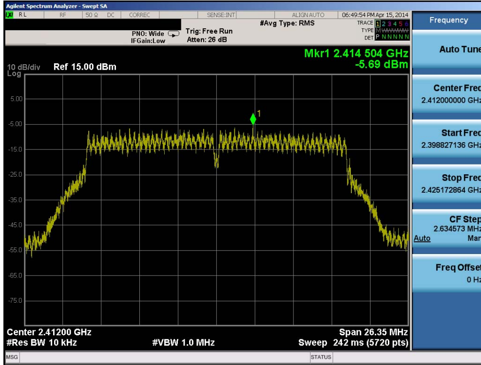
Plot 6-43. Power Spectral Density Plot (802.11n (2.4GHz) – Ch. 1)
