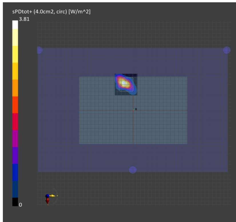
Figure C-3 4cm 2 -averaged power density distribution measured at input.power.limit of 5.2dBm on the Rear Surface n260 beam ID 26.
