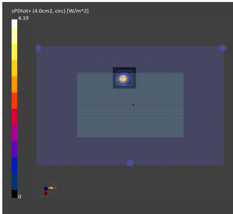
Figure C-2 4cm 2 -averaged power density distribution measured at input.power.limit of 2.3dBm on the Rear Surface n261 beam ID 146.
