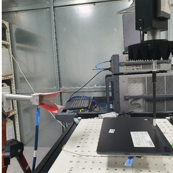
A.10 : Radiated power measurement setup
