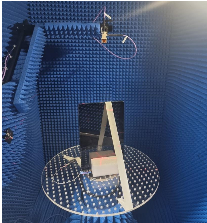
A.10 : Radiated power measurement setup
