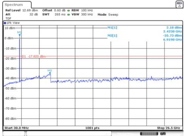
Conducted spurious / 2 417 MHz
