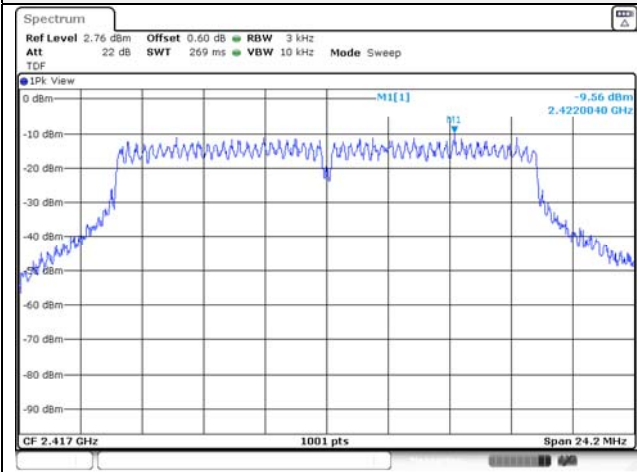
802.11g / 2 417 MHz
