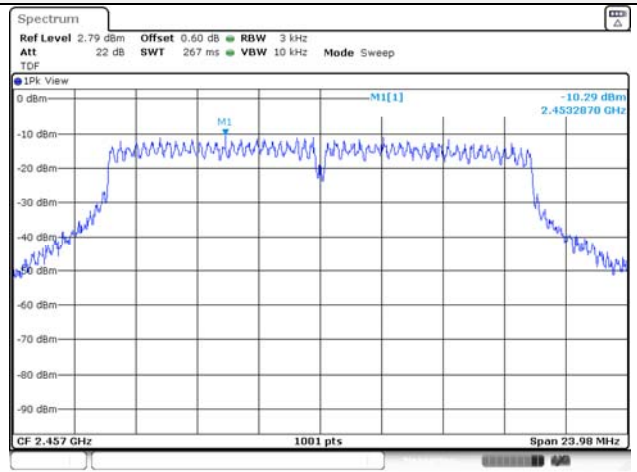
802.11g / 2 457 MHz
