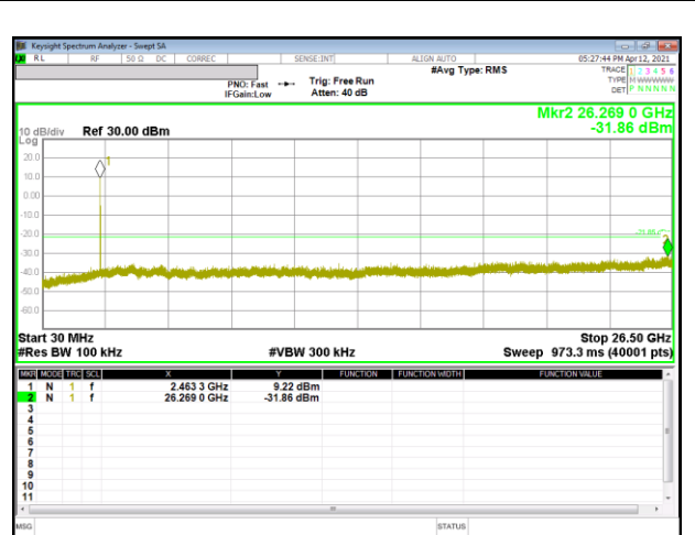
Out-Of-Band 11 Channel
