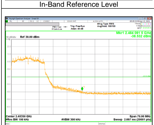
10 Channel Band-edge
