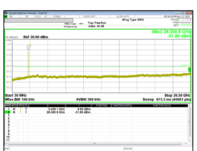
Out-Of-Band 6 Channel
