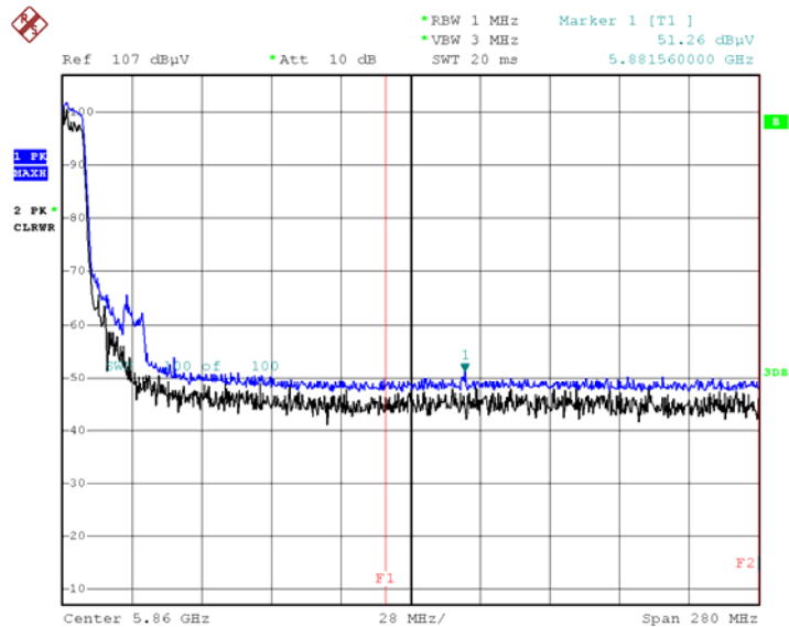
Peak Reading (802.11n_HT20, Ch.144, Y-H)
