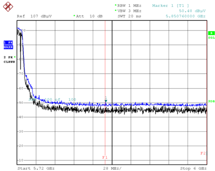
Peak Reading (802.11a, Ch.144, Y-H)
