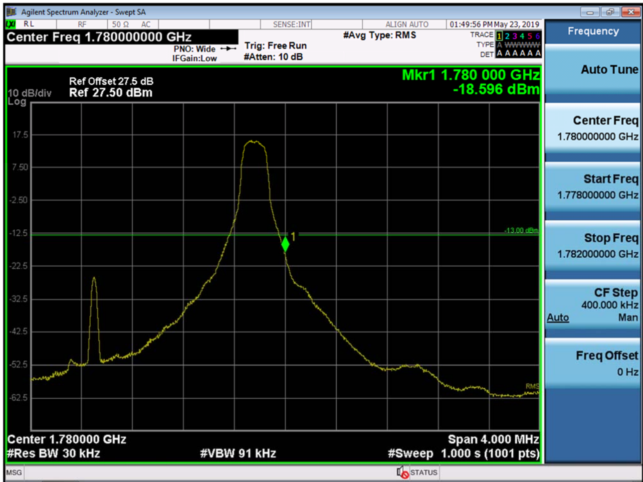
BAND 66/4. Upper Band Edge Plot (3M BW Ch.132657 QPSK_RB1_Offset 14) -1
