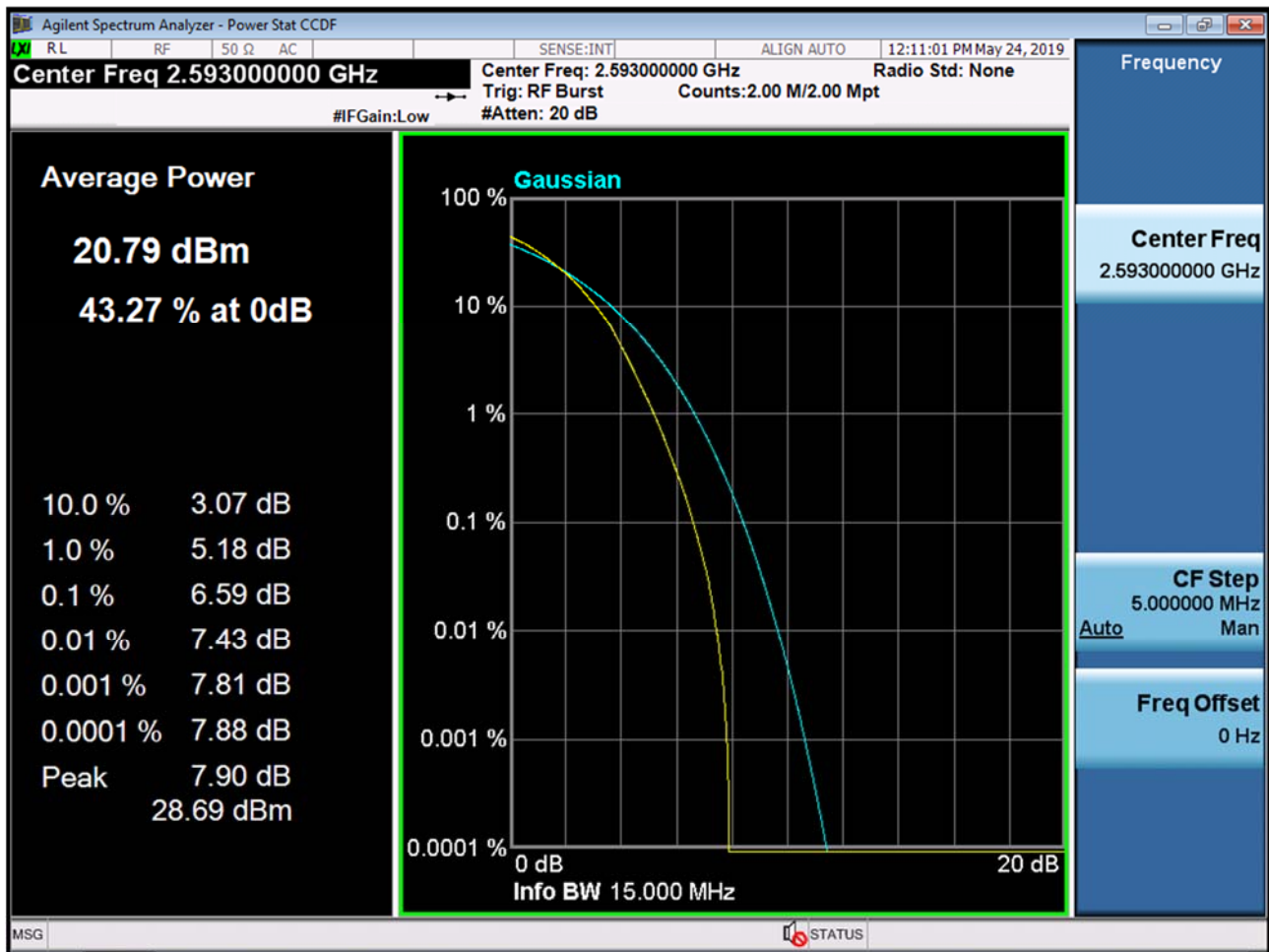
BAND 41. PAR Plot (15M BW_Ch.40620_64QAM_RB75_0)
