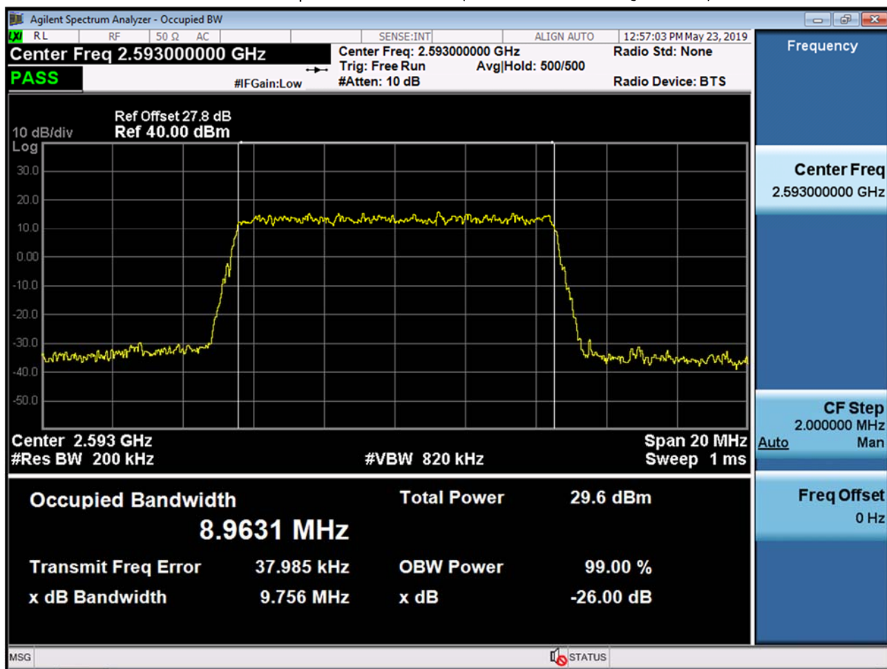
BAND 41. Occupied Bandwidth Plot (10 MHz Ch.40620 16-QAM RB 50)
