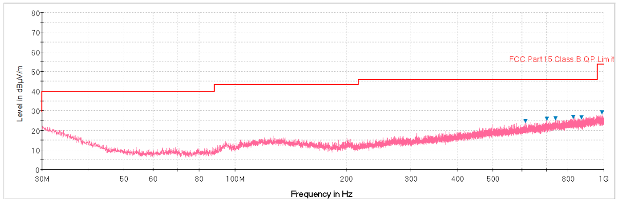
Plot 7-107. Radiated Spurious Plot below 1GHz (Pol. H)
