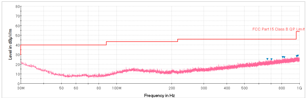
Plot 7-109. Radiated Spurious Plot below 1GHz (Pol. H)
