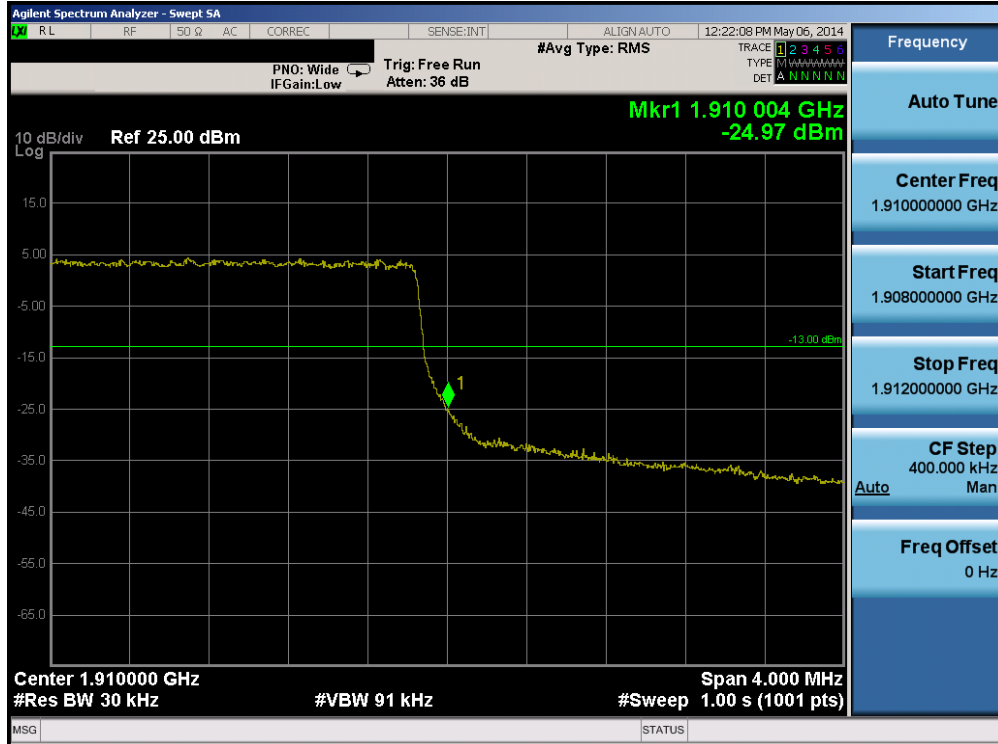
Plot 6-199. Upper Band Edge Plot (Band 2 – 3.0MHz QPSK – RB Size 15)
