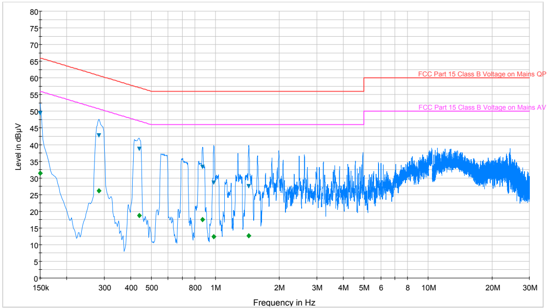
Plot 6-137. Line Conducted Plot with 802.11b (L1)
