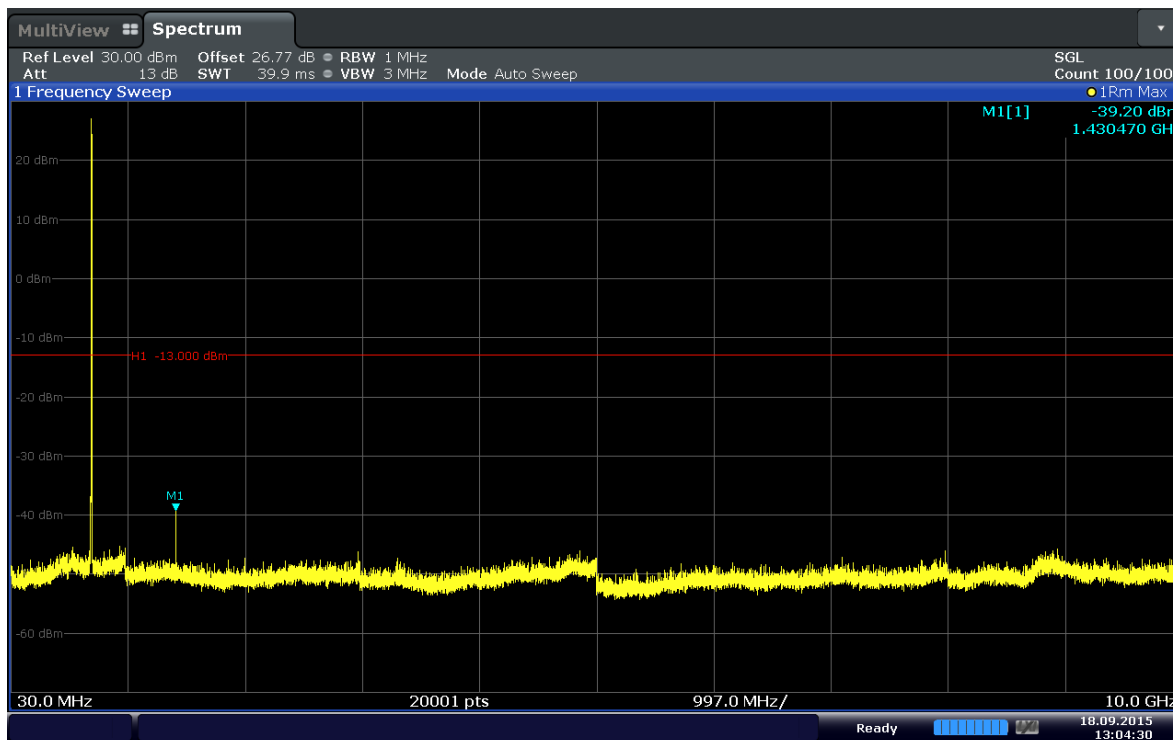
Plot 6-23. Conducted Spurious Plot (Band 12-1.4MHz-QPSK-RB Size 1-RB Offset 2-Ch.23173)
