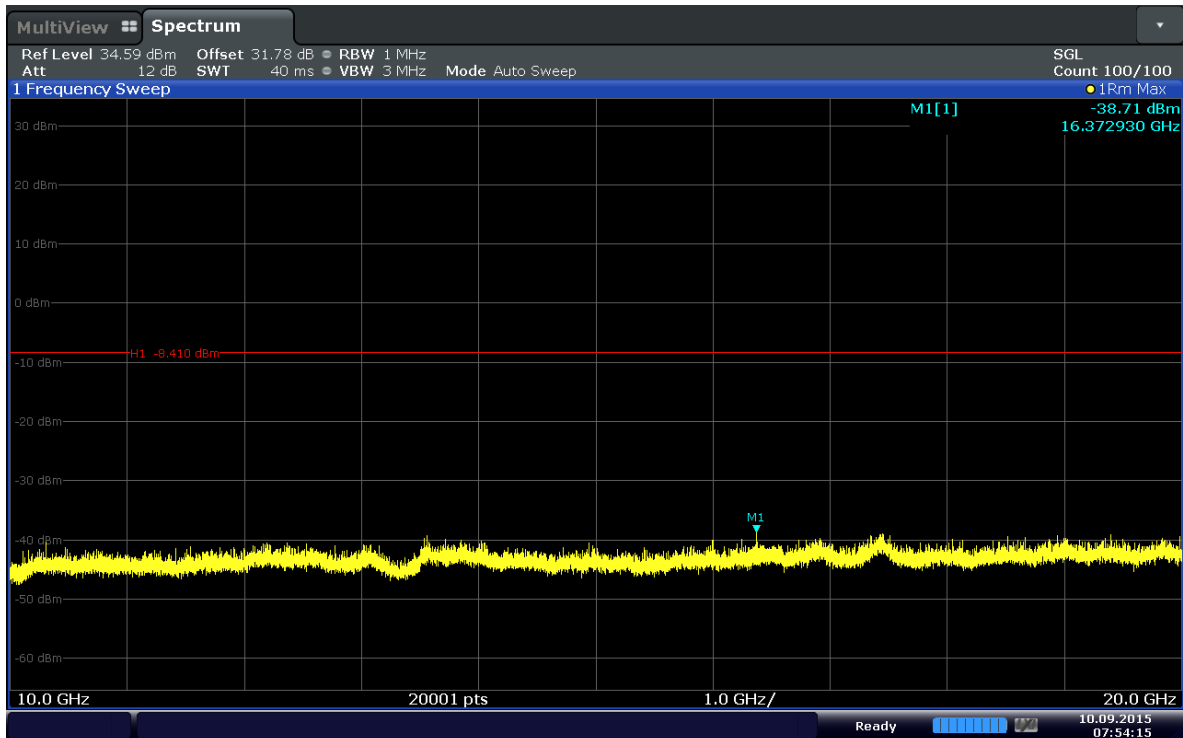
Plot 6-38. Conducted Spurious Plot (Band 4-1.4MHz-QPSK-RB Size 1-RB Offset 5-Ch.20393)
