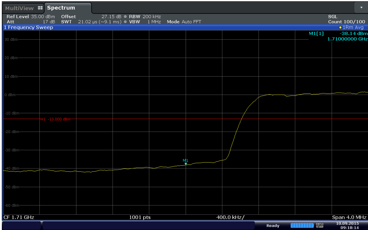
Plot 6-95. Lower Band Edge Plot (Band 4 – 15MHz – QPSK – RB Size 75)
