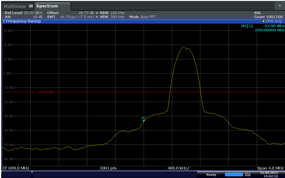
Plot 6-77. Lower Band Edge Plot (Band 12 – 10MHz – QPSK – RB Size 1 – RB Offset 0)
