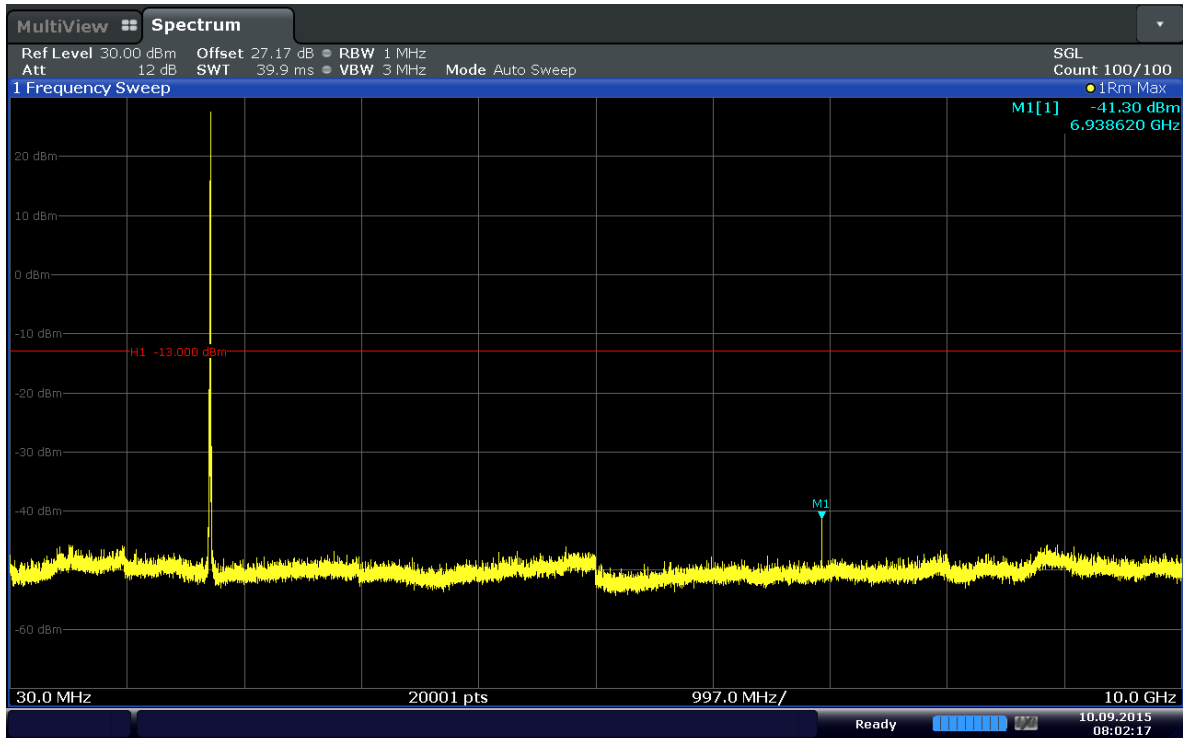
Plot 6-47. Conducted Spurious Plot (Band 4–5MHz–QPSK–RB Size 1–RB Offset 24–Ch.20175)
