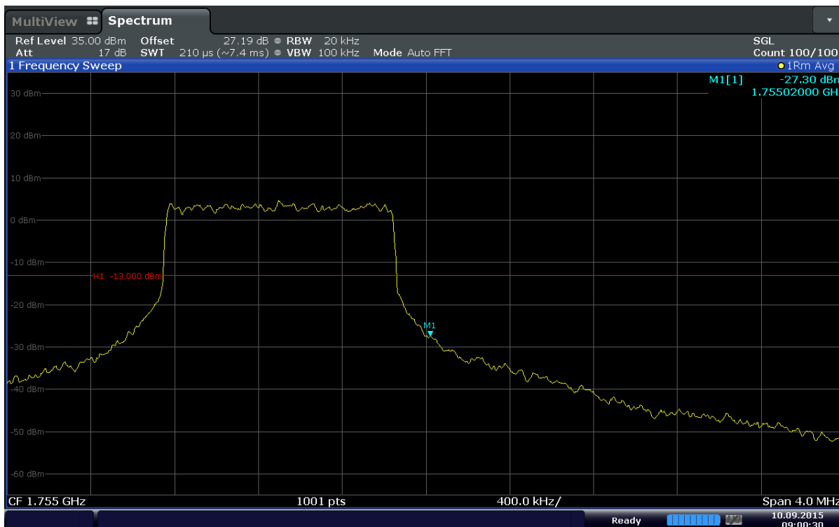
Plot 6-81. Upper Band Edge Plot (Band 4 – 1.4MHz – QPSK – RB Size 6)
