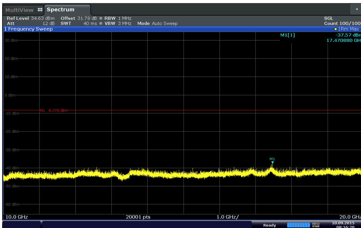
Plot 6-64. Conducted Spurious Plot (Band 4–20MHz–QPSK–RB Size 1–RB Offset 50–Ch.20050)
