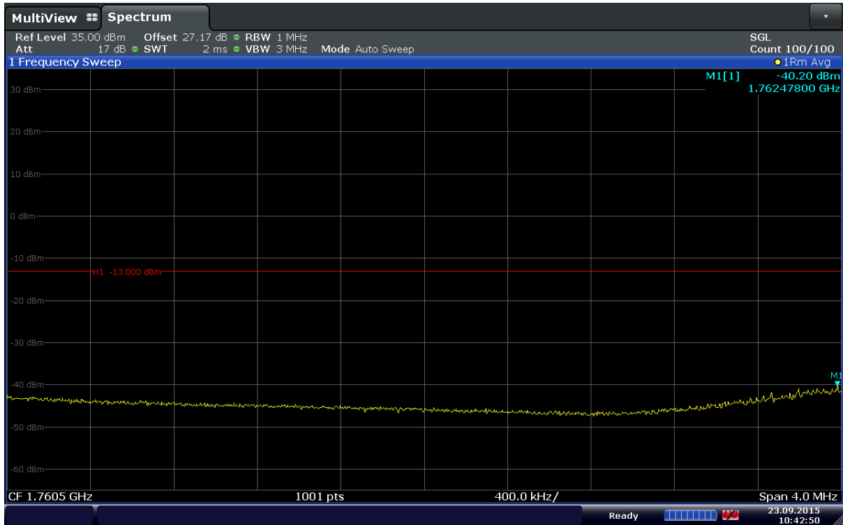
Plot 6-106. Extended Upper Band Edge Plot (Band 4 – 20MHz – QPSK – RB Size 1 – RB Offset 49)
