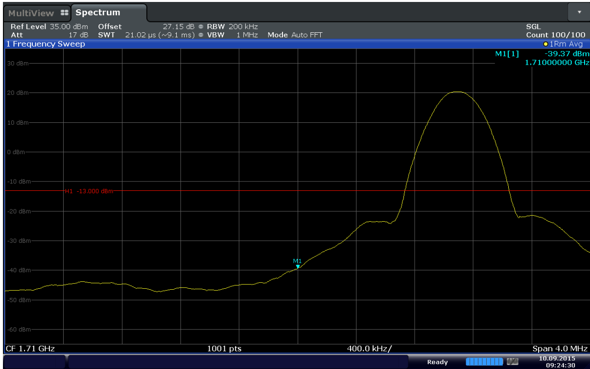
Plot 6-101. Lower Band Edge Plot (Band 4 – 20MHz – QPSK – RB Size 1 – RB Offset 0)
