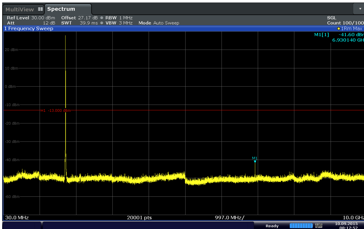
Plot 6-65. Conducted Spurious Plot (Band 4–20MHz–QPSK–RB Size 1–RB Offset 50–Ch.20175)
