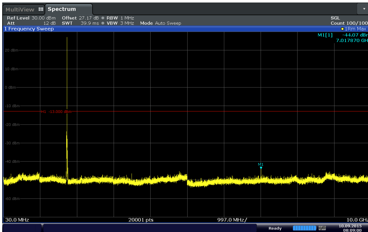
Plot 6-55. Conducted Spurious Plot (Band 4-10MHz-QPSK-RB Size 1-RB Offset 49-Ch.20350)
