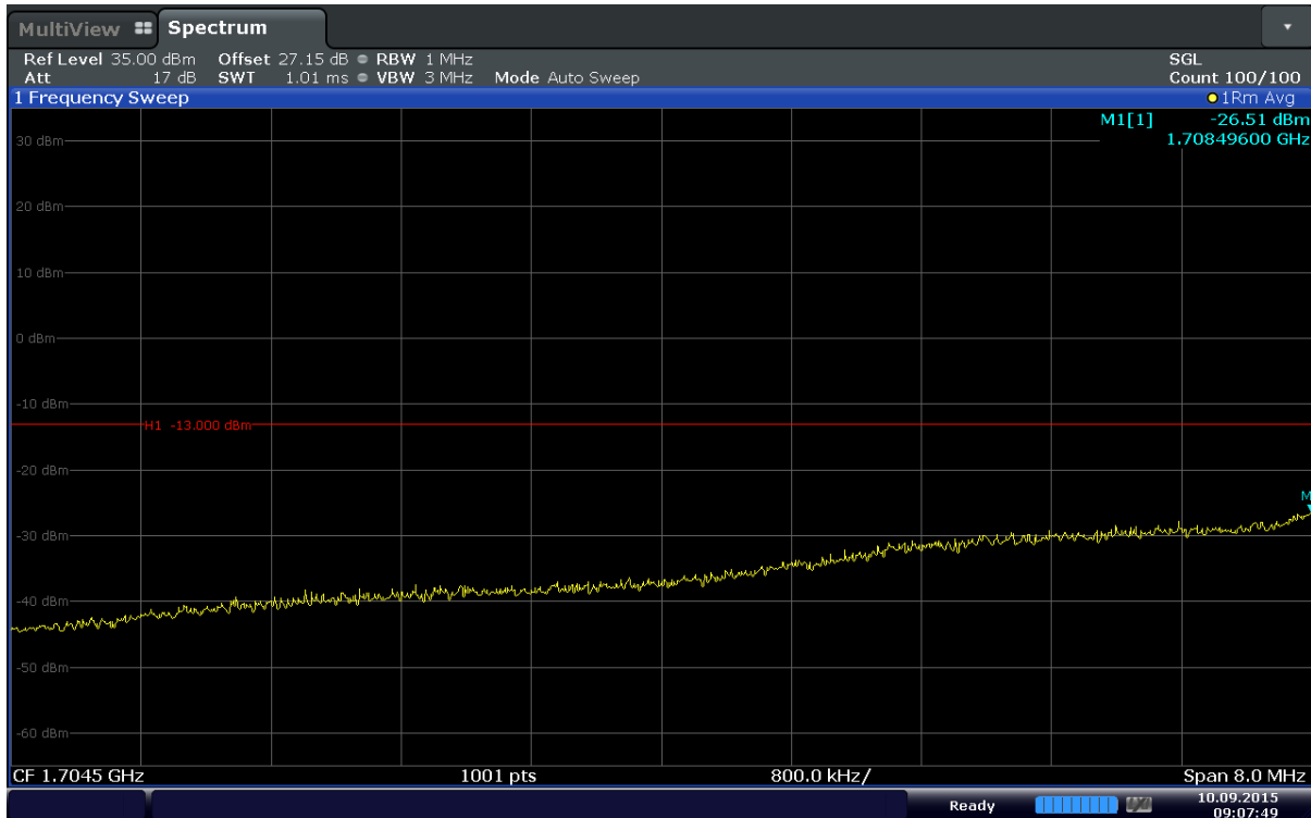
Plot 6-88. Extended Lower Band Edge Plot (Band 4 – 5MHz – QPSK – RB Size 25)
