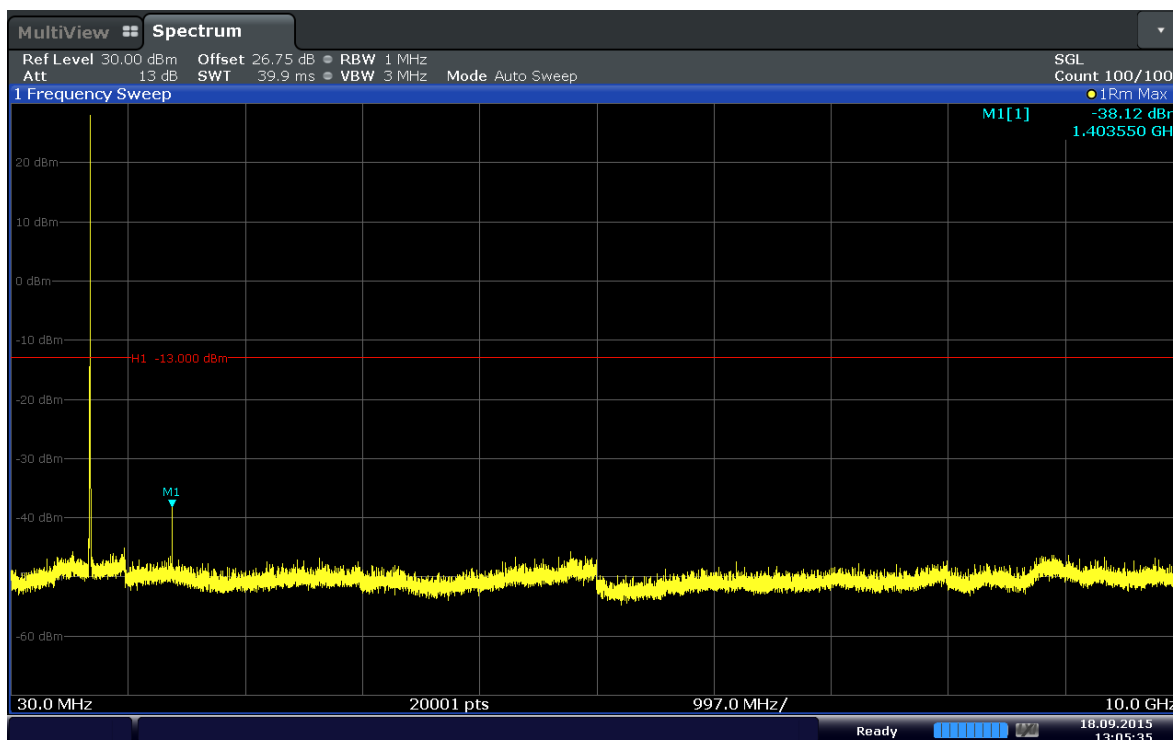
Plot 6-24. Conducted Spurious Plot (Band 12-3MHz-QPSK-RB Size 1-RB Offset 14-Ch.23025)
