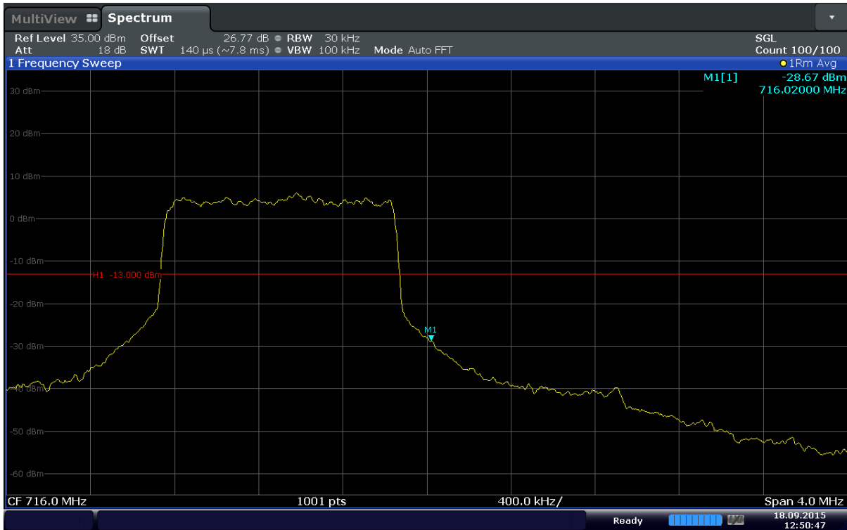
Plot 6-70. Upper Band Edge Plot (Band 12 – 1.4MHz – QPSK – RB Size 6)
