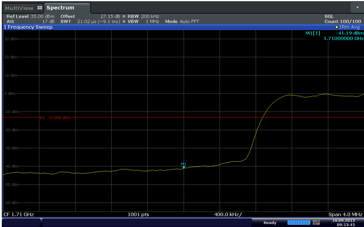
Plot 6-99. Lower Band Edge Plot (Band 4 – 20MHz – QPSK – RB Size 100)
