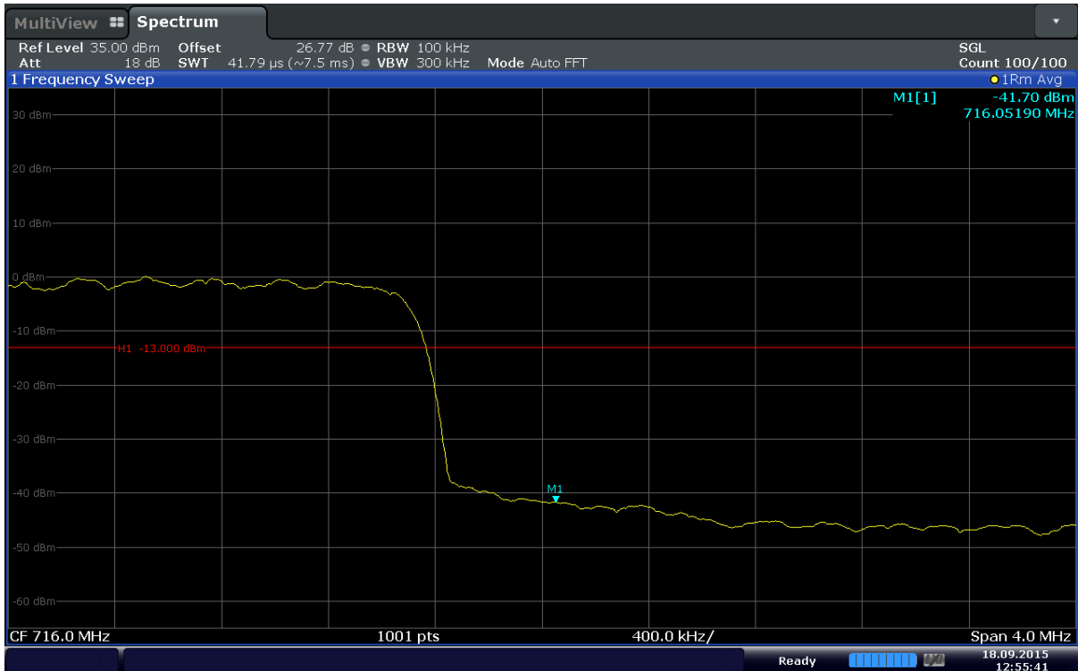
Plot 6-76. Upper Band Edge Plot (Band 12 – 10MHz – QPSK – RB Size 50)
