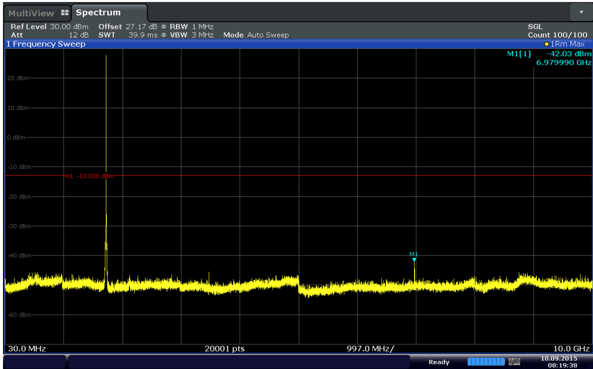
Plot 6-67. Conducted Spurious Plot (Band 4–20MHz–QPSK–RB Size 1–RB Offset 50–Ch.20300)
