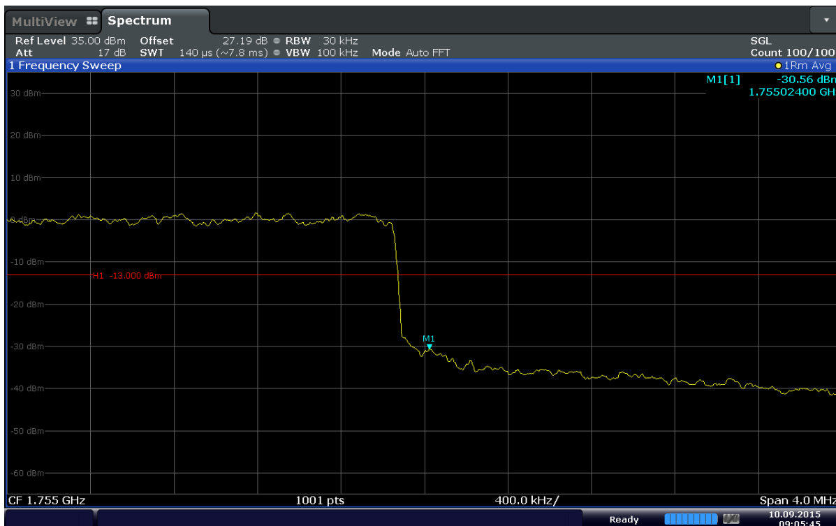
Plot 6-85. Upper Band Edge Plot (Band 4 – 3MHz – QPSK – RB Size 15)
