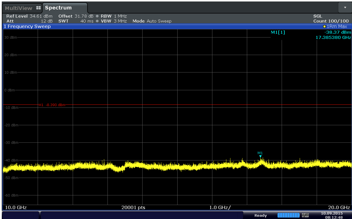
Plot 6-60. Conducted Spurious Plot (Band 4–15MHz–QPSK–RB Size 1–RB Offset 0–Ch.20175)
