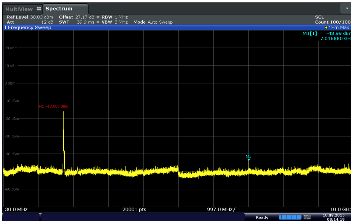
Plot 6-61. Conducted Spurious Plot (Band 4-15MHz-QPSK-RB Size 1-RB Offset 74-Ch.20325)
