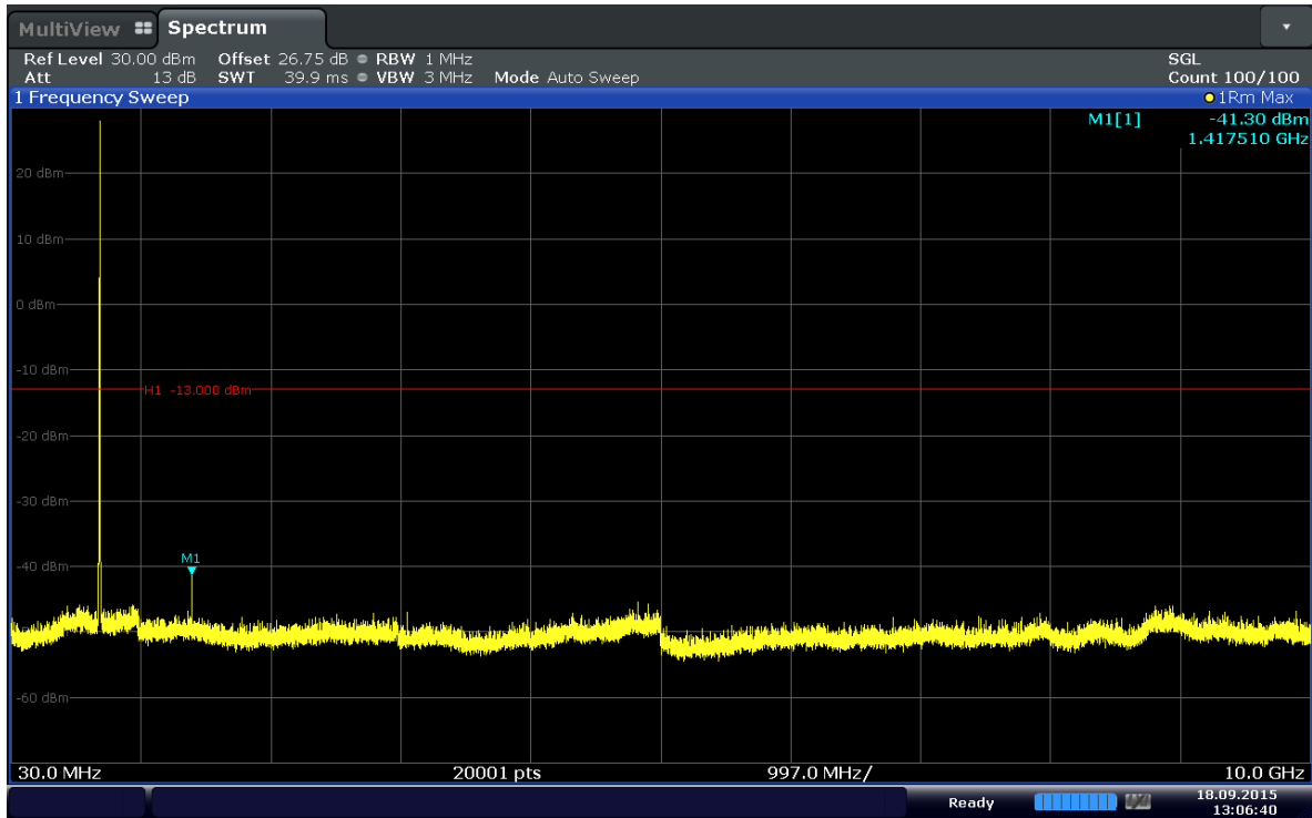
Plot 6-25. Conducted Spurious Plot (Band 12-3MHz-QPSK-RB Size 1-RB Offset 14-Ch.23095)
