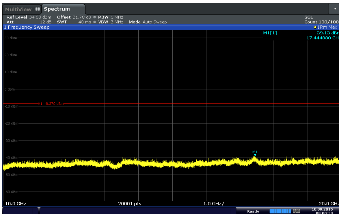
Plot 6-46. Conducted Spurious Plot (Band 4–5MHz–QPSK–RB Size 1–RB Offset 24–Ch.19975)
