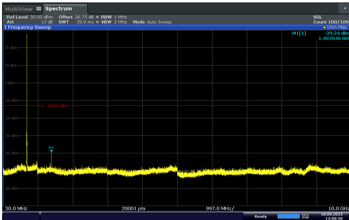
Plot 6-27. Conducted Spurious Plot (Band 12-5MHz-QPSK-RB Size 1-RB Offset 24-Ch.23035)
