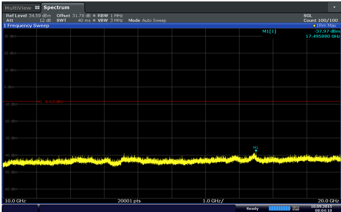
Plot 6-50. Conducted Spurious Plot (Band 4–5MHz–QPSK–RB Size 1–RB Offset 24–Ch.20375)
