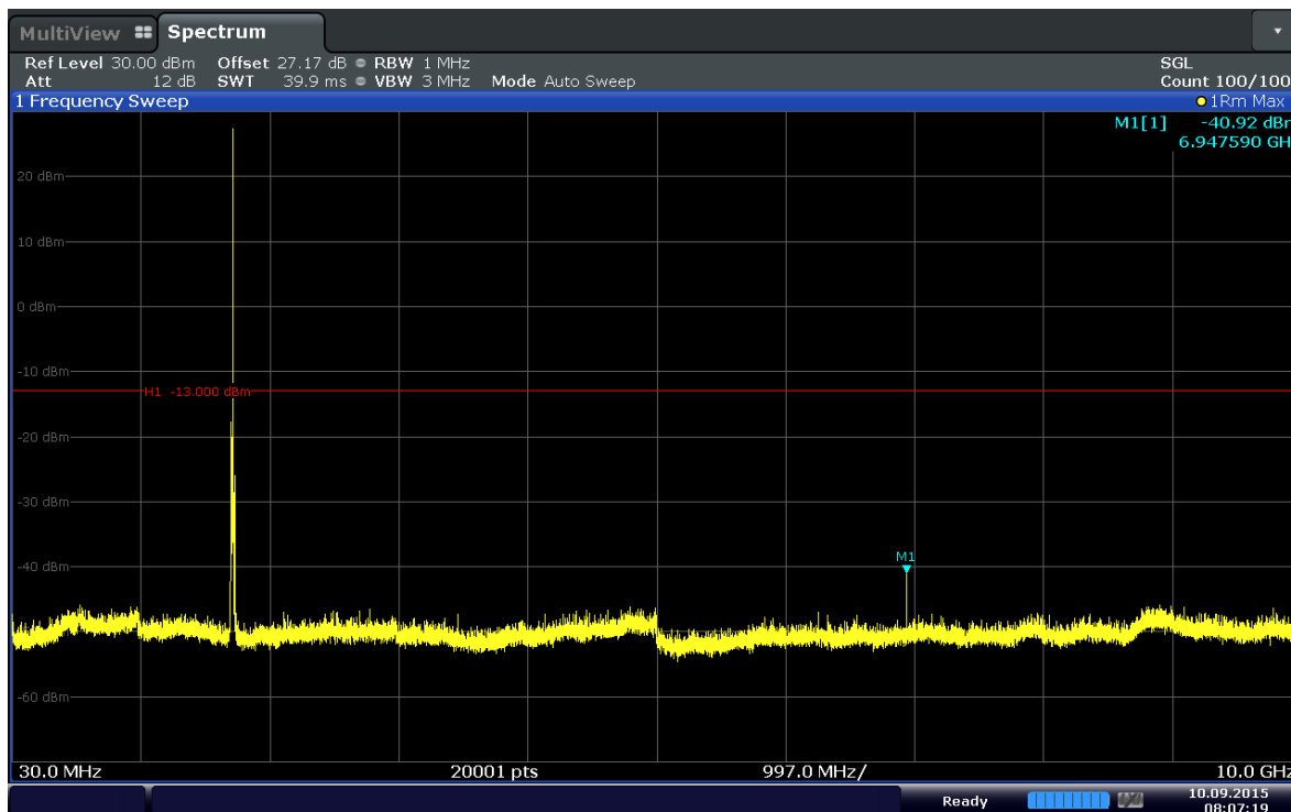
Plot 6-53. Conducted Spurious Plot (Band 4-10MHz-QPSK-RB Size 1-RB Offset 49-Ch.20175)
