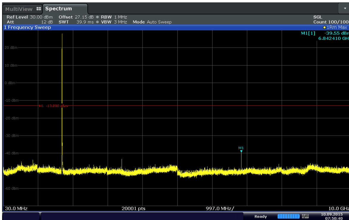
Plot 6-33. Conducted Spurious Plot (Band 4–1.4MHz–QPSK–RB Size 1–RB Offset 2–Ch.19957)
