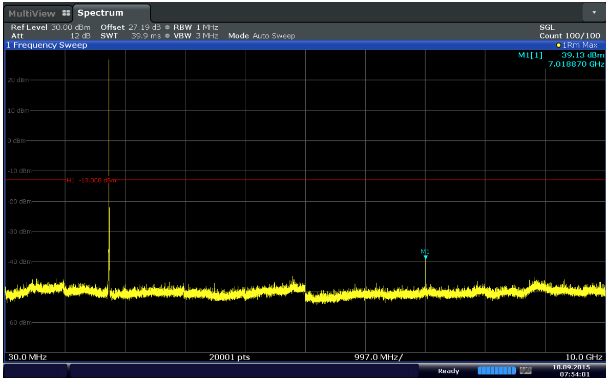
Plot 6-37. Conducted Spurious Plot (Band 4-1.4MHz-QPSK-RB Size 1-RB Offset 5-Ch.20393)
