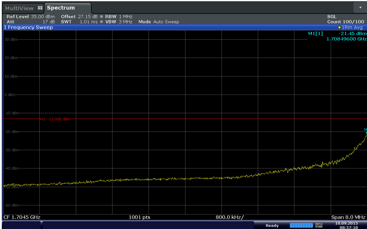
Plot 6-80. Extended Lower Band Edge Plot (Band 4 – 1.4MHz – QPSK – RB Size 6)
