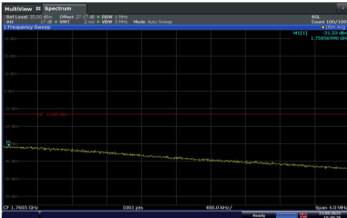
Plot 6-86. Extended Upper Band Edge Plot (Band 4 – 3MHz – QPSK – RB Size 15)
