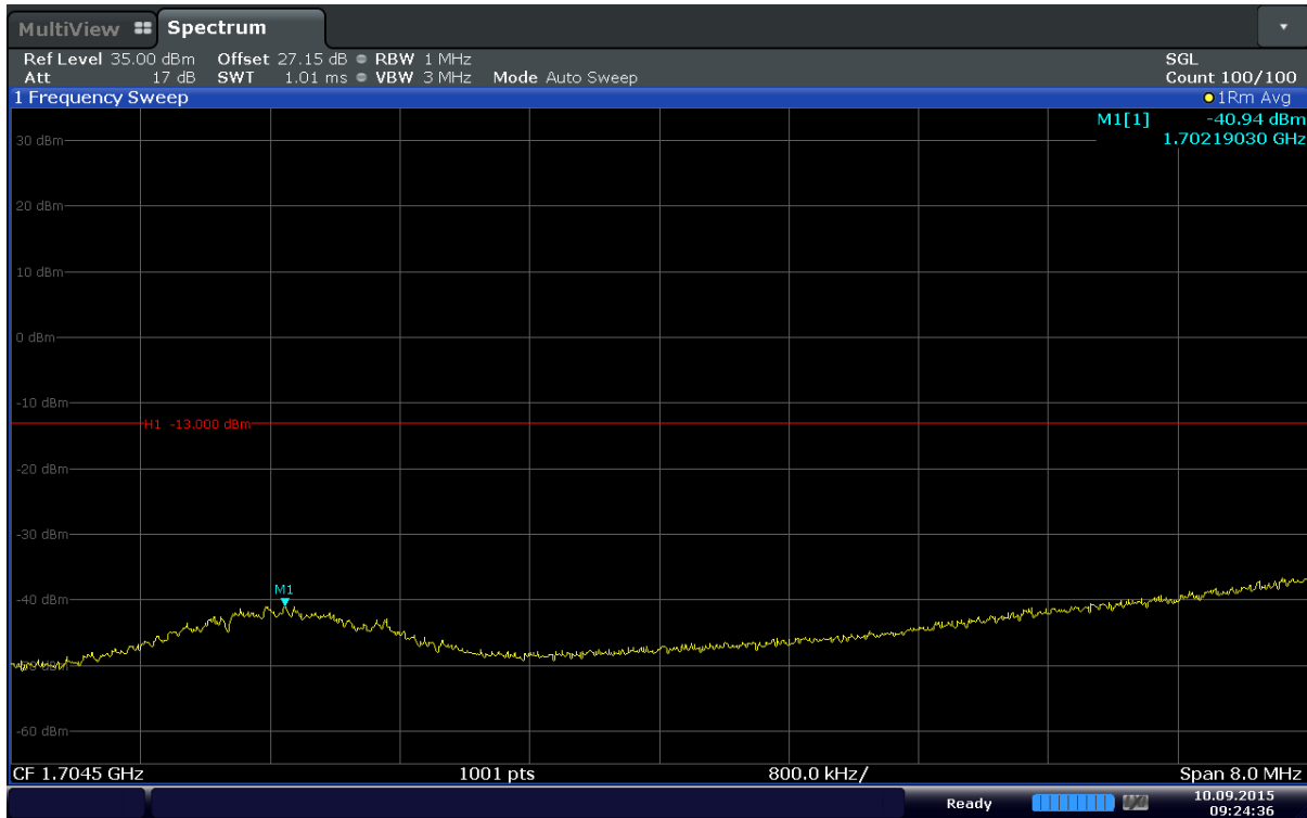
Plot 6-102. Extended Lower Band Edge Plot (Band 4 – 20MHz – QPSK – RB Size 1 – RB Offset 0)
