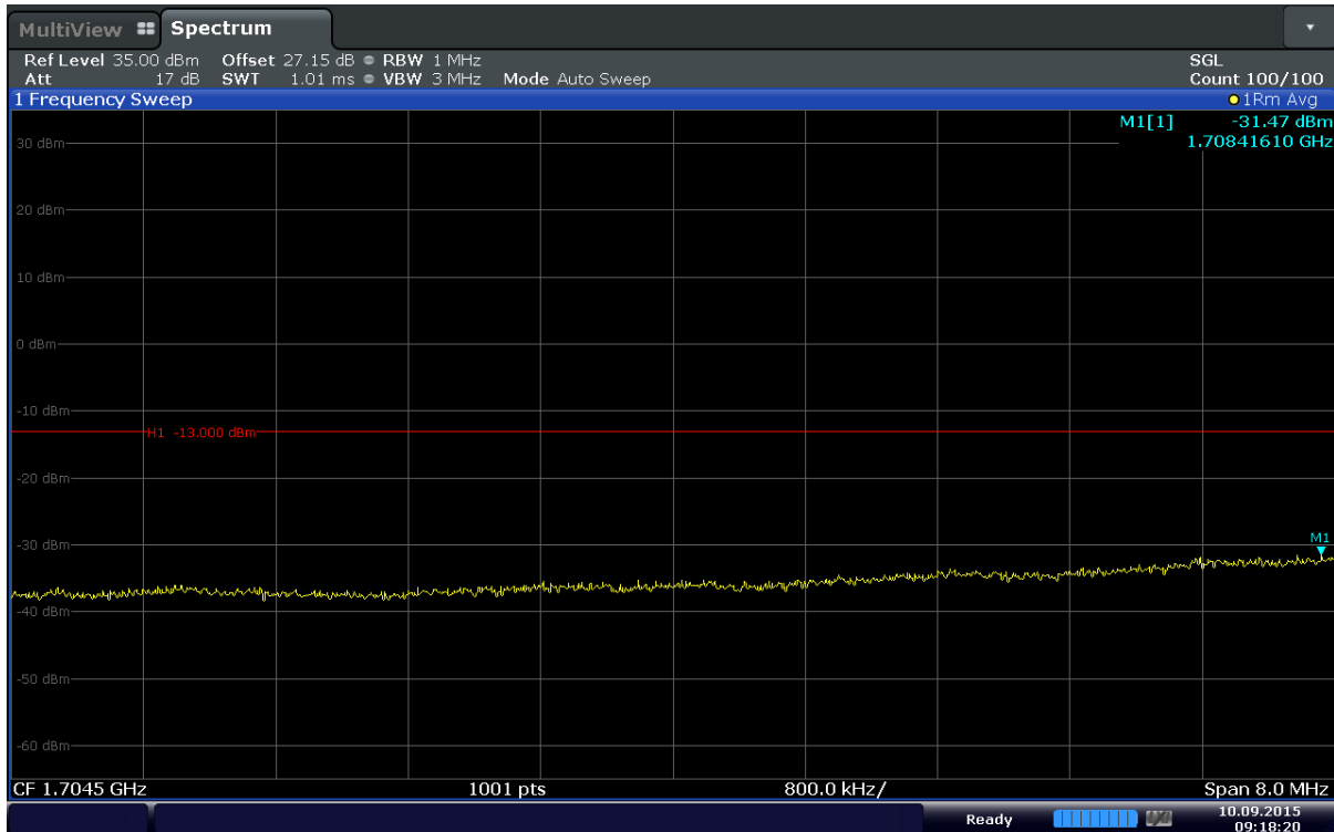
Plot 6-96. Extended Lower Band Edge Plot (Band 4 – 15MHz – QPSK – RB Size 75)
