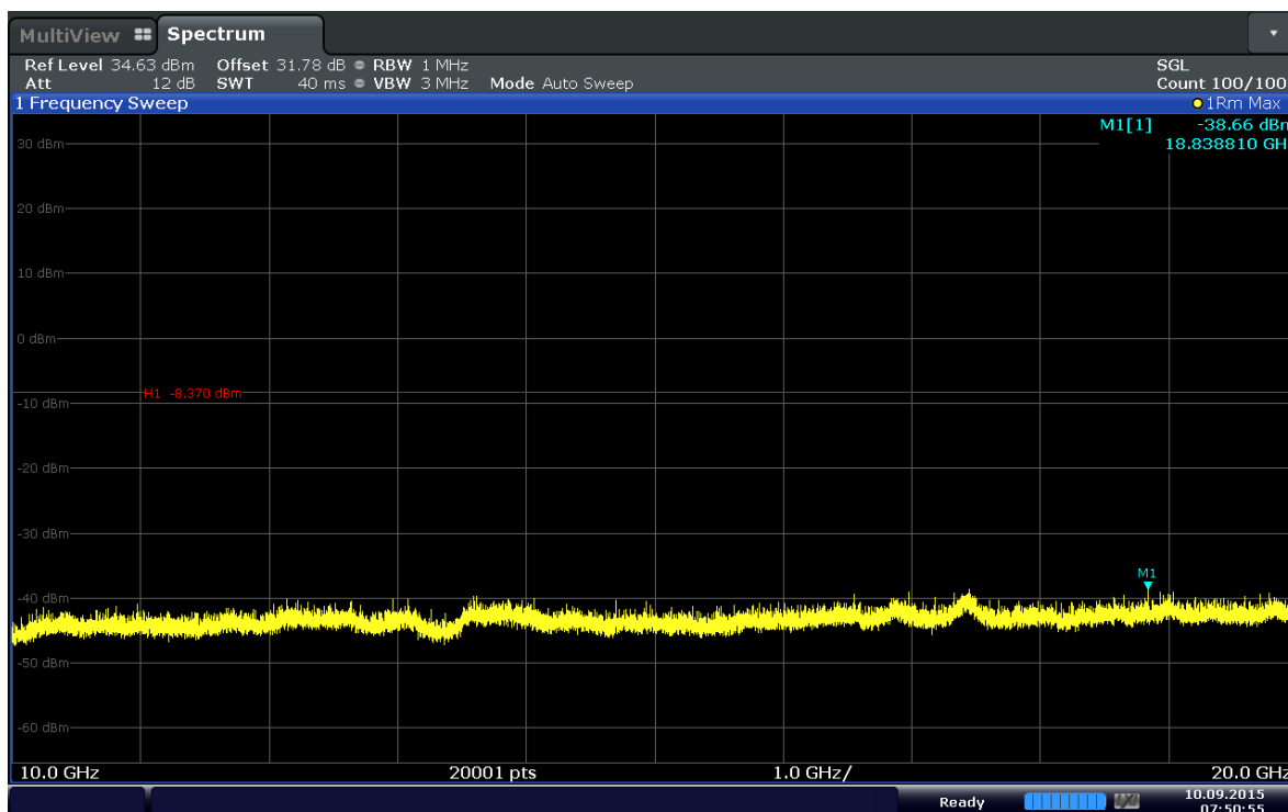
Plot 6-34. Conducted Spurious Plot (Band 4–1.4MHz–QPSK–RB Size 1–RB Offset 2–Ch.19957)
