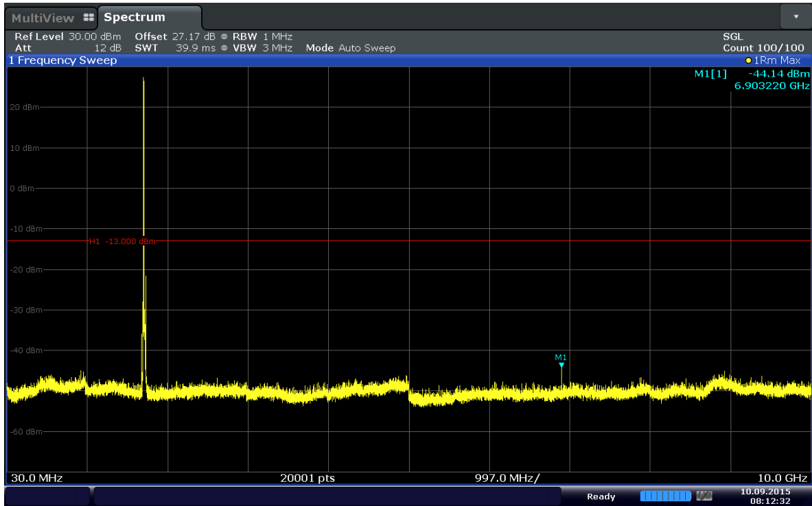
Plot 6-59. Conducted Spurious Plot (Band 4–15MHz–QPSK–RB Size 1–RB Offset 0–Ch.20175)
