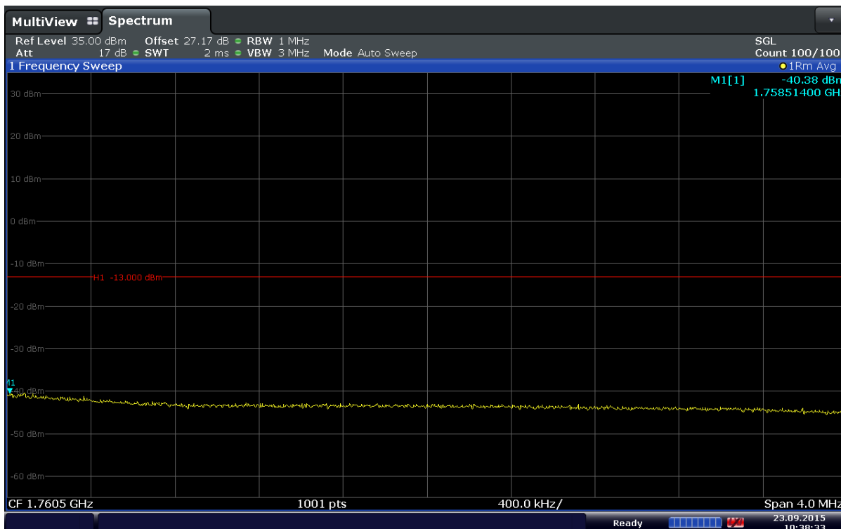
Plot 6-82. Extended Upper Band Edge Plot (Band 4 – 1.4MHz – QPSK – RB Size 6)
