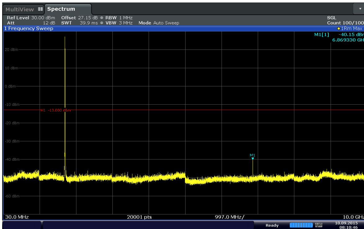
Plot 6-57. Conducted Spurious Plot (Band 4–15MHz–QPSK–RB Size 1–RB Offset 36–Ch.20025)
