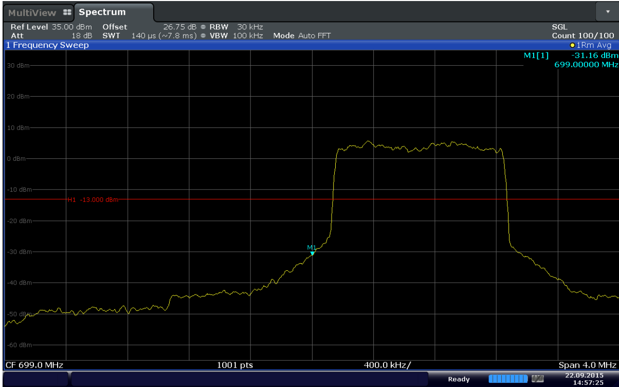
Plot 6-69. Lower Band Edge Plot (Band 12 – 1.4MHz – QPSK – RB Size 6)
