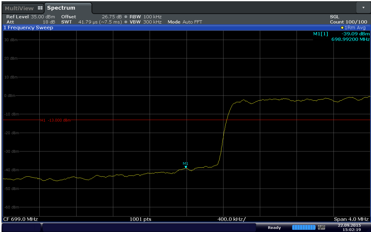
Plot 6-75. Lower Band Edge Plot (Band 12 – 10MHz – QPSK – RB Size 50)
