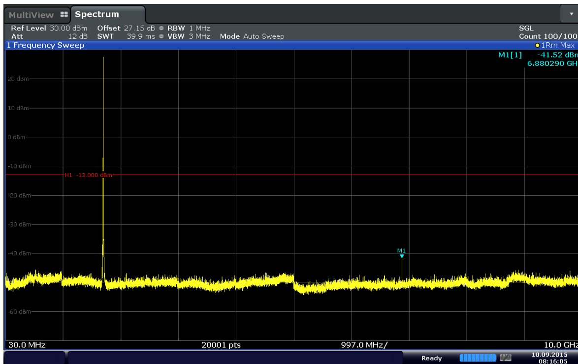
Plot 6-63. Conducted Spurious Plot (Band 4–20MHz–QPSK–RB Size 1–RB Offset 50–Ch.20050)
