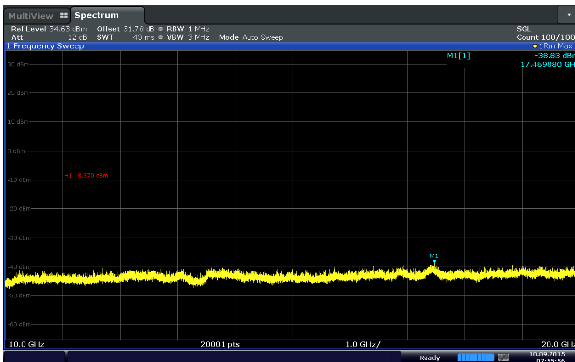
Plot 6-40. Conducted Spurious Plot (Band 4-3MHz-QPSK-RB Size 1-RB Offset 14-Ch.19965)
