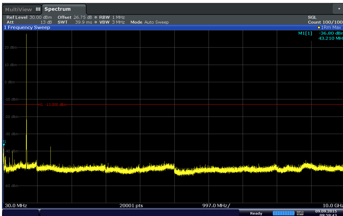
Plot 6-28. Conducted Spurious Plot (Band 12-5MHz-QPSK-RB Size 1-RB Offset 24-Ch.23095)
