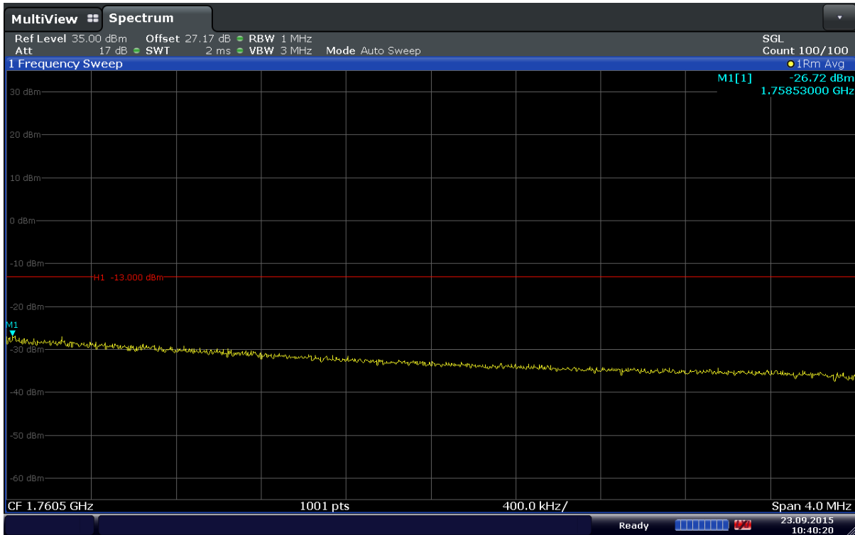
Plot 6-90. Extended Upper Band Edge Plot (Band 4 – 5MHz – QPSK – RB Size 25)
