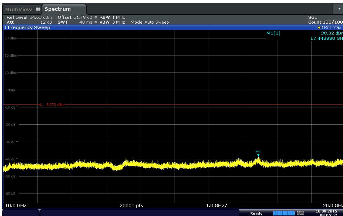
Plot 6-52. Conducted Spurious Plot (Band 4-10MHz-QPSK-RB Size 1-RB Offset 49-Ch.20000)
