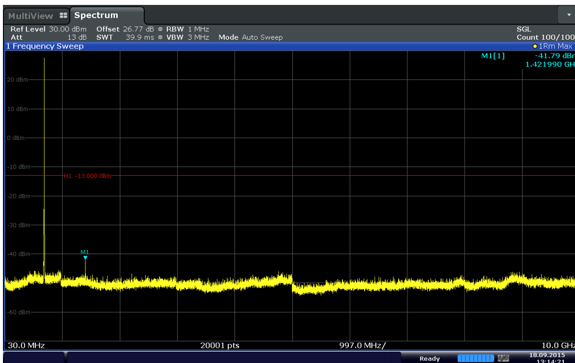
Plot 6-32. Conducted Spurious Plot (Band 12-10MHz-QPSK-RB Size 1-RB Offset 24-Ch.23130)
