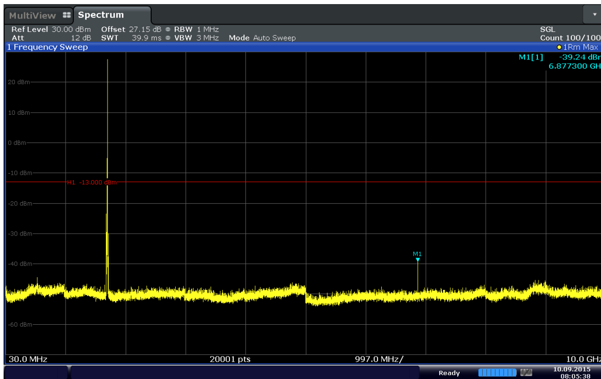
Plot 6-51. Conducted Spurious Plot (Band 4-10MHz-QPSK-RB Size 1-RB Offset 49-Ch.20000)
