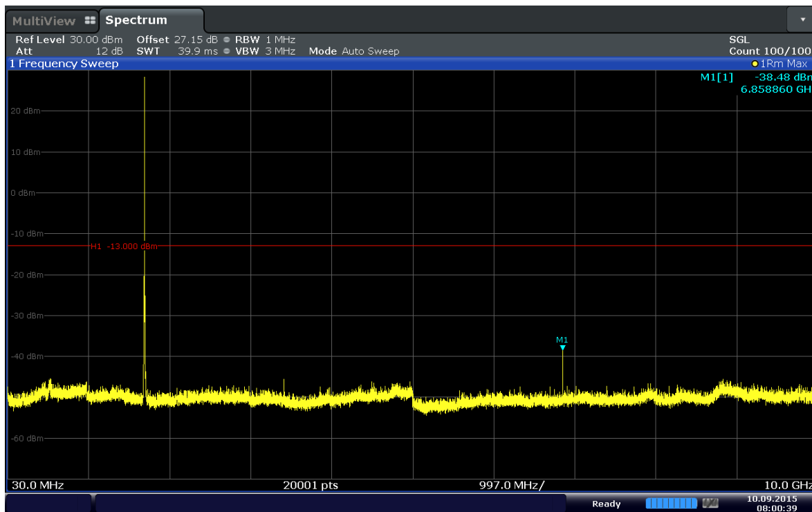
Plot 6-45. Conducted Spurious Plot (Band 4–5MHz–QPSK–RB Size 1–RB Offset 24–Ch.19975)
