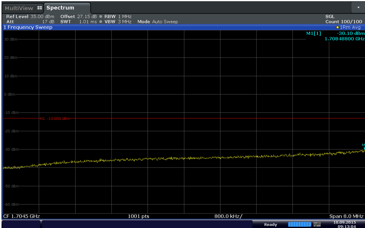
Plot 6-92. Extended Lower Band Edge Plot (Band 4 – 10MHz – QPSK – RB Size 50)
