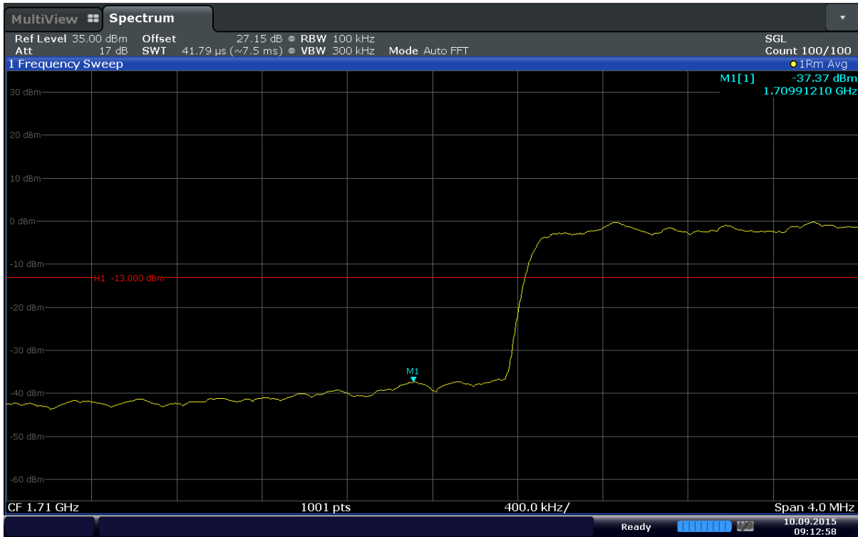
Plot 6-91. Lower Band Edge Plot (Band 4 – 10MHz – QPSK – RB Size 50)
