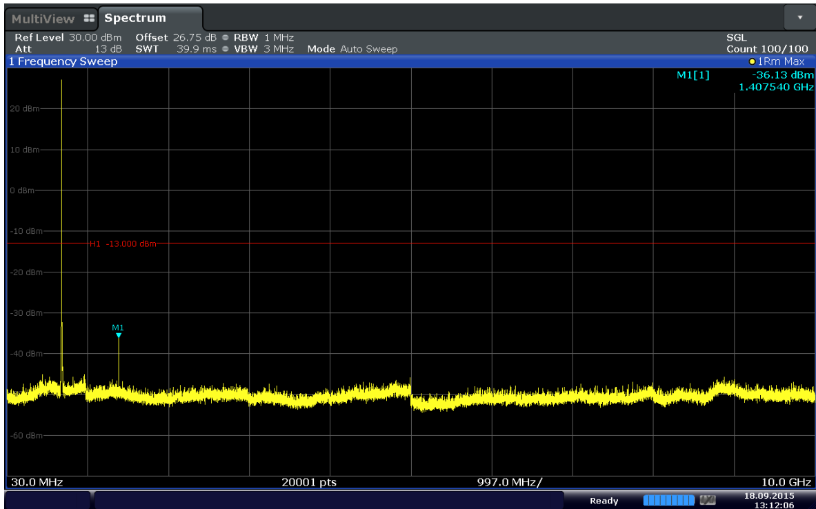
Plot 6-30. Conducted Spurious Plot (Band 12–10MHz–QPSK–RB Size 1–RB Offset 24–Ch.23060)
