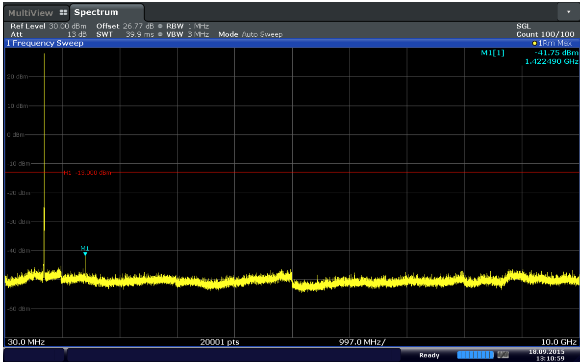
Plot 6-29. Conducted Spurious Plot (Band 12–5MHz–QPSK–RB Size 1–RB Offset 0–Ch.23155)
