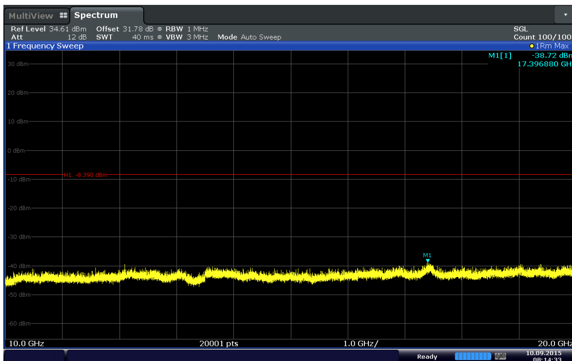
Plot 6-62. Conducted Spurious Plot (Band 4-15MHz-QPSK-RB Size 1-RB Offset 74-Ch.20325)
