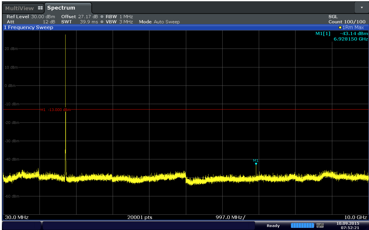
Plot 6-35. Conducted Spurious Plot (Band 4-1.4MHz-QPSK-RB Size 1-RB Offset 0-Ch.20175)
