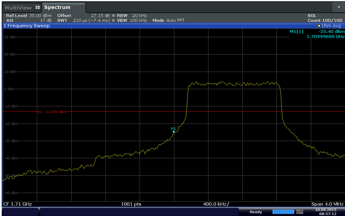
Plot 6-79. Lower Band Edge Plot (Band 4 – 1.4MHz – QPSK – RB Size 6)
