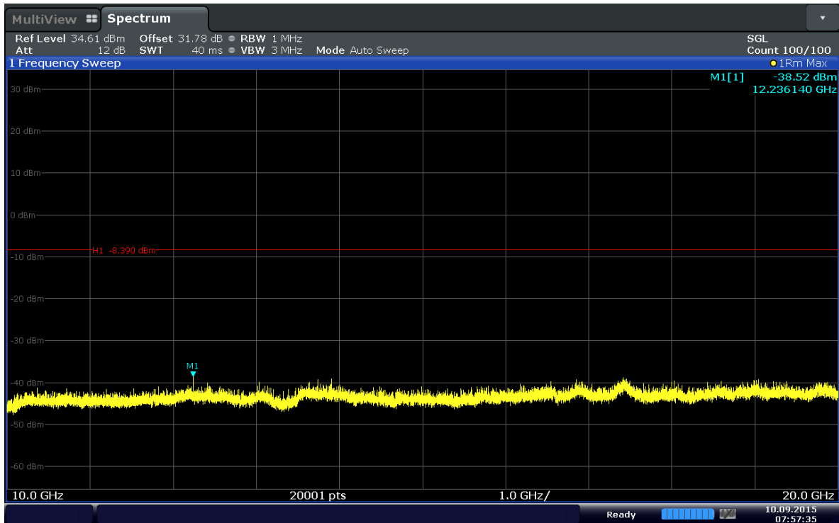
Plot 6-42. Conducted Spurious Plot (Band 4-3MHz-QPSK-RB Size 1-RB Offset 14-Ch.20175)
