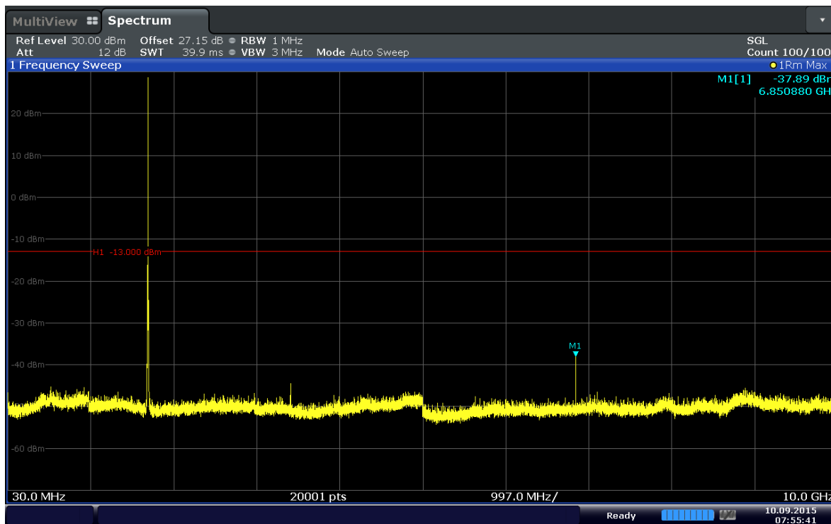
Plot 6-39. Conducted Spurious Plot (Band 4-3MHz-QPSK-RB Size 1-RB Offset 14-Ch.19965)
