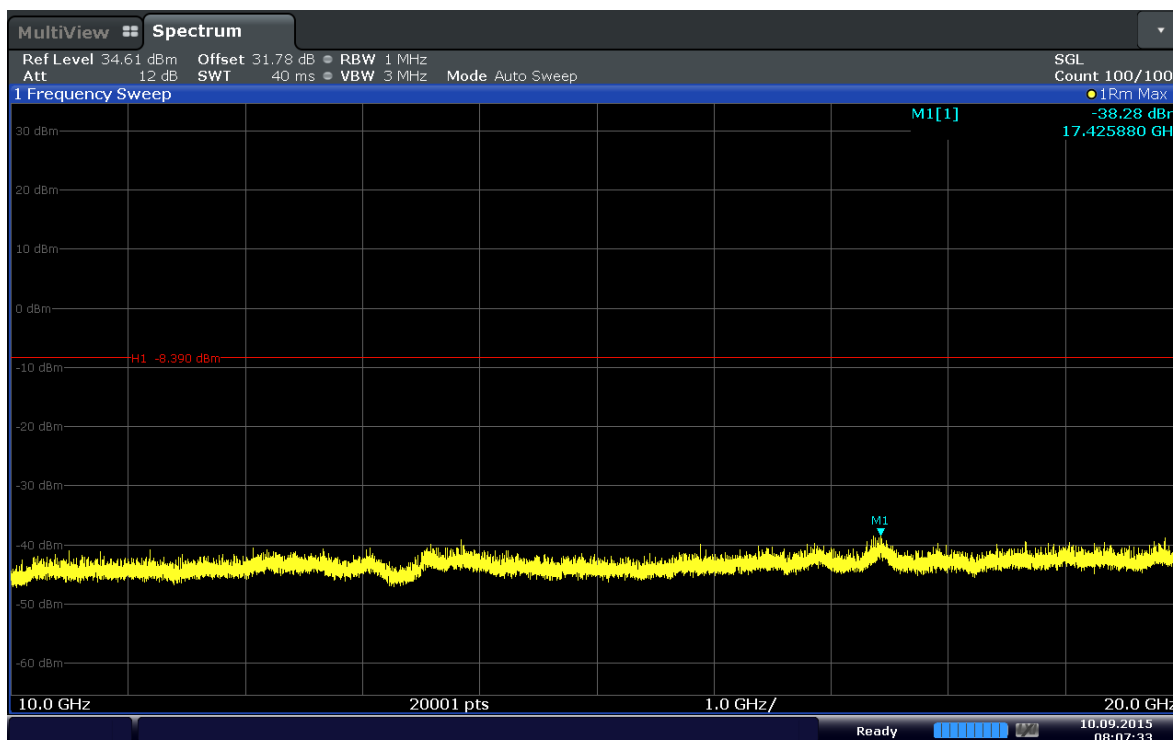
Plot 6-54. Conducted Spurious Plot (Band 4-10MHz-QPSK-RB Size 1-RB Offset 49-Ch.20175)
