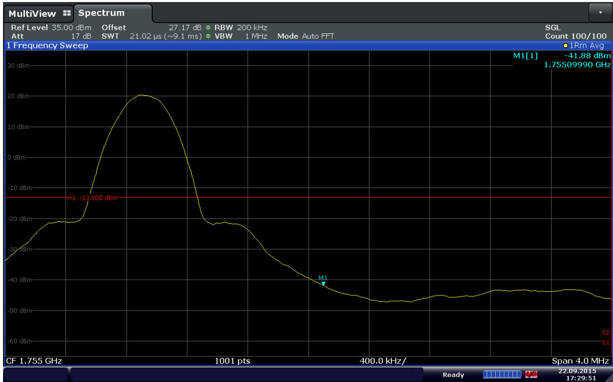
Plot 6-105. Upper Band Edge Plot (Band 4 – 20MHz – QPSK – RB Size 1 – RB Offset 49)
