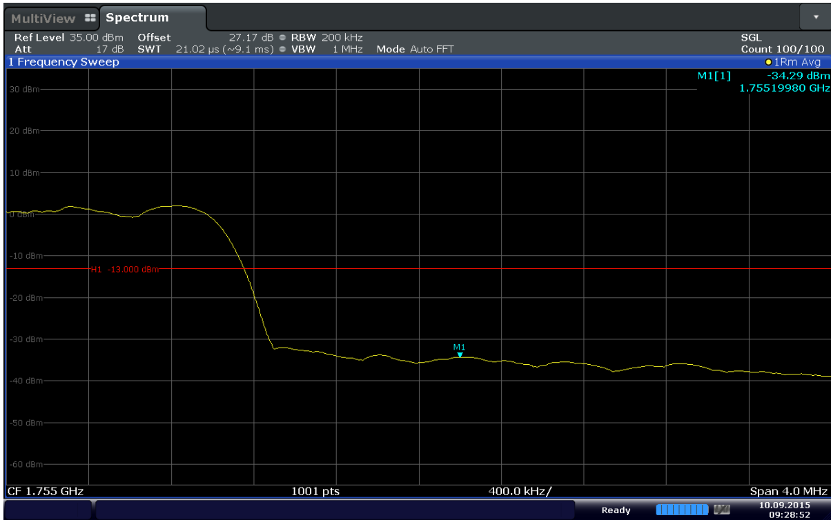
Plot 6-103. Upper Band Edge Plot (Band 4 – 20MHz – QPSK – RB Size 100)
