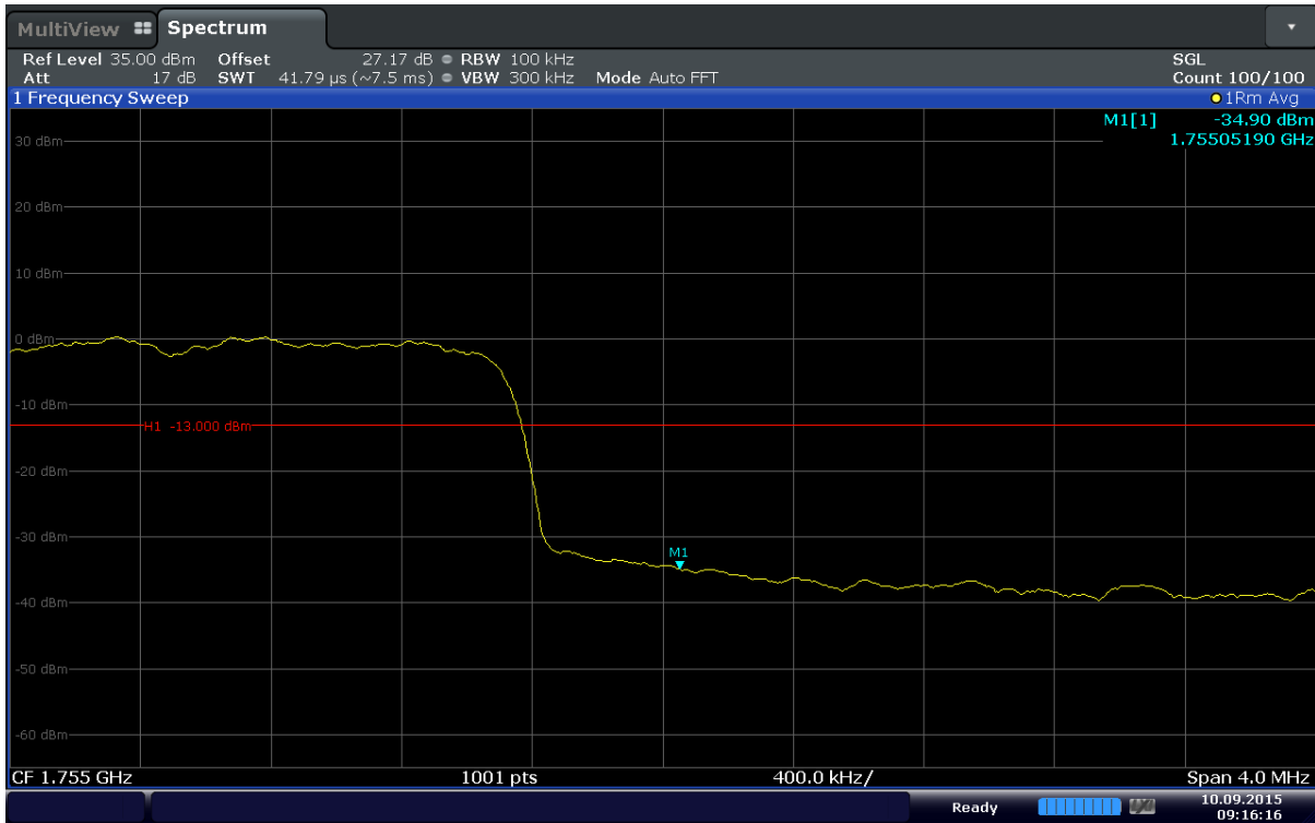
Plot 6-93. Upper Band Edge Plot (Band 4 – 10MHz – QPSK – RB Size 50)
