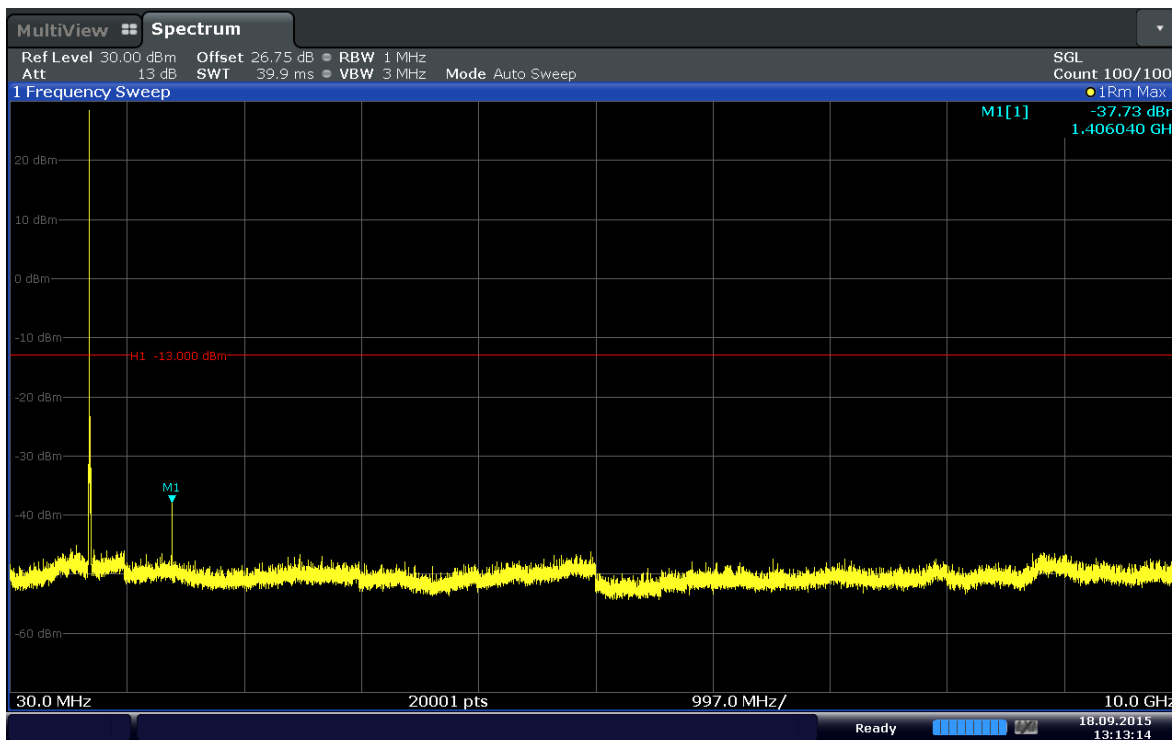
Plot 6-31. Conducted Spurious Plot (Band 12-10MHz-QPSK-RB Size 1-RB Offset 0-Ch.23095)
