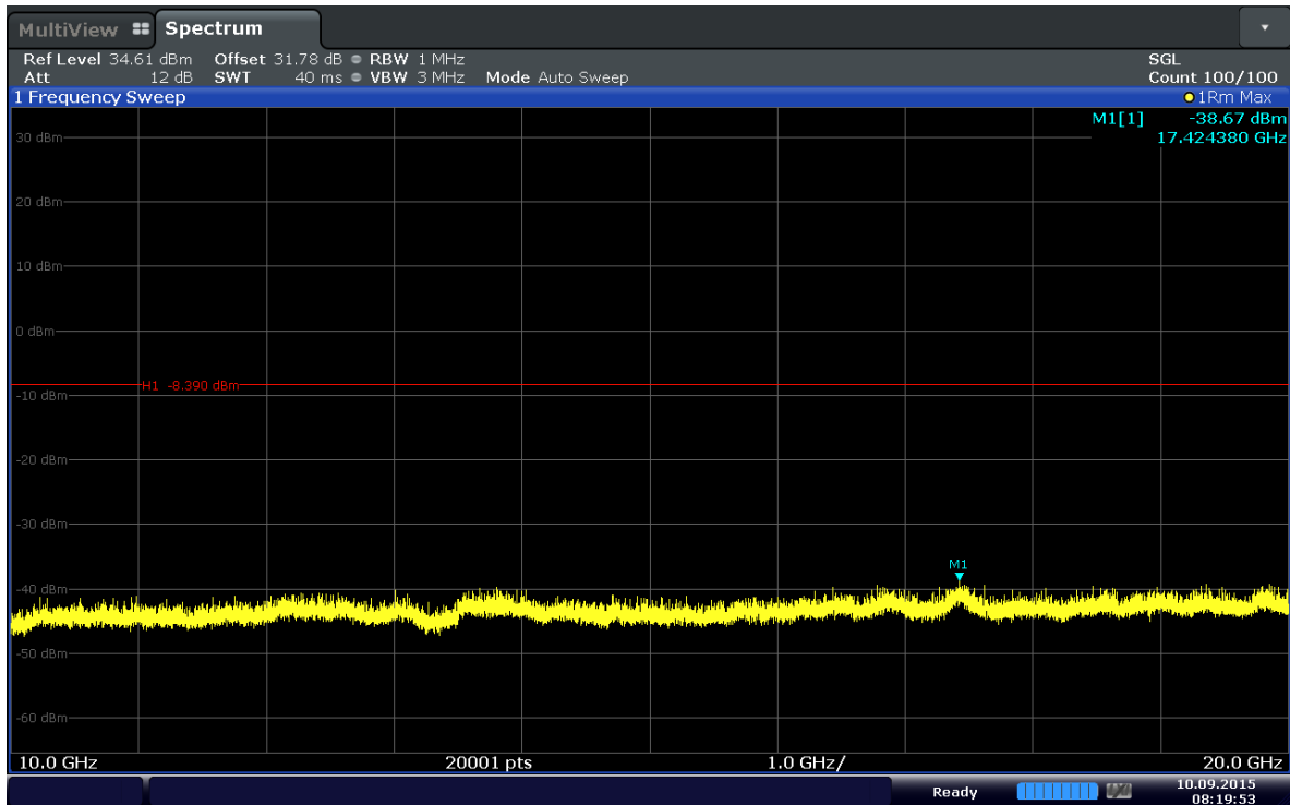
Plot 6-68. Conducted Spurious Plot (Band 4–20MHz–QPSK–RB Size 1–RB Offset 50–Ch.20300)
