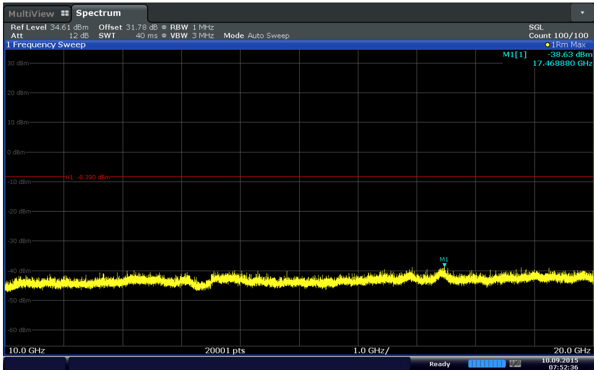
Plot 6-36. Conducted Spurious Plot (Band 4-1.4MHz-QPSK-RB Size 1-RB Offset 0-Ch.20175)
