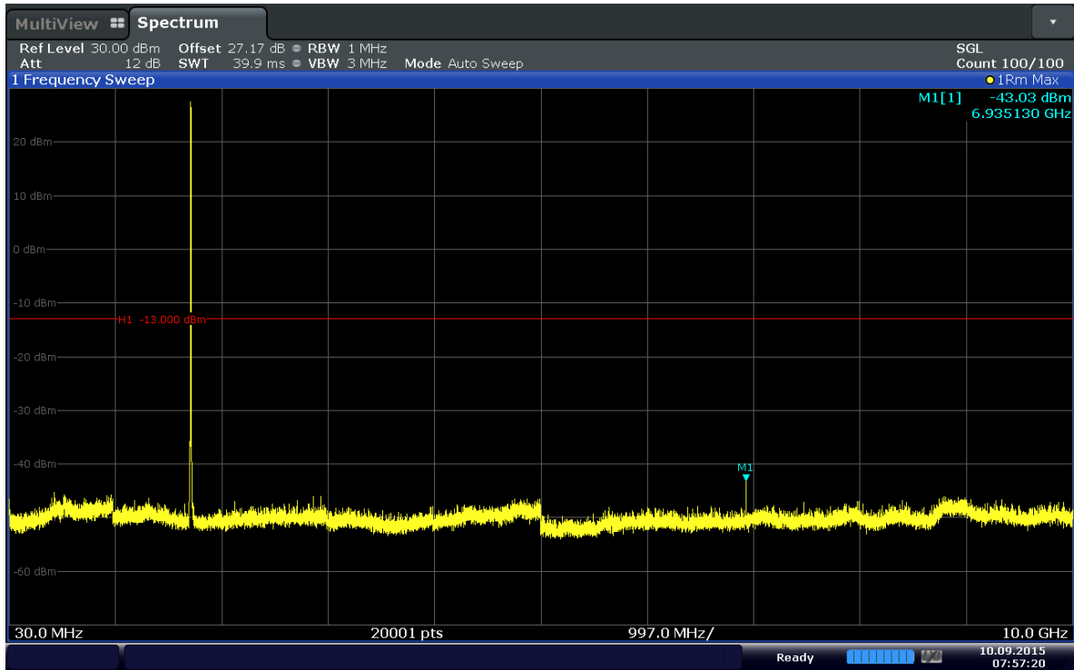
Plot 6-41. Conducted Spurious Plot (Band 4-3MHz-QPSK-RB Size 1-RB Offset 14-Ch.20175)
