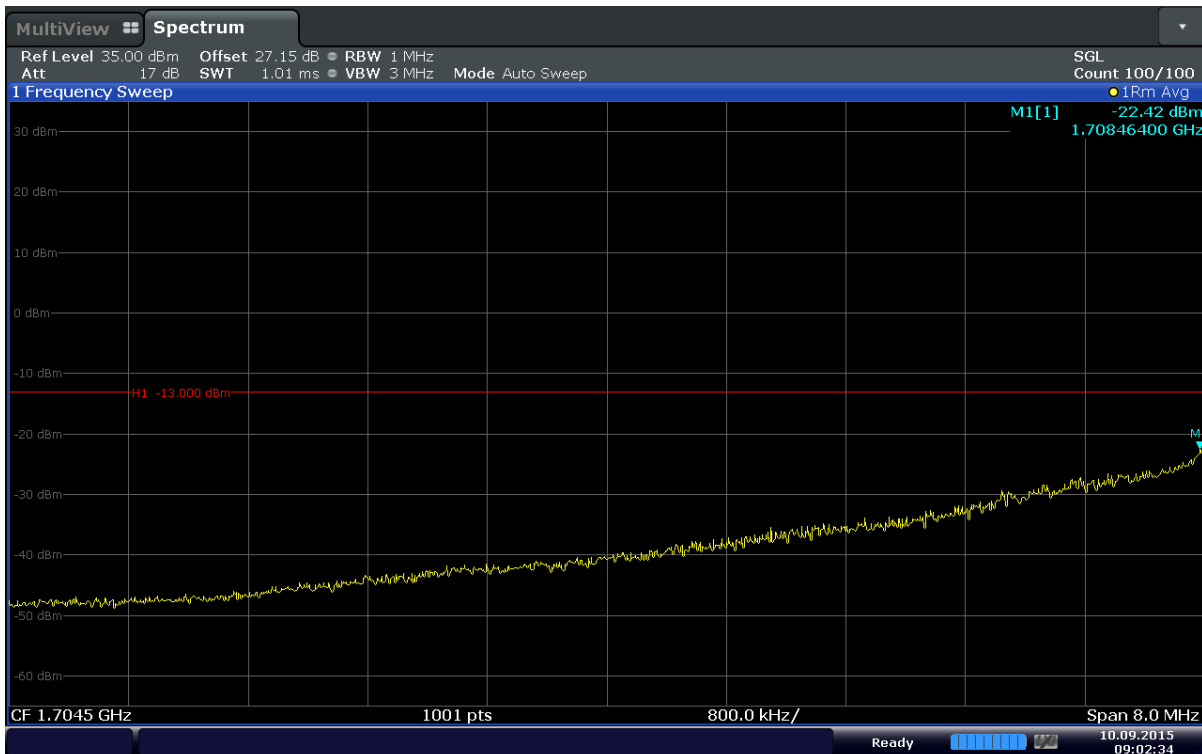
Plot 6-84. Extended Lower Band Edge Plot (Band 4 – 3MHz – QPSK – RB Size 15)
