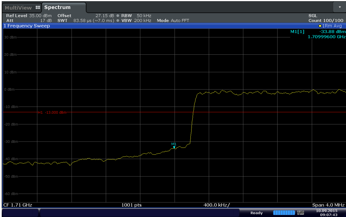
Plot 6-87. Lower Band Edge Plot (Band 4 – 5MHz – QPSK – RB Size 25)
