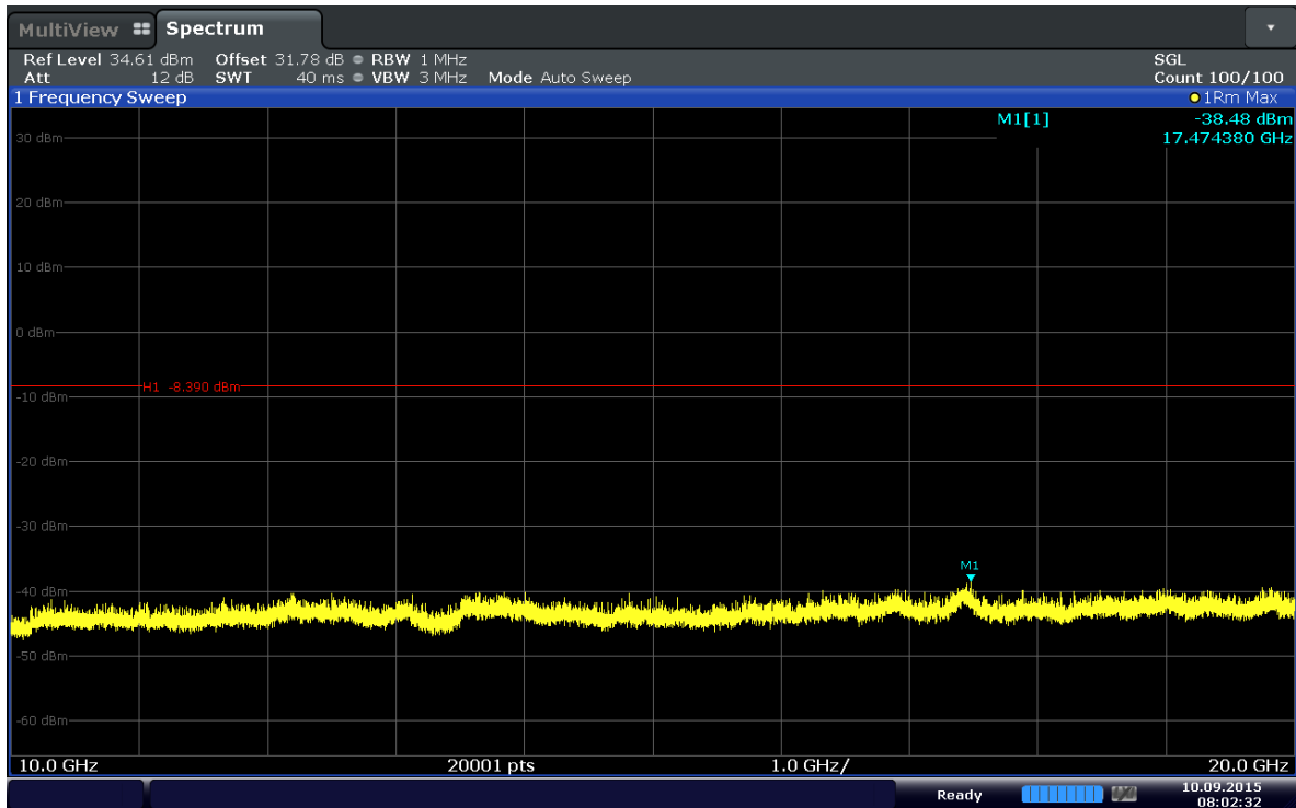
Plot 6-48. Conducted Spurious Plot (Band 4–5MHz–QPSK–RB Size 1–RB Offset 24–Ch.20175)
