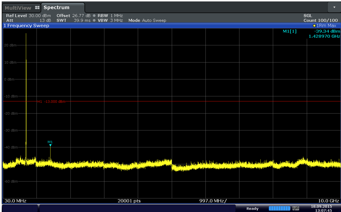
Plot 6-26. Conducted Spurious Plot (Band 12-3MHz-QPSK-RB Size 1-RB Offset 7-Ch.23165)
