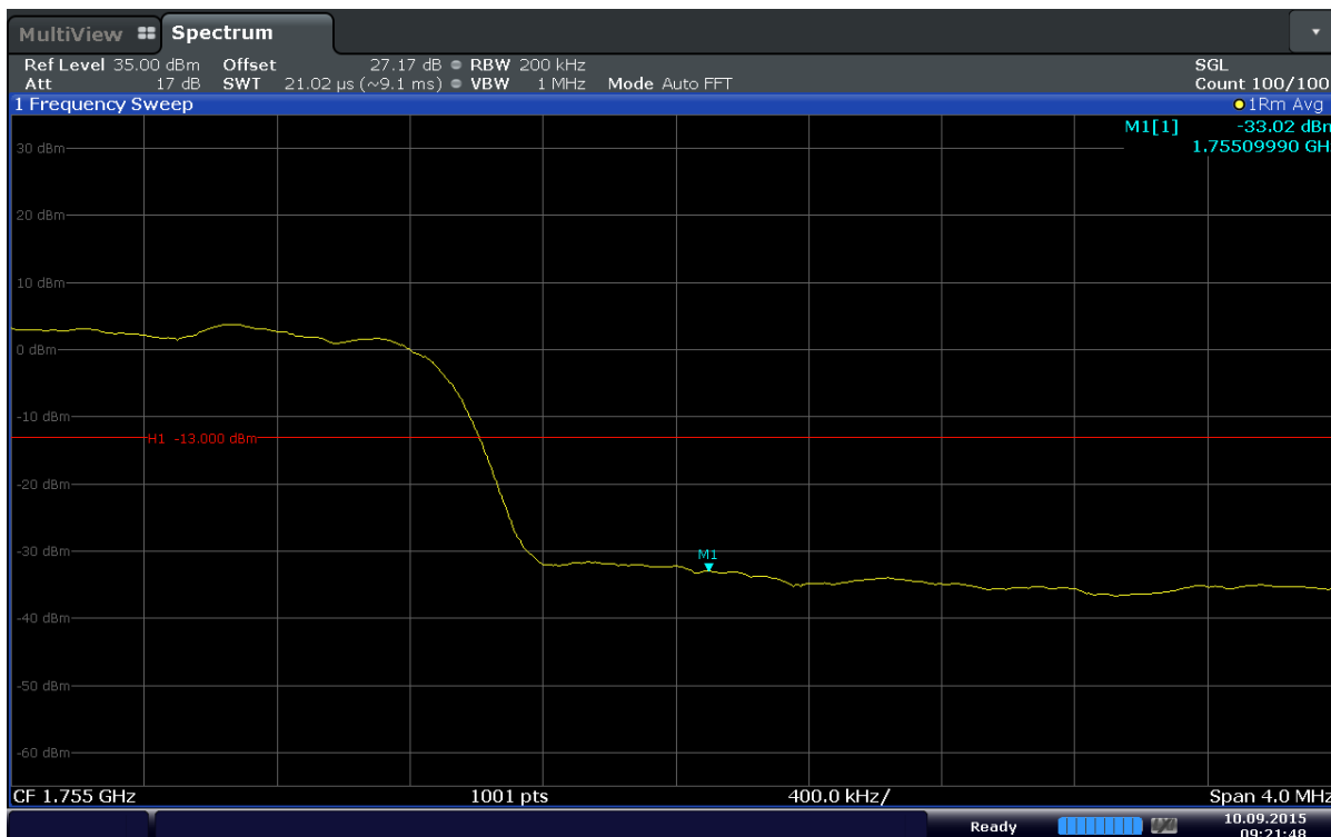
Plot 6-97. Upper Band Edge Plot (Band 4 – 15MHz – QPSK – RB Size 75)
