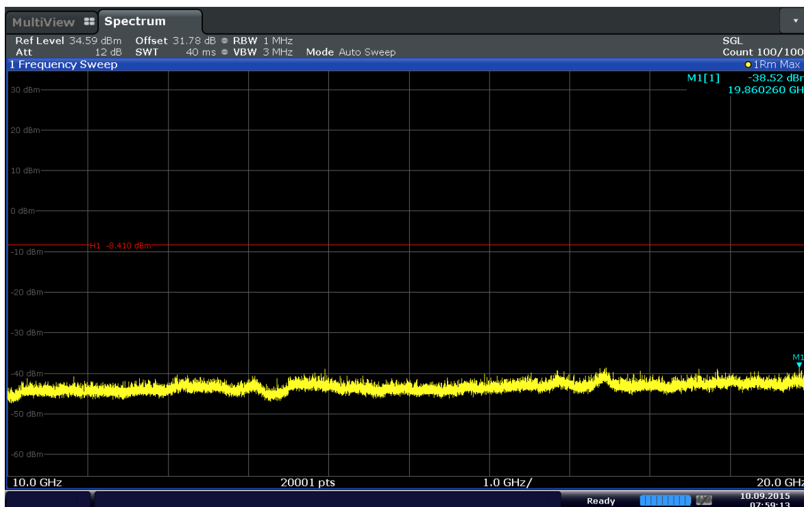
Plot 6-44. Conducted Spurious Plot (Band 4-3MHz-QPSK-RB Size 1-RB Offset 14-Ch.20385)
