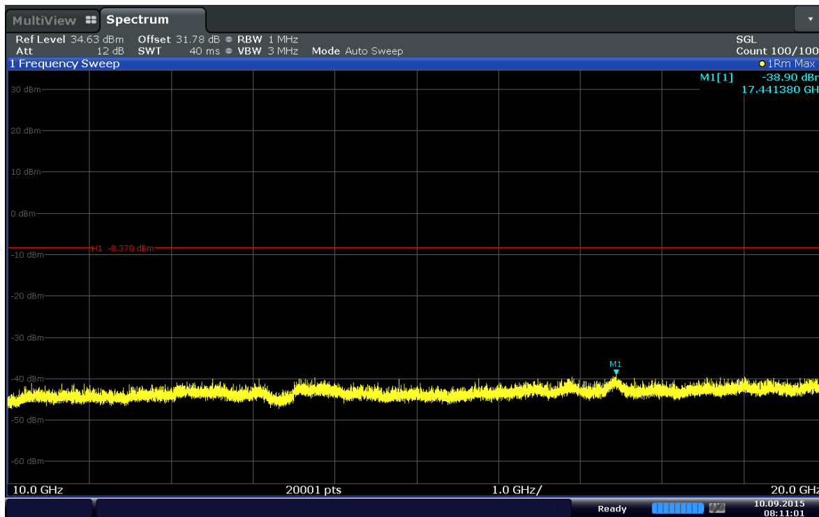
Plot 6-58. Conducted Spurious Plot (Band 4–15MHz–QPSK–RB Size 1–RB Offset 36–Ch.20025)
