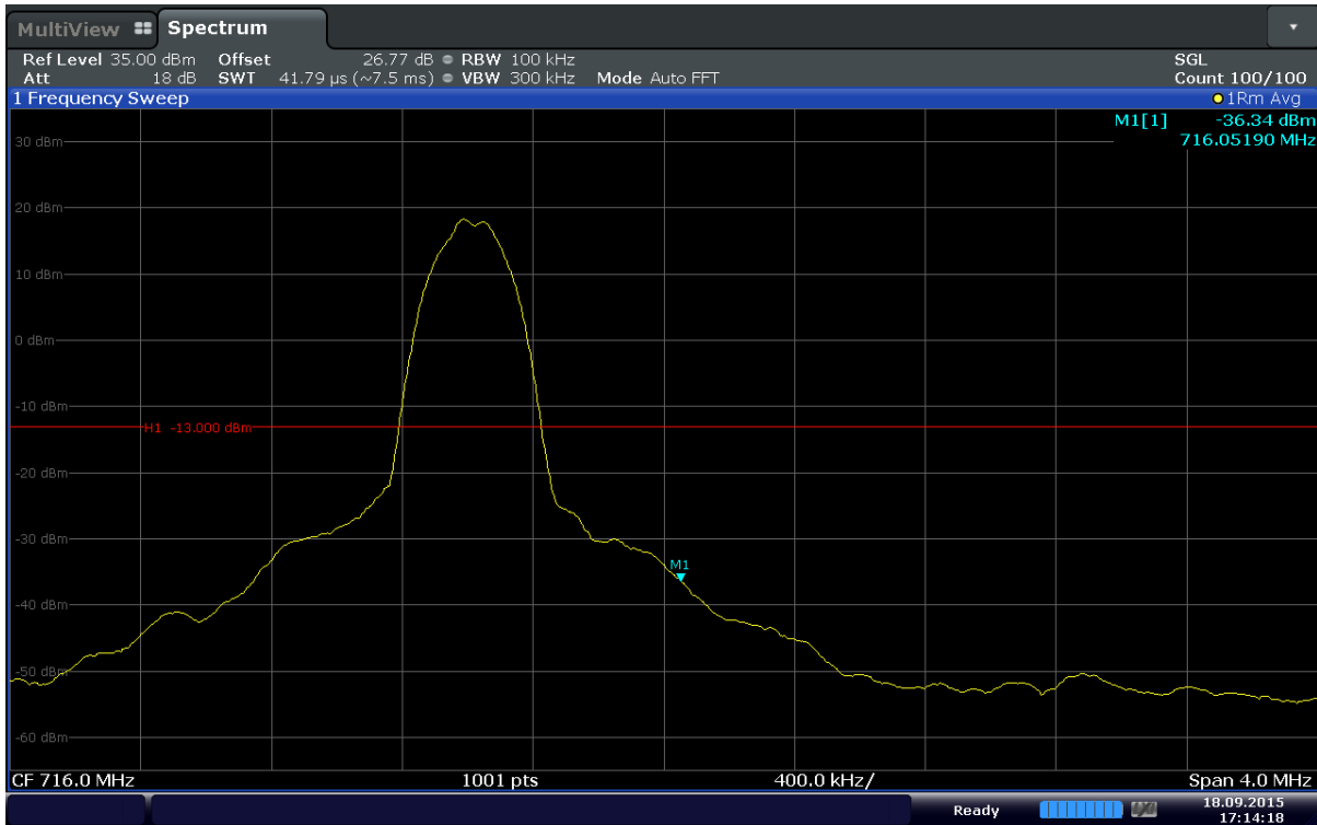
Plot 6-78. Upper Band Edge Plot (Band 12 – 10MHz – QPSK – RB Size 1 – RB Offset 49)
