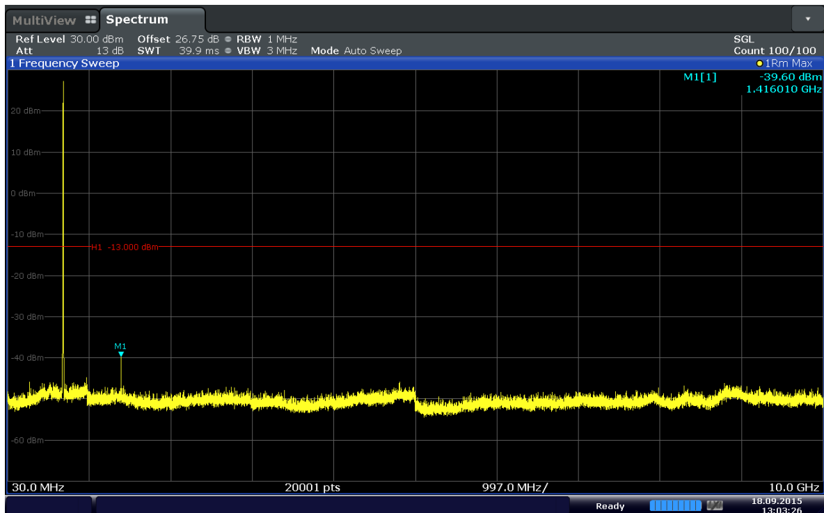
Plot 6-21. Conducted Spurious Plot (Band 12-1.4MHz-QPSK-RB Size 1-RB Offset 5-Ch.23017)
