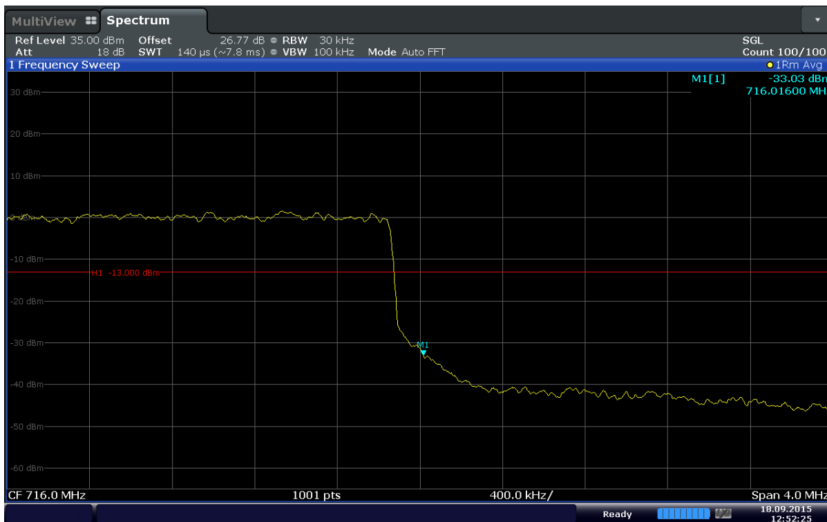
Plot 6-72. Upper Band Edge Plot (Band 12 – 3MHz – QPSK – RB Size 15)
