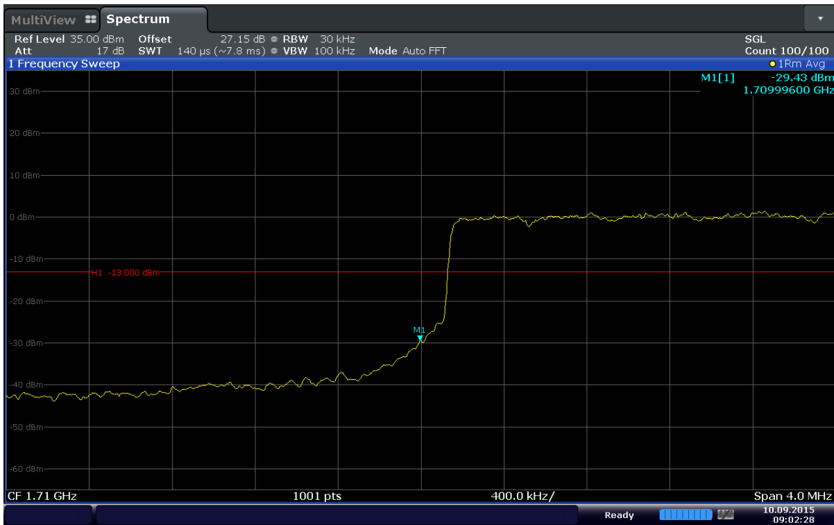
Plot 6-83. Lower Band Edge Plot (Band 4 – 3MHz – QPSK – RB Size 15)
