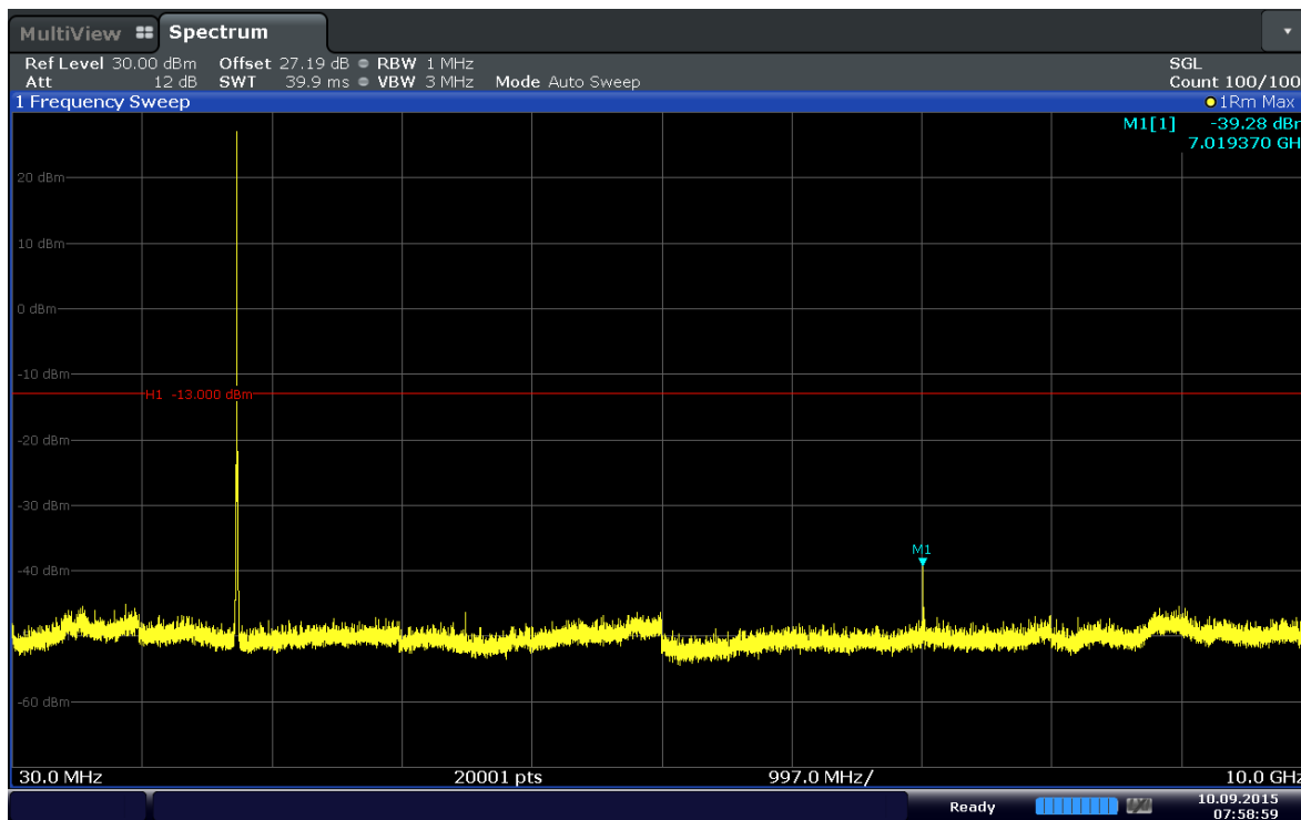
Plot 6-43. Conducted Spurious Plot (Band 4-3MHz-QPSK-RB Size 1-RB Offset 14-Ch.20385)
