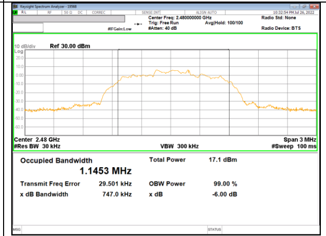
99% bandwidth / 78 CHANNEL
