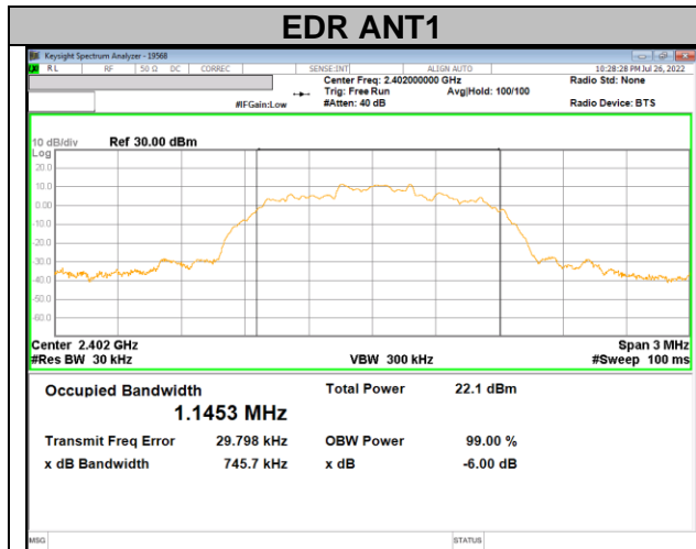
99% bandwidth / 0 CHANNEL
