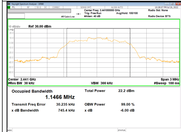
99% bandwidth / 39 CHANNEL
