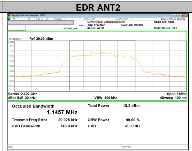
99% bandwidth / 0 CHANNEL
