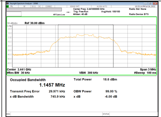
99% bandwidth / 39 CHANNEL
