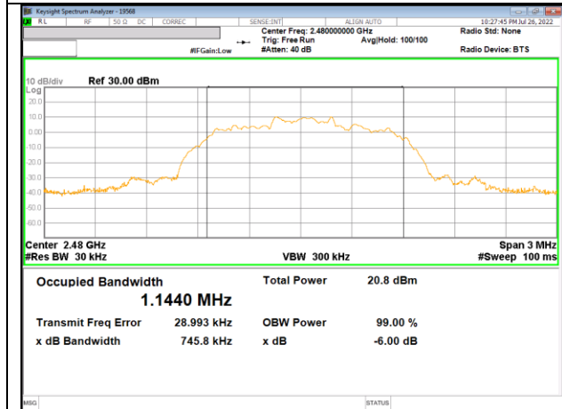
99% bandwidth / 78 CHANNEL
