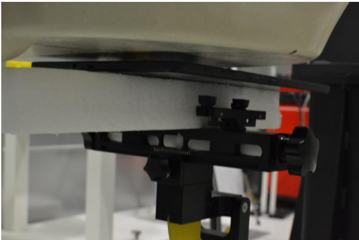
SAR Test Setup Photo 2: Back Side at 0.9 cm
