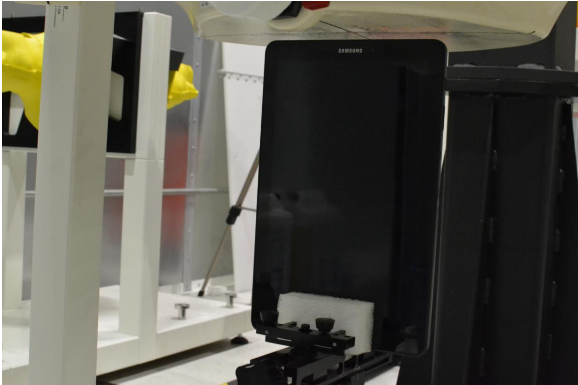
SAR Test Setup Photo 5: Top Edge at 0.5 cm
