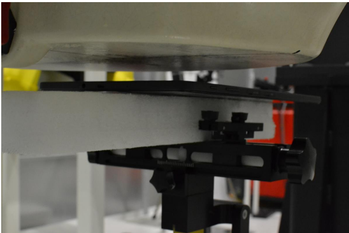
SAR Test Setup Photo 1: Back Side at 1.8 cm
