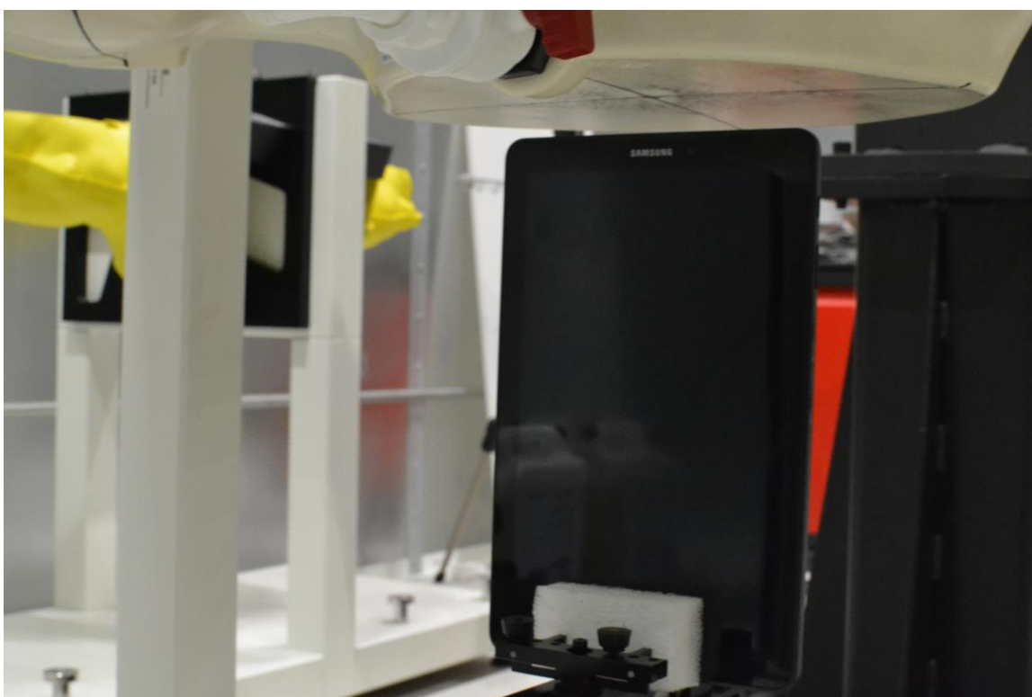
SAR Test Setup Photo 4: Top Edge at 1.4 cm
