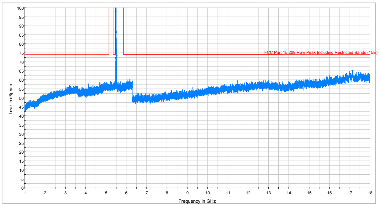
Plot 7-84. Radiated Spurious Plot above 1GHz (802.11a – U2C Ch. 120, Ant. Pol. V)
