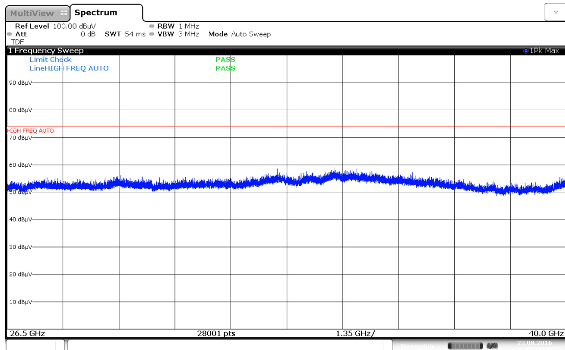
Plot 7-88. Radiated Spurious Plot above 26GHz (802.11a – Ant. Pol. H)
