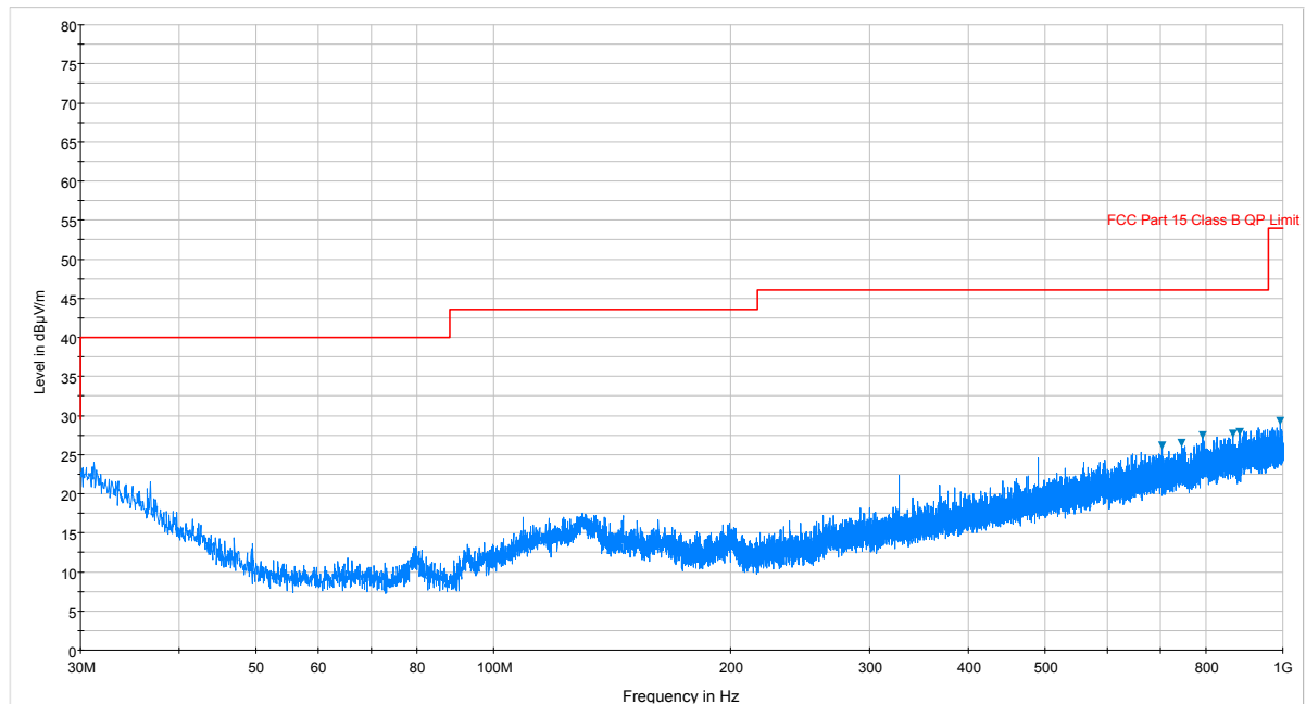
Plot 7-111. Radiated Spurious Plot below 1GHz (802.11a – U3 Ch. 157, Ant. Pol. H)
