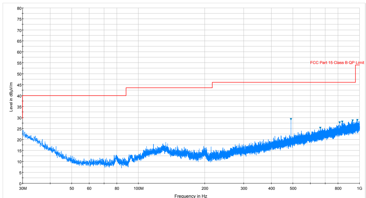
Plot 7-112. Radiated Spurious Plot below 1GHz (802.11a – U3 Ch. 157, Ant. Pol. V)
