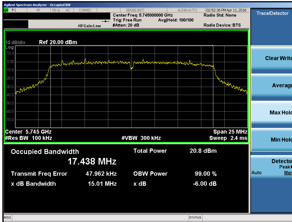
Plot 7-34. 6dB Bandwidth Plot (20MHz BW 802.11n (UNII Band 3) – Ch. 149)
