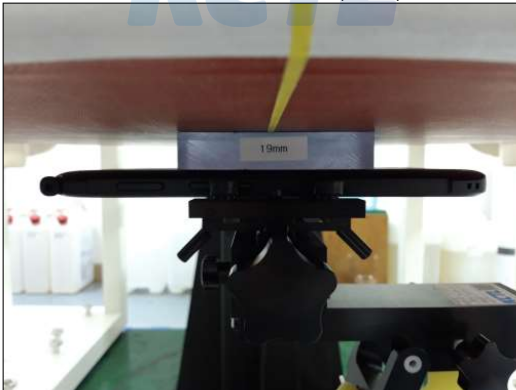
Rear With Protective Cover (19 mm)
