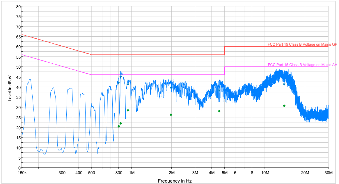
Plot 6-63. Line Conducted Plot with 802.11b (L1)
