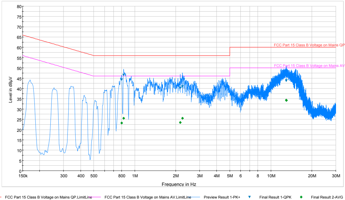
Plot 6-64. Line Conducted Plot with 802.11b (N)
