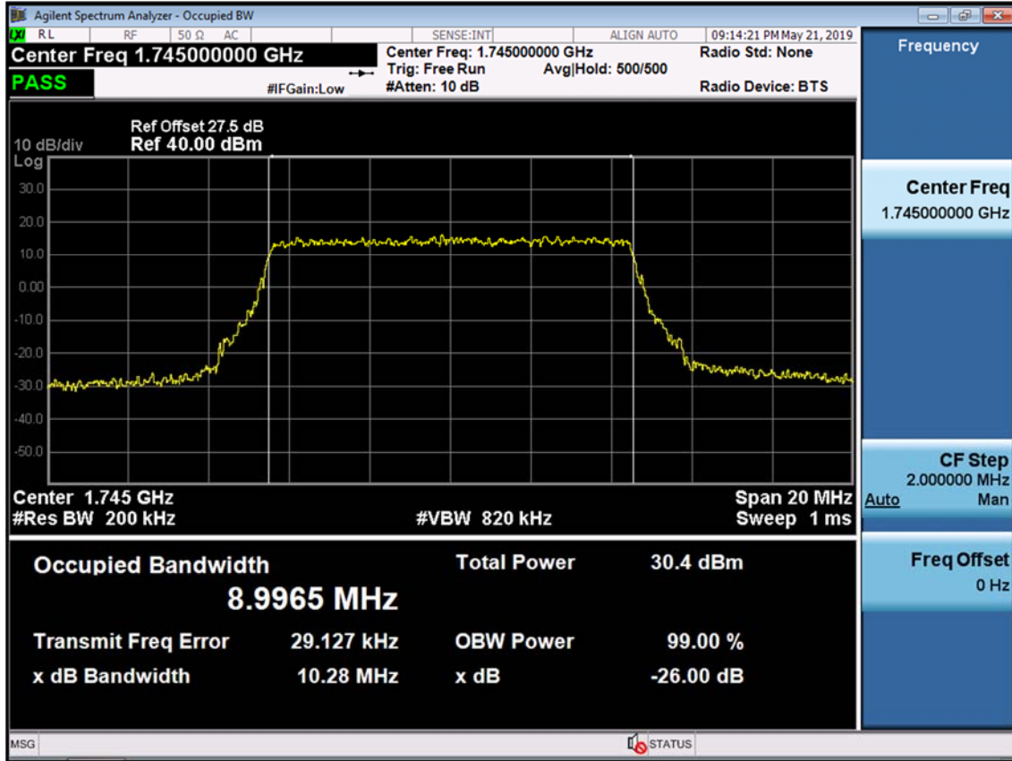
BAND 66/4. Occupied Bandwidth Plot (10M BW Ch.132322 QPSK RB 50)
