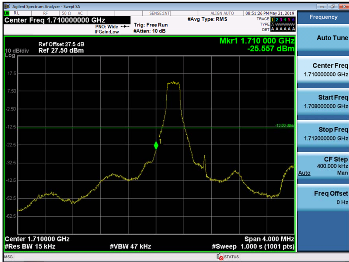
BAND 66/4. Lower Band Edge Plot (1.4M BW Ch.131979 QPSK RB 1, Offset 0) -1
