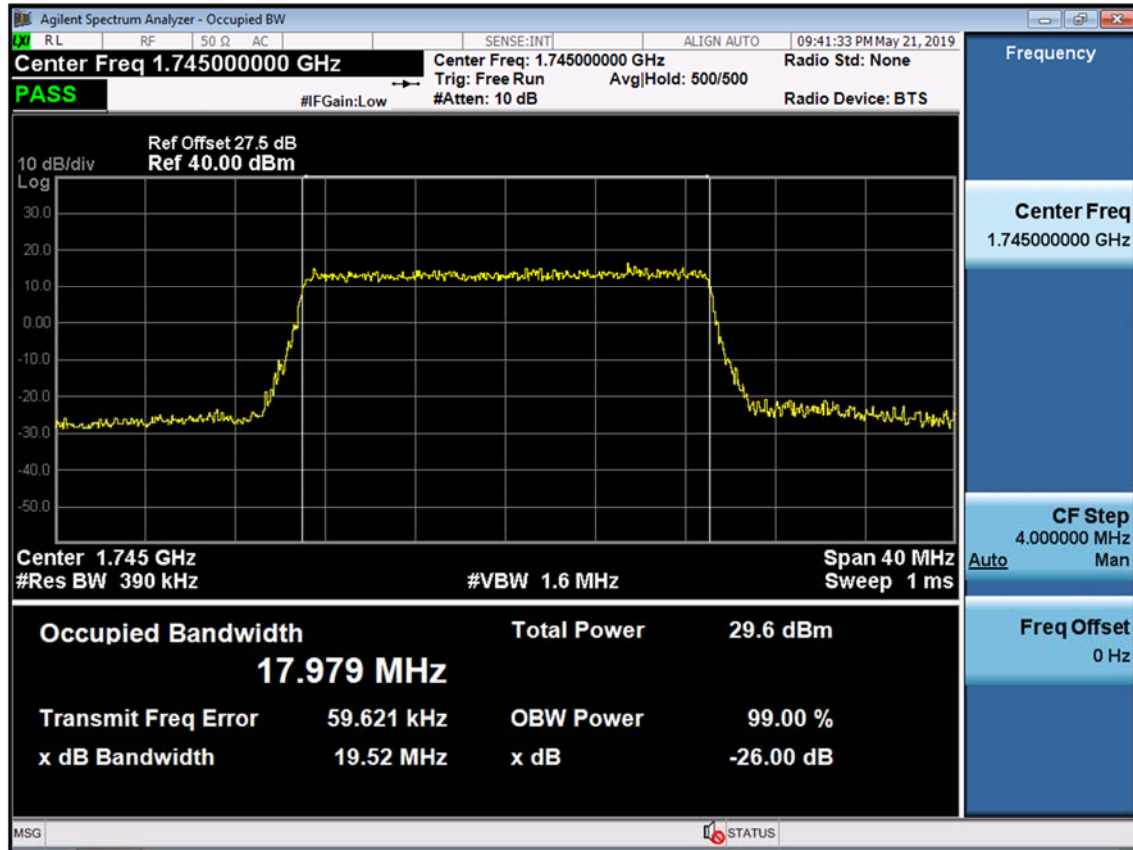
BAND 66/4. Occupied Bandwidth Plot (20M BW Ch.132322 16QAM RB 100)
