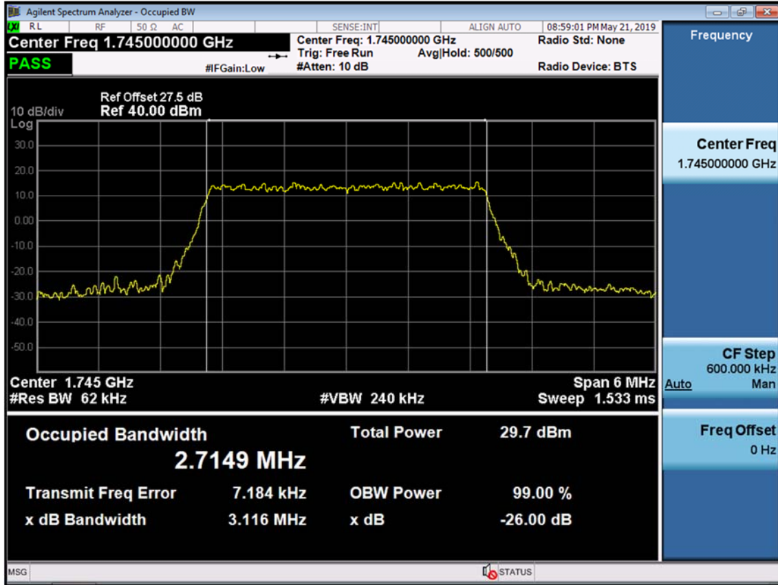
BAND 66/4. Occupied Bandwidth Plot (3M BW Ch.132322 16QAM RB 15)
