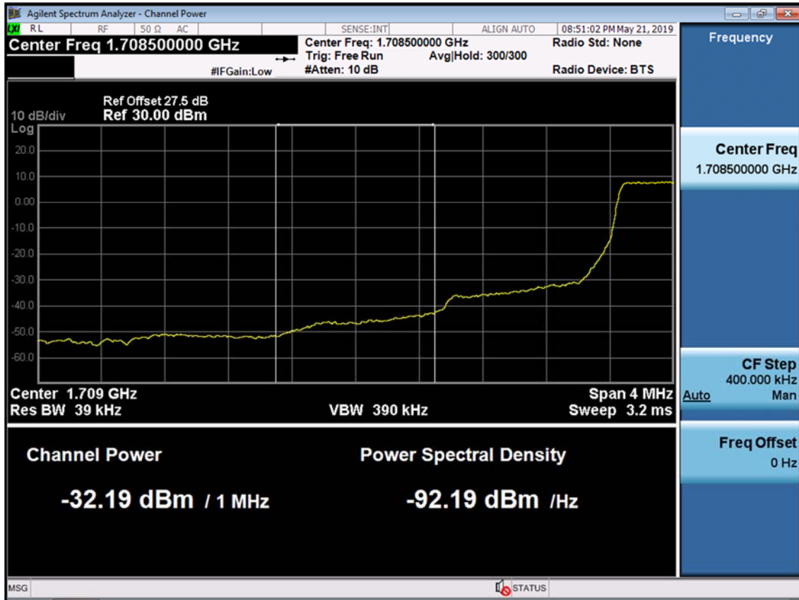
BAND 66/4. Lower Extended Band Edge Plot (1.4M BW Ch.131979 QPSK_RB6_0) -3
