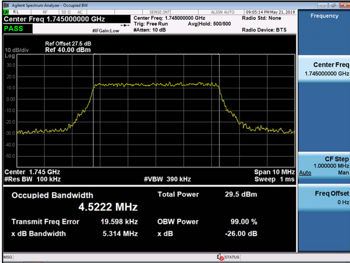
BAND 66/4. Occupied Bandwidth Plot (5M BW Ch.132322 16QAM RB 25)
