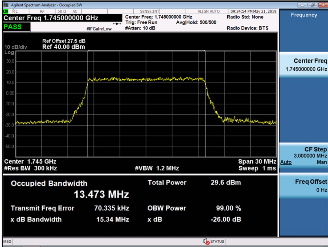
BAND 66/4. Occupied Bandwidth Plot (15M BW Ch.132322 16QAM RB 75)
