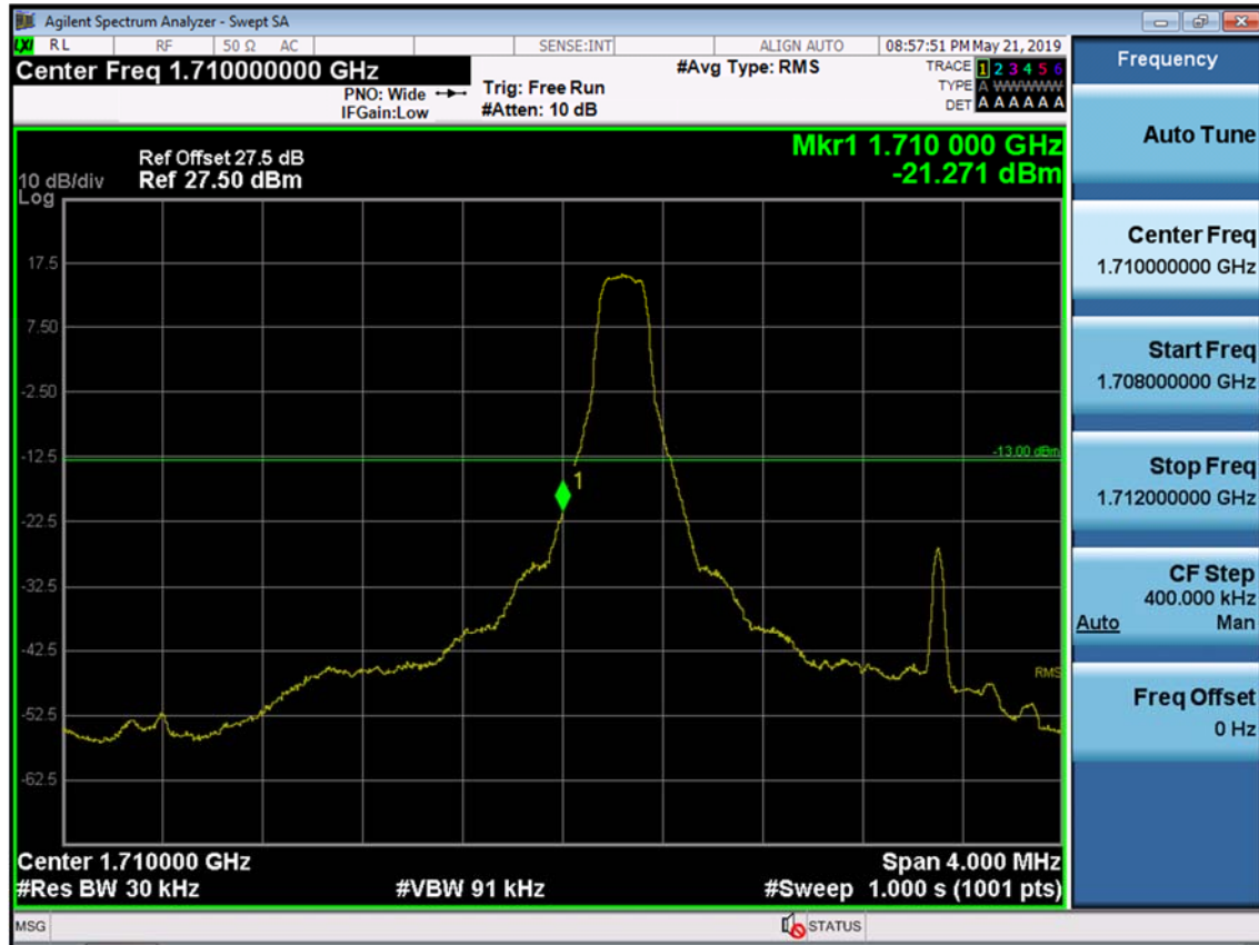
BAND 66/4. Lower Band Edge Plot (3M BW Ch.131987 QPSK RB 1, Offset 0) -1
