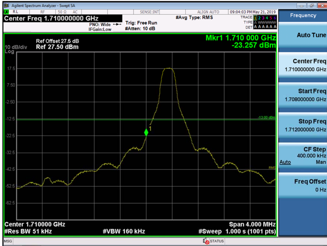
BAND 66/4. Lower Band Edge Plot (5M BW Ch.131997 QPSK RB 1, Offset 0) -1
