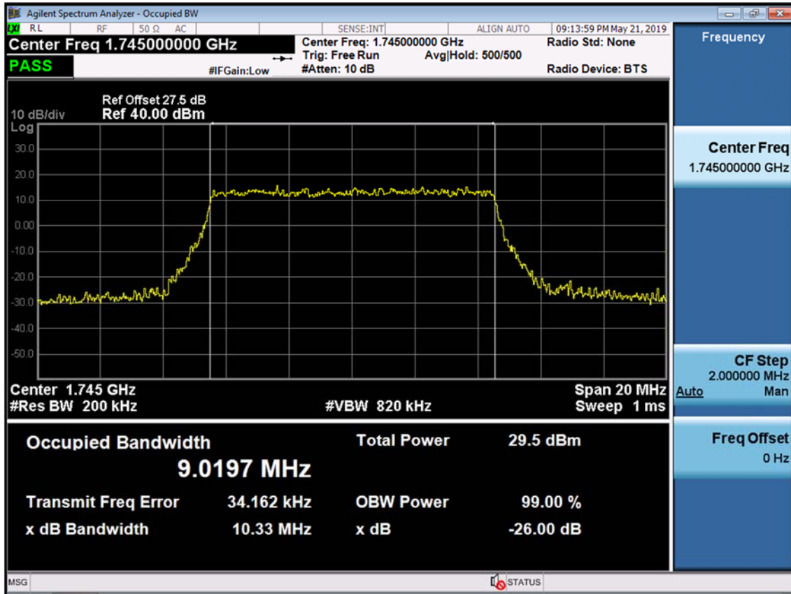
BAND 66/4. Occupied Bandwidth Plot (10M BW Ch.132322 16QAM RB 50)
