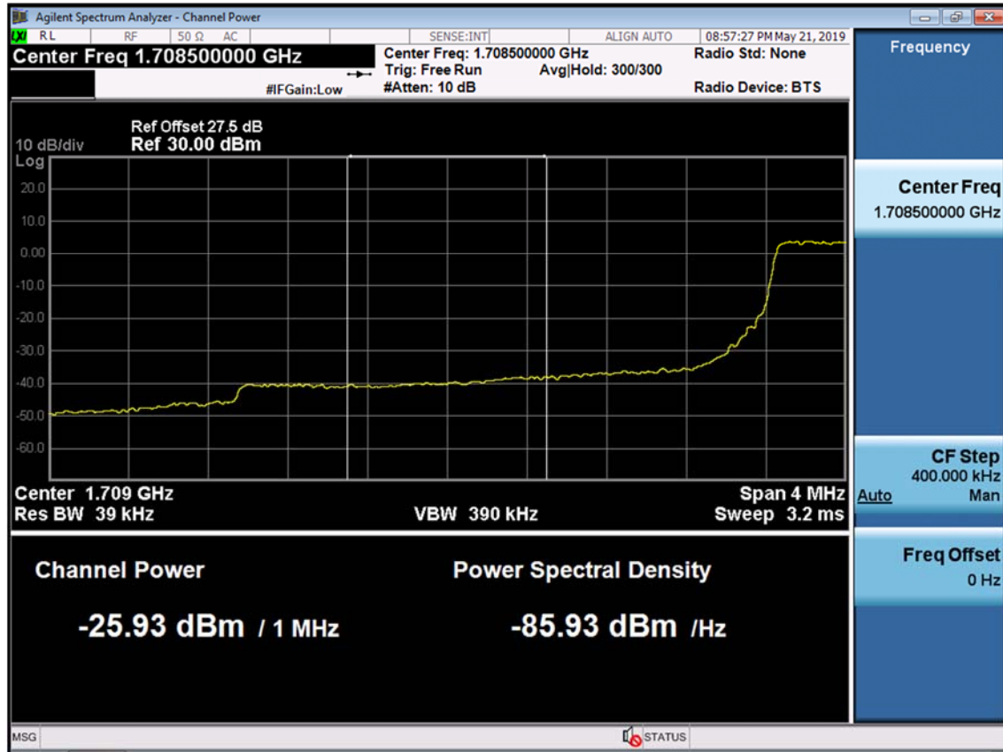
BAND 66/4. Lower Extended Band Edge Plot (3M BW Ch.131987 QPSK_RB15_0) -3
