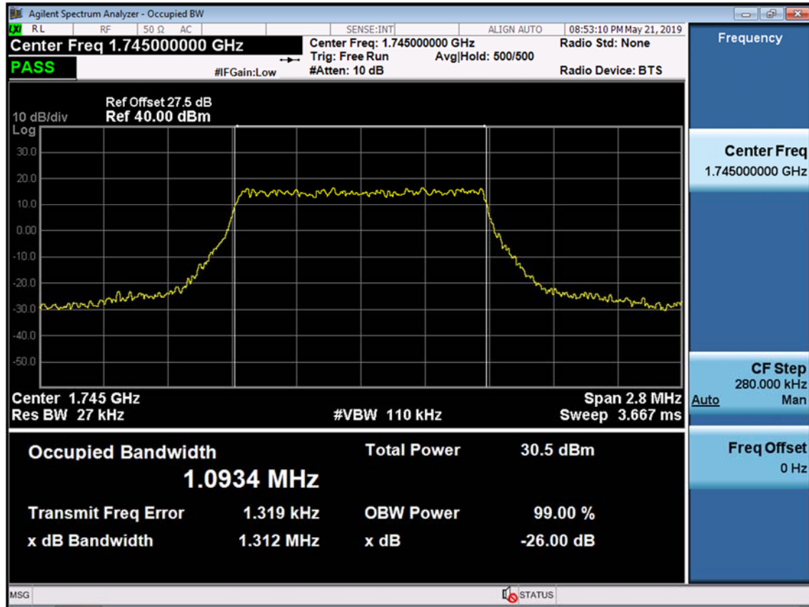
BAND 66/4. Occupied Bandwidth Plot (1.4M BW Ch.132322 QPSK RB 6)
