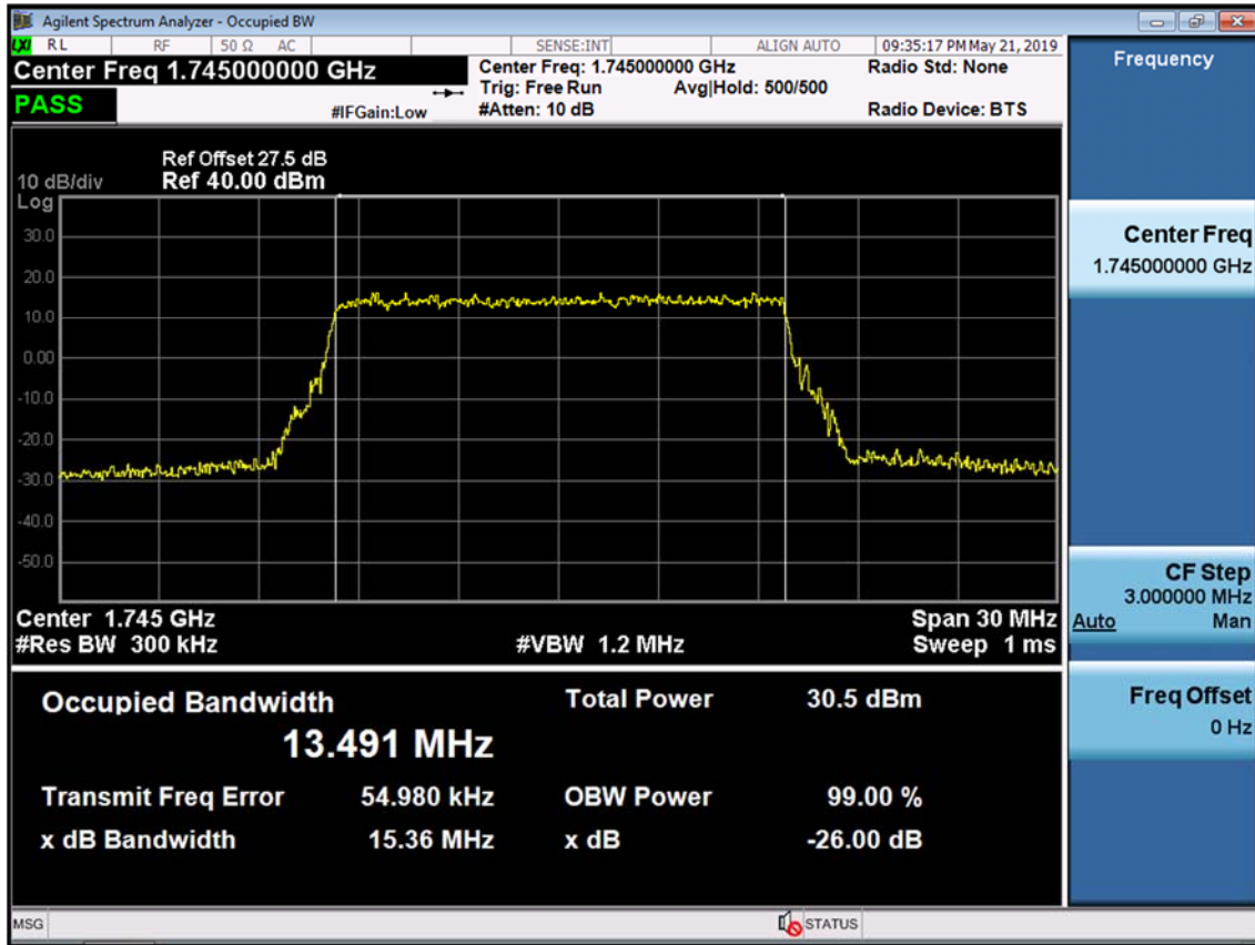
BAND 66/4. Occupied Bandwidth Plot (15M BW Ch.132322 QPSK RB 75)
