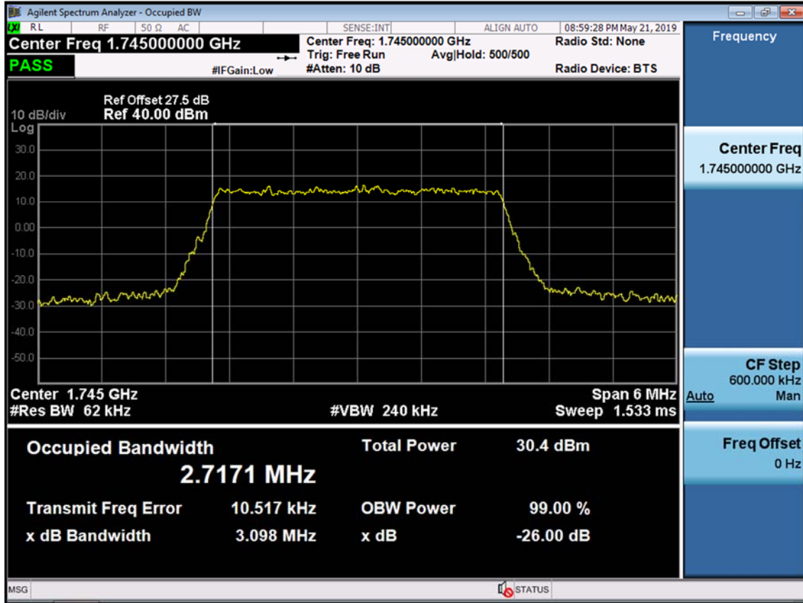
BAND 66/4. Occupied Bandwidth Plot (3M BW Ch.132322 QPSK RB 15)
