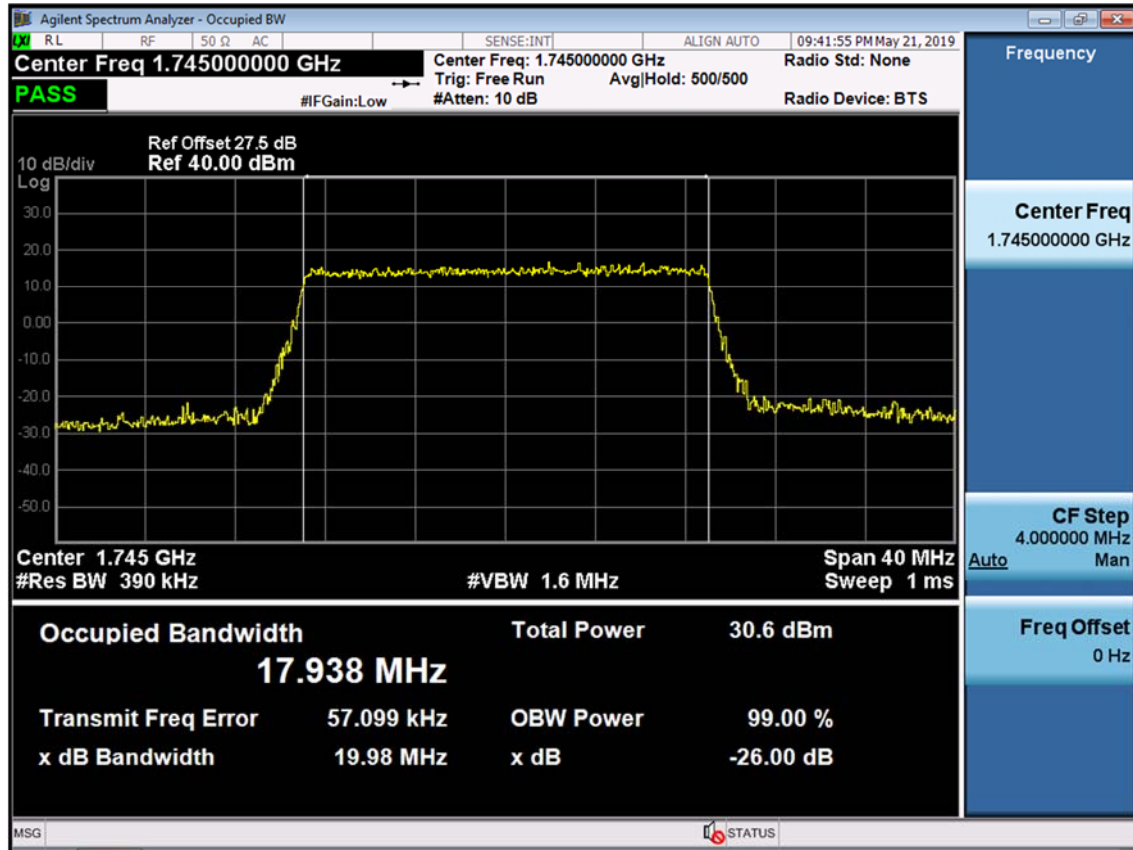
BAND 66/4. Occupied Bandwidth Plot (20M BW Ch.132322 QPSK RB 100)
