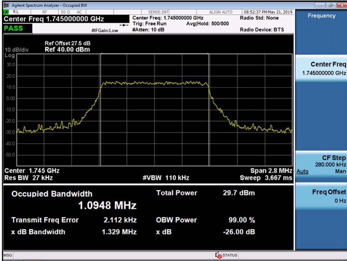
BAND 66/4. Occupied Bandwidth Plot (1.4M BW Ch.132322 16QAM RB 6)
