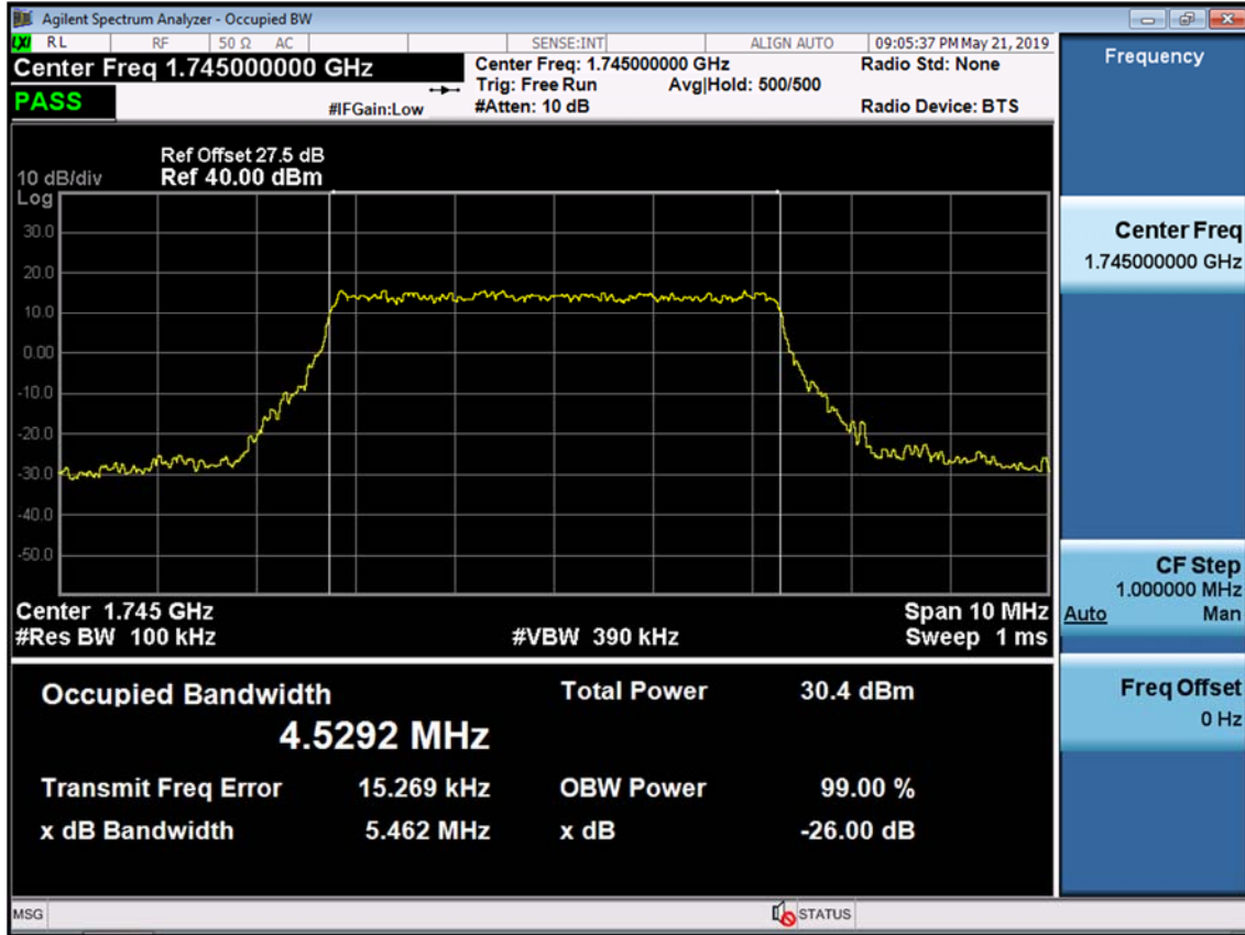
BAND 66/4. Occupied Bandwidth Plot (5M BW Ch.132322 QPSK RB 25)
