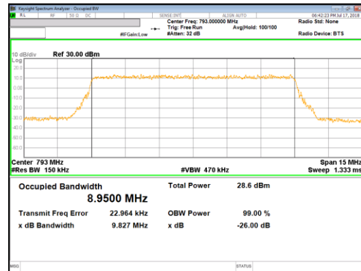
10MHz 16QAM Mid channel
