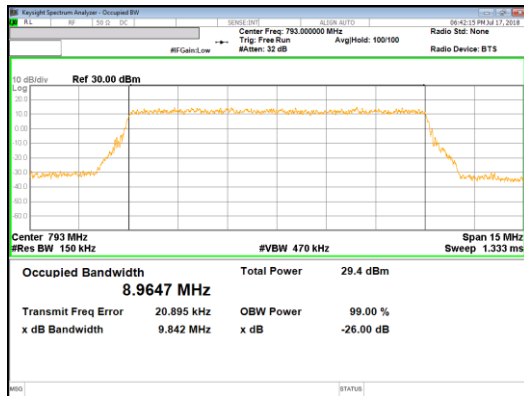
10MHz QPSK Mid channel
