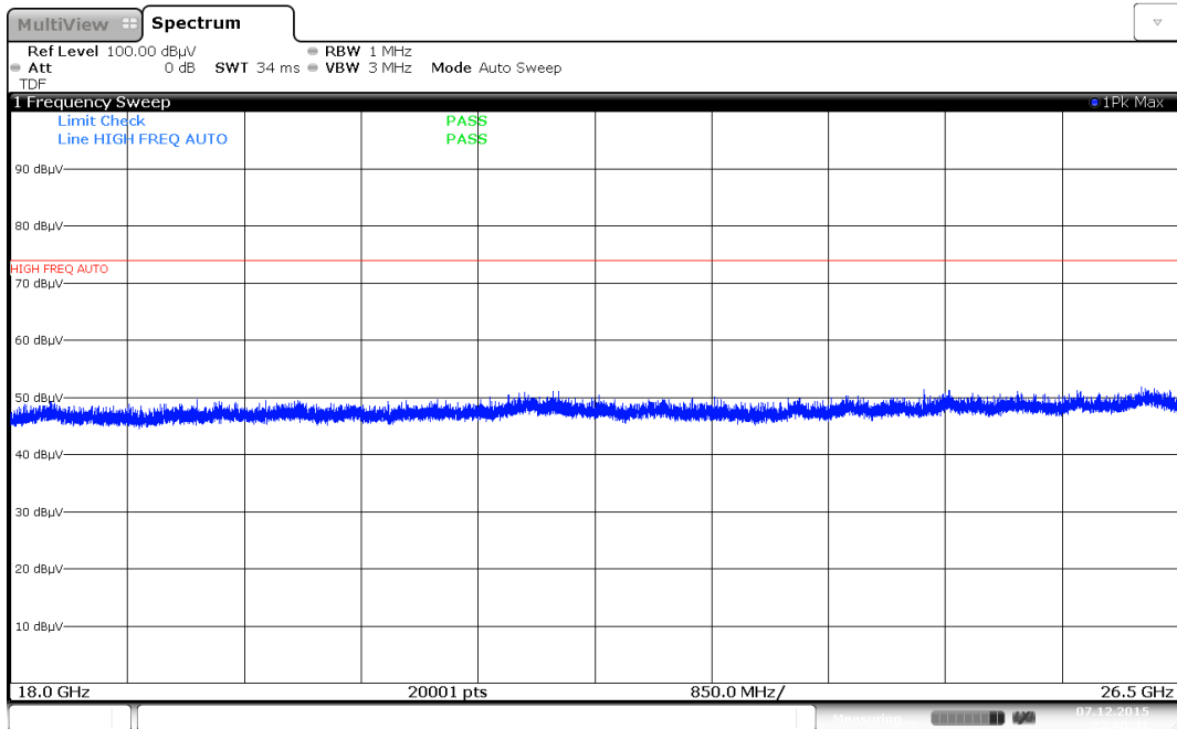
Plot 7-76. Radiated Spurious Plot from 18GHz – 26.5 GHz (802.11a – Ant. Pol. V)
