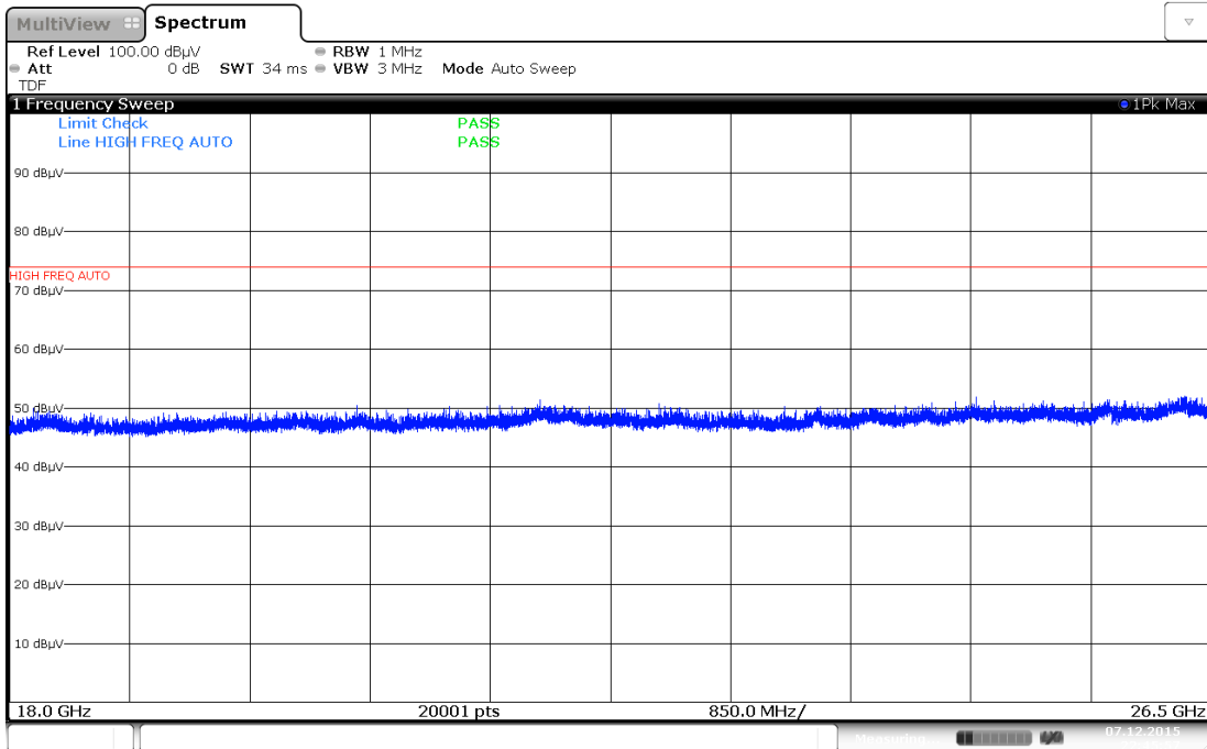
Plot 7-75. Radiated Spurious Plot from 18GHz – 26.5 GHz (802.11a – Ant. Pol. H)
