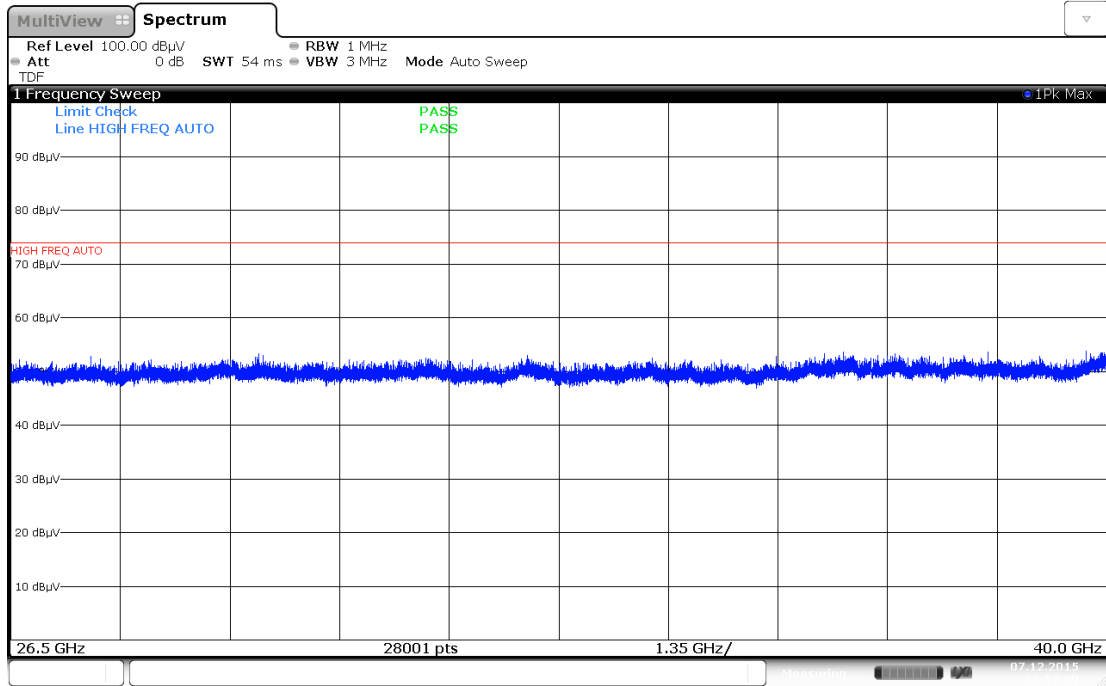
Plot 7-77. Radiated Spurious Plot above 26.5GHz (802.11a – Ant. Pol. H)
