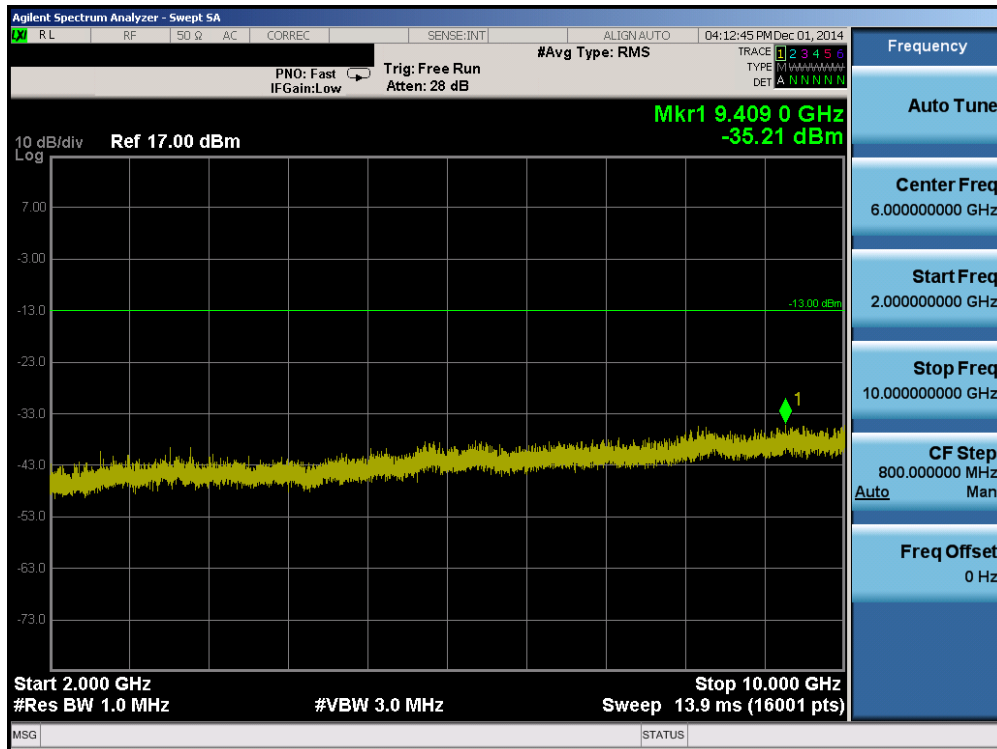
Plot 6-13. Conducted Spurious Plot (Cellular GPRS Mode – Ch. 190)
