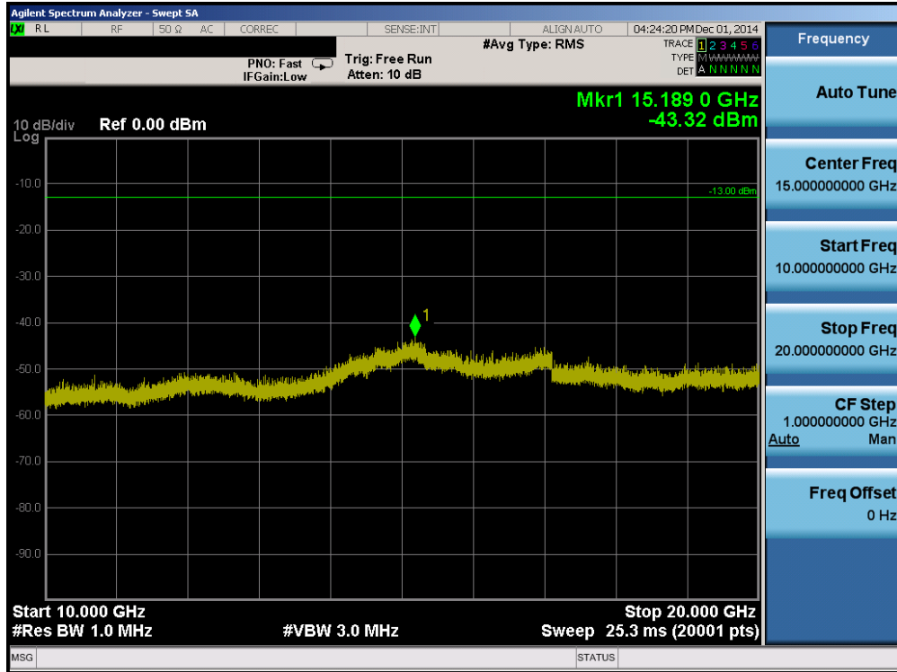
Plot 6-20. Conducted Spurious Plot (PCS GPRS Mode – Ch. 661)
