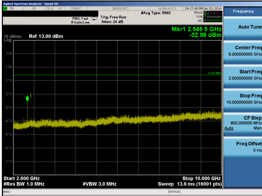
Plot 6-16. Conducted Spurious Plot (Cellular GPRS Mode – Ch. 251)
