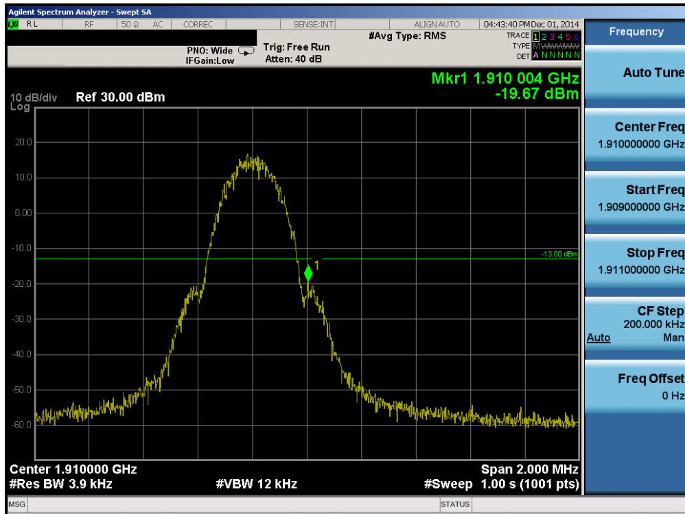
Plot 6-44. Band Edge Plot (PCS GPRS Mode – Ch. 810)
