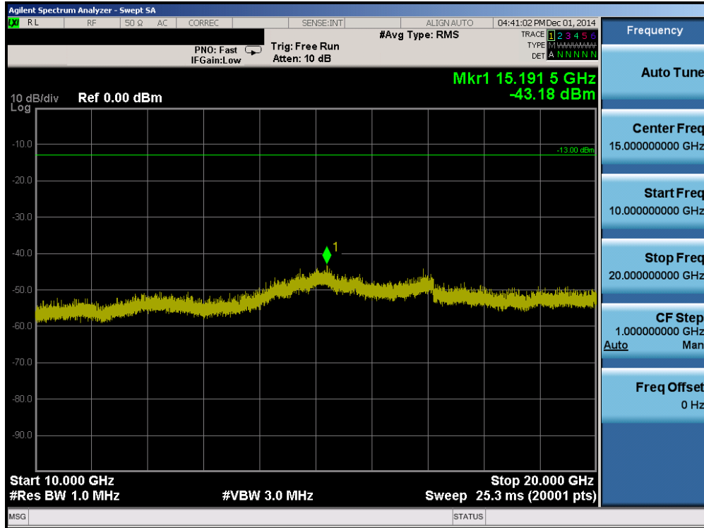
Plot 6-18. Conducted Spurious Plot (PCS GPRS Mode – Ch. 512)
