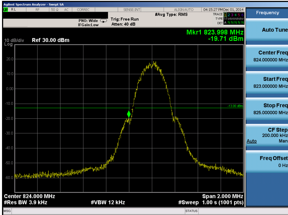
Plot 6-41. Band Edge Plot (Cellular GPRS Mode – Ch. 128)
