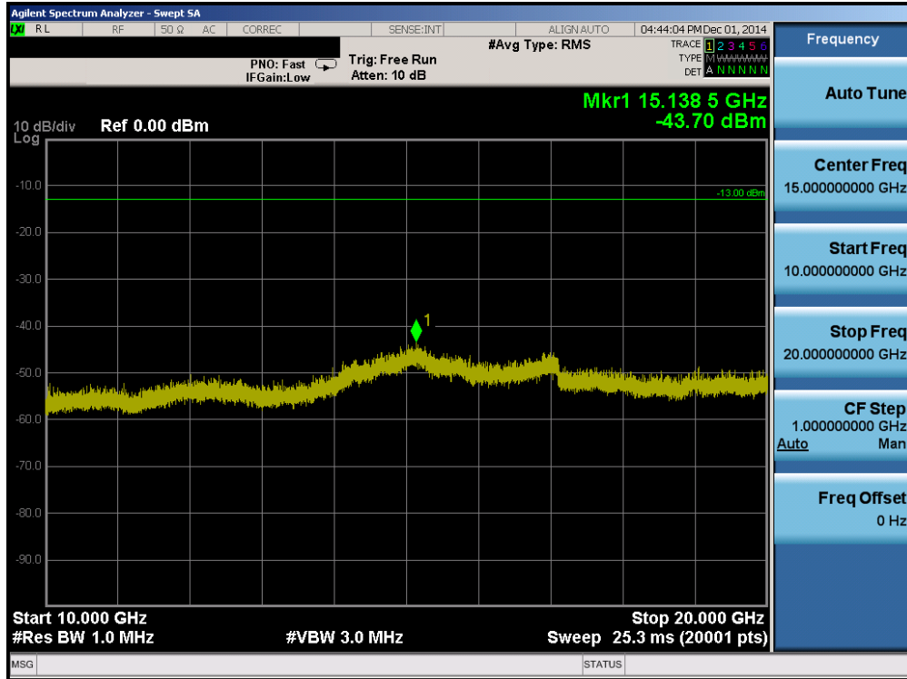
Plot 6-22. Conducted Spurious Plot (PCS GPRS Mode – Ch. 810)
