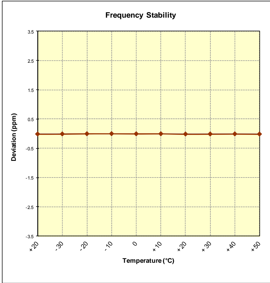
Figure 6-10. Frequency Stability Graph (PCS GPRS Mode – Ch. 661)
