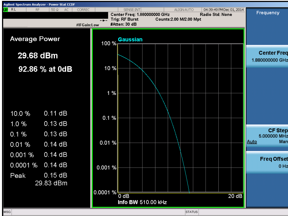
Plot 6-55. Peak-Average Ratio Plot (PCS GPRS Mode – Ch. 661)
