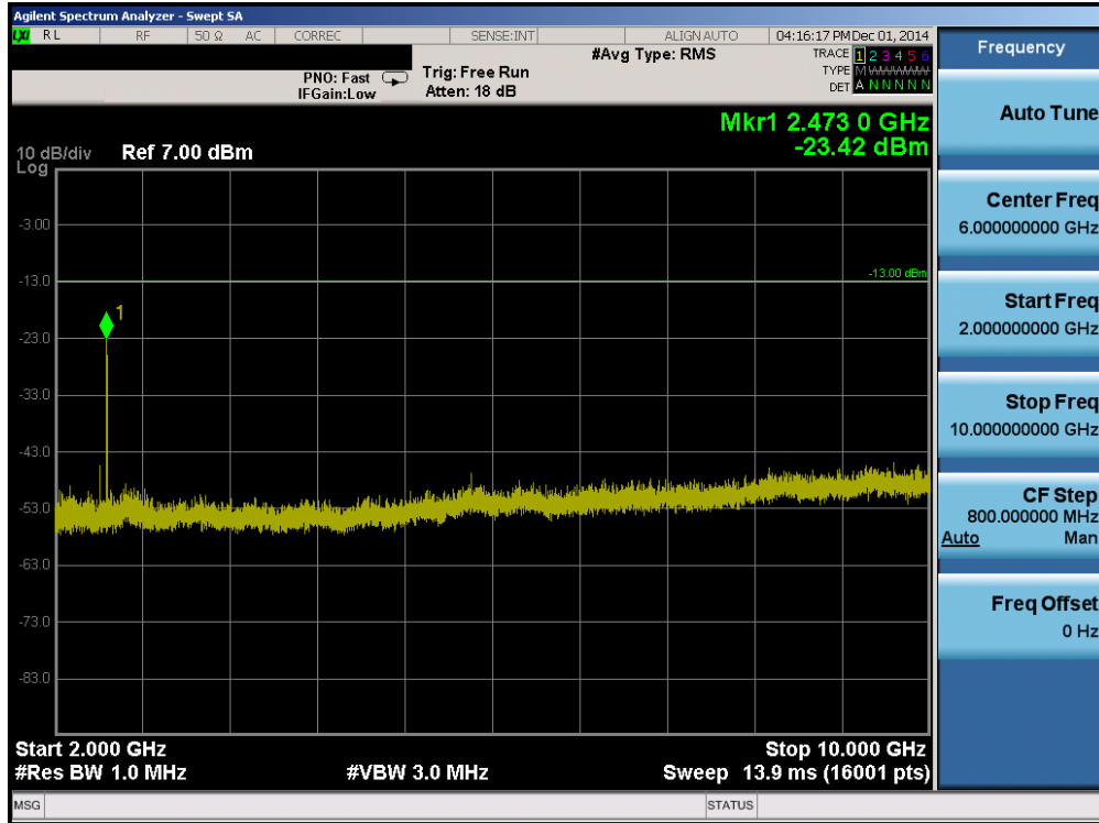
Plot 6-10. Conducted Spurious Plot (Cellular GPRS Mode – Ch. 128)
