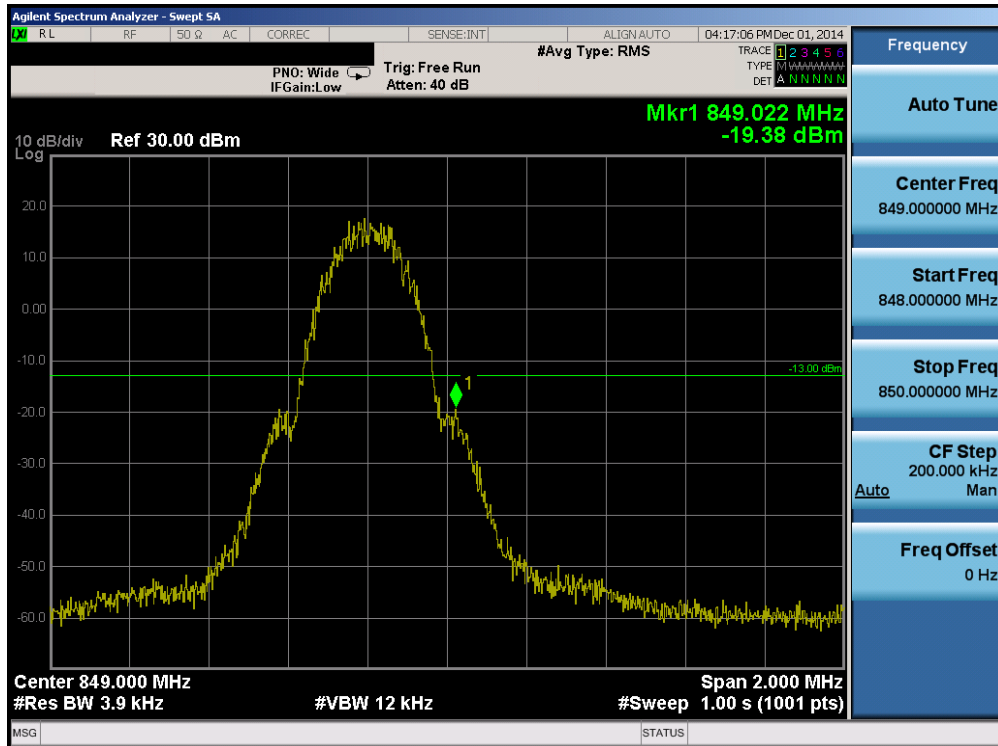
Plot 6-42. Band Edge Plot (Cellular GPRS Mode – Ch. 251)
