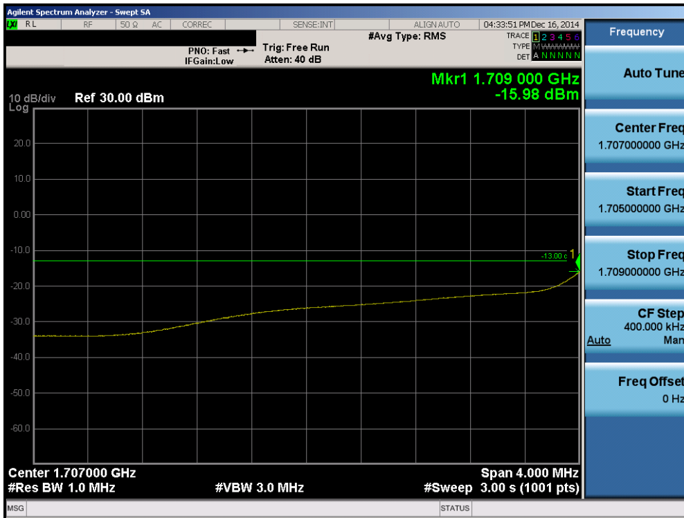
Plot 6-48. Band Edge Plot (AWS WCDMA Mode – Ch. 1312)
