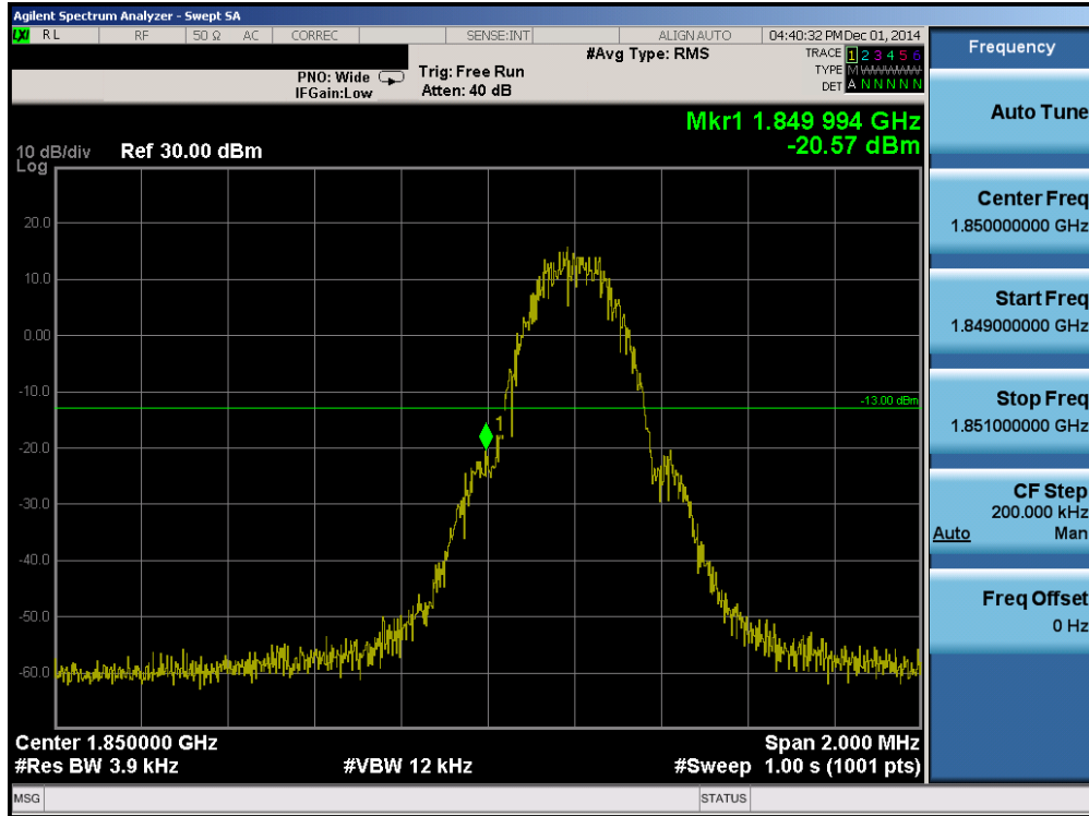
Plot 6-43. Band Edge Plot (PCS GPRS Mode – Ch. 512)
