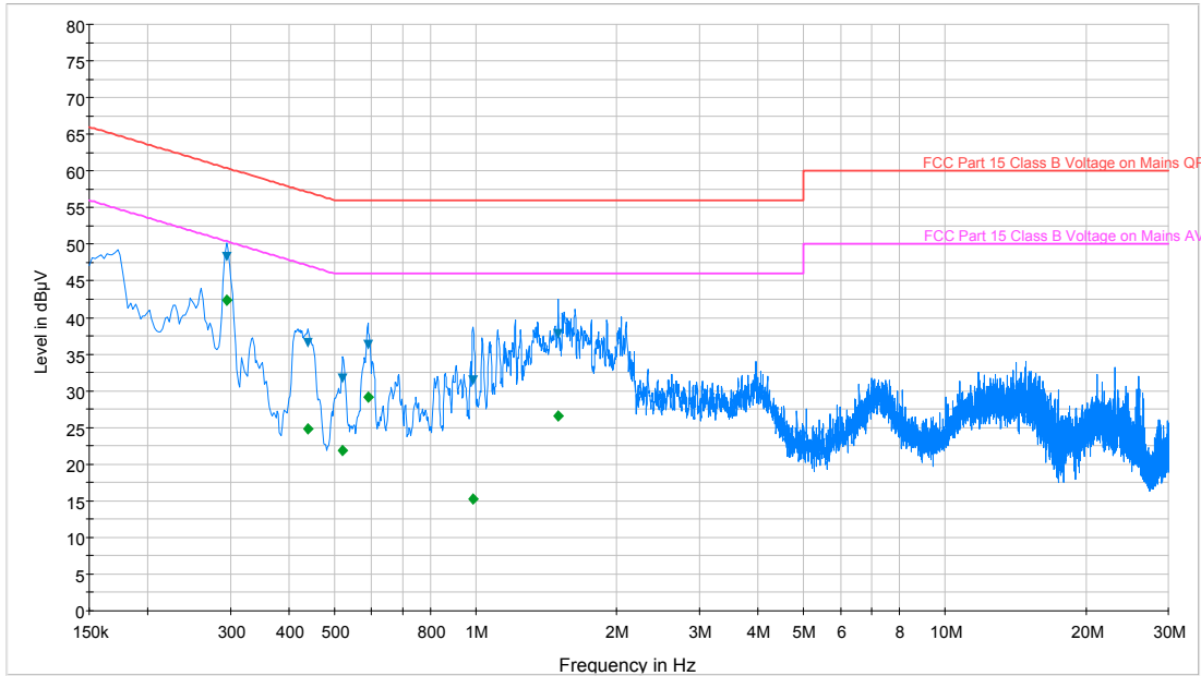
— FCC Part 15 Class B Voltage on Mains QP.LimitLine — FCC Part 15 Class B Voltage on Mains AV.LimitLine — Preview Result 1-PK+ ◆ Final Result 2-AVG
