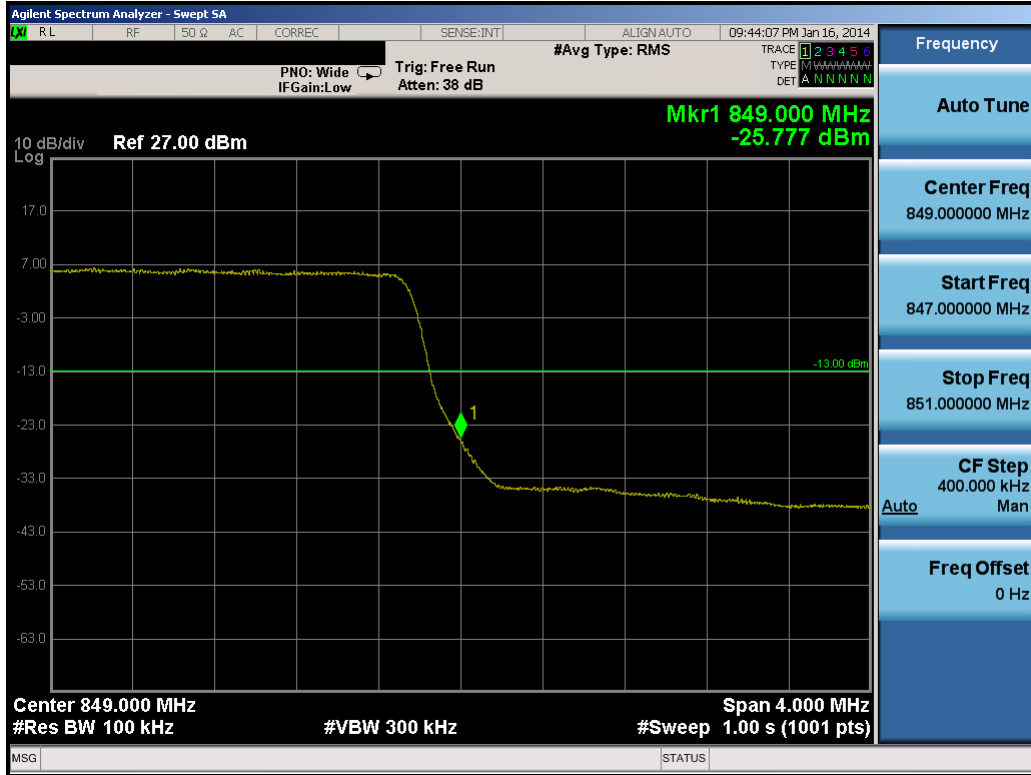
Plot 7-12. Upper Band Edge Plot (5.0MHz QPSK – RB Size 25)
