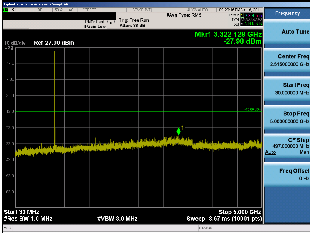
Plot 7-16. Conducted Spurious Plot (10.0MHz QPSK – RB Size 1, RB Offset 0– Low Channel)
