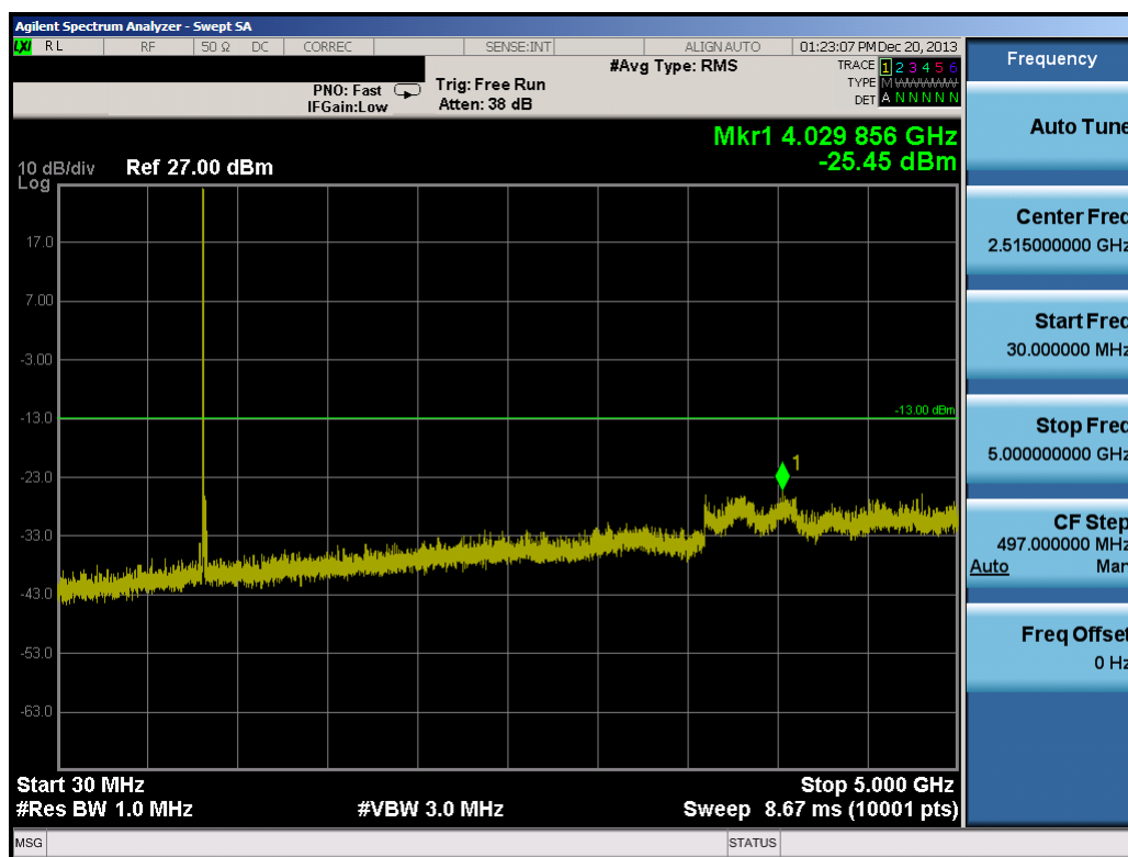
Plot 7-14. Conducted Spurious Plot (5.0MHz QPSK – RB Size 1, RB Offset 0 – Mid Channel)
