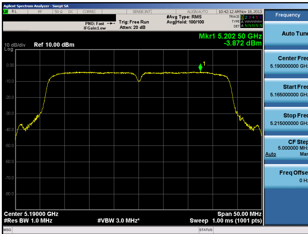
Plot 6-38. Peak Power Spectral Density Plot (40MHz BW 802.11n (UNII Band 1) – Ch. 38)
