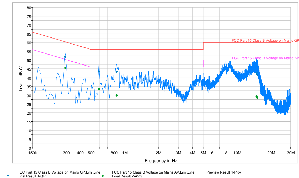
Plot 6-89. Line Conducted Plot with 802.11a UNII Band 2C (N)
