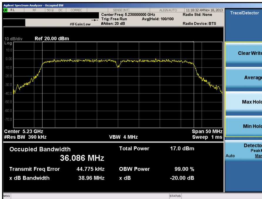
Plot 6-30. 20dB Bandwidth Plot (40MHz BW 802.11n (UNII Band 2A) – Ch. 46)
