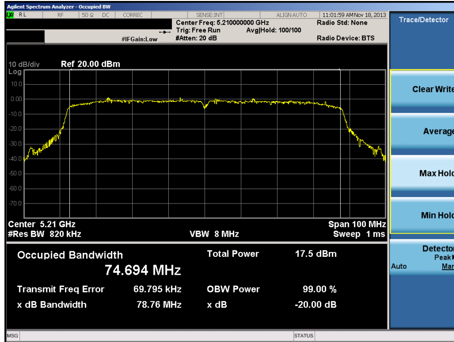
Plot 6-31. 20dB Bandwidth Plot (80MHz BW 802.11n (UNII Band 2A) – Ch. 42)
