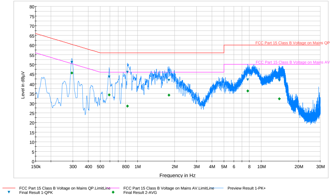
Plot 6-88. Line Conducted Plot with 802.11a UNII Band 2C (L1)
