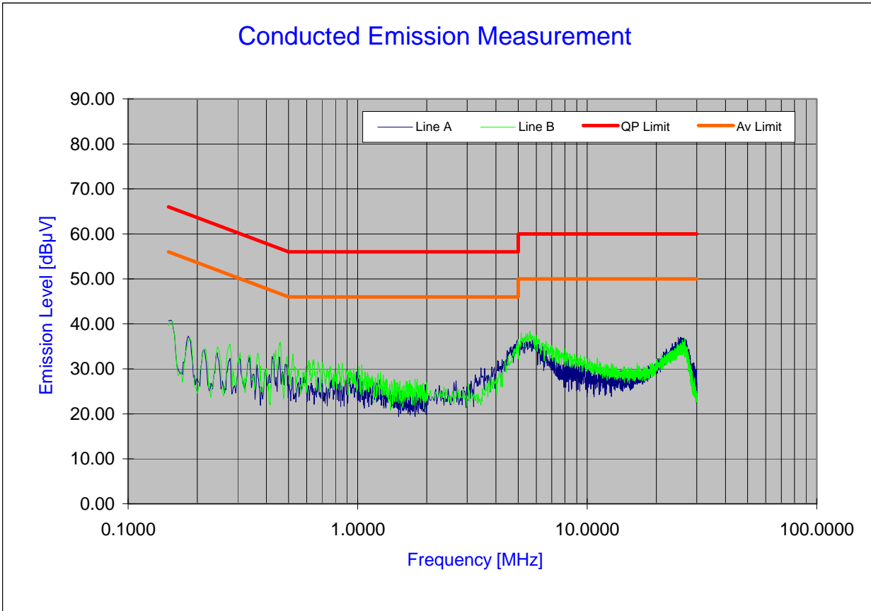
Plot 6-62. Line Conducted Plot with 802.11b
