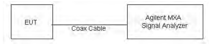
Figure 6-5. Test Instrument & Measurement Setup
