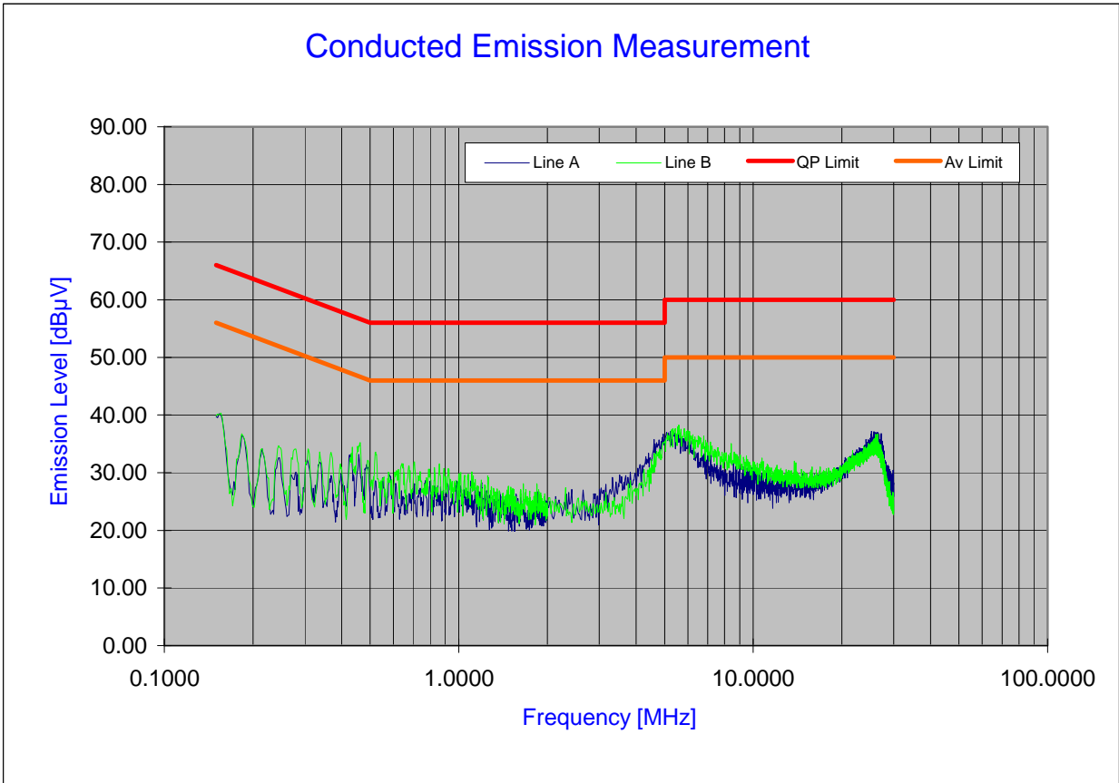
Plot 6-61. Line Conducted Plot with 802.11a
