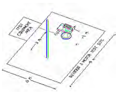
Figure 3-7. Turntable and System Setup
