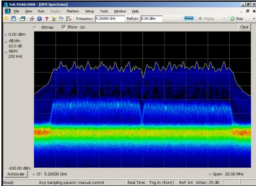
Figure 5-3. Real-Time Spectrum Display, WLAN Traffic (Streaming Video)
