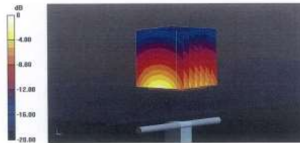
0 dB = 14.9 W/kg = 11.73 dBW/kg
