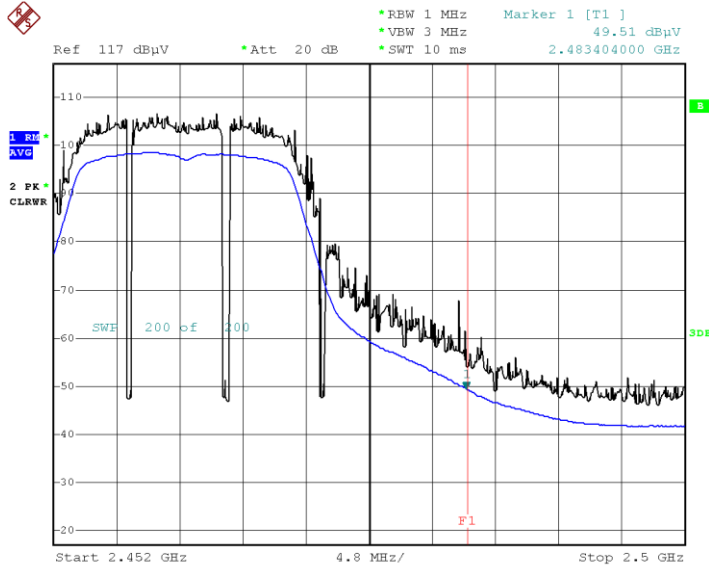
Radiated Restricted Band Edges plot – Average Reading (802.11g_6Mbps Ch.11)
