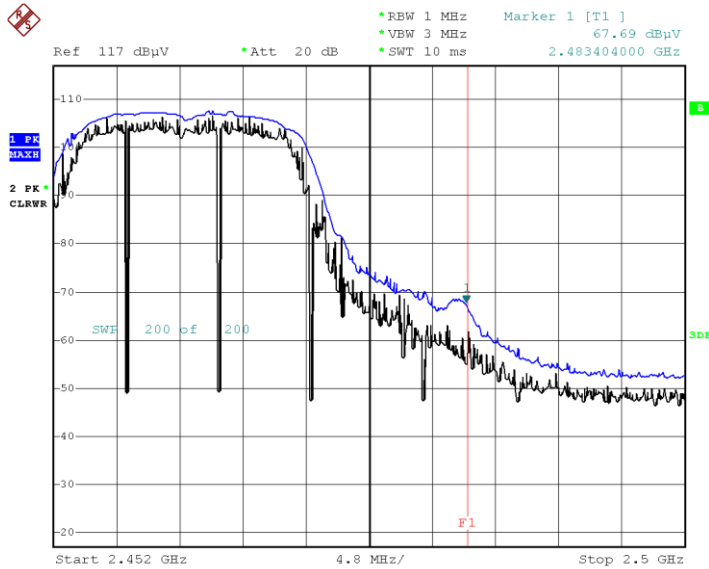
Radiated Restricted Band Edges plot – Peak Reading (802.11g_6Mbps Ch.11)
