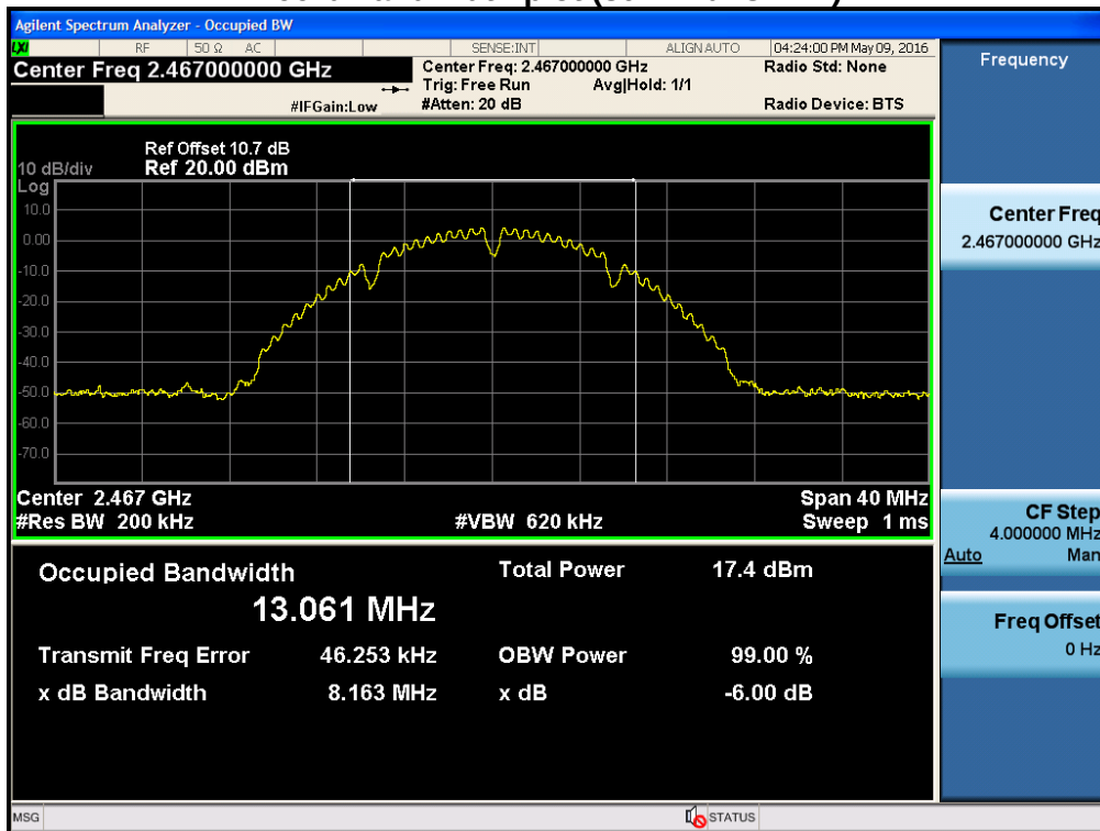
99% Bandwidth plot (802.11b- CH 12)
