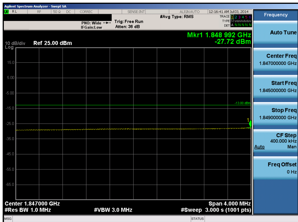
Plot 6-22. Lower Extended Band Edge Plot (Band 25 – 20.0MHz QPSK – RB Size 100)
