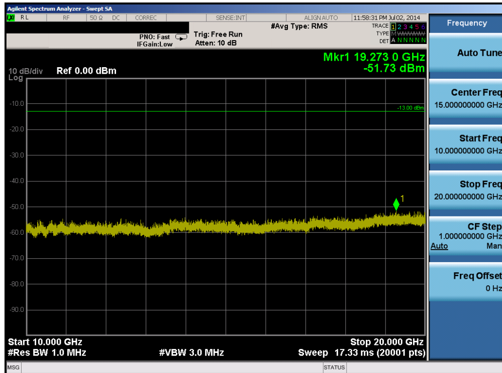
Plot 6-10. Conducted Spurious Plot (Band 25 – 15.0MHz QPSK – RB Size 1, RB Offset 0 – Mid Channel)
