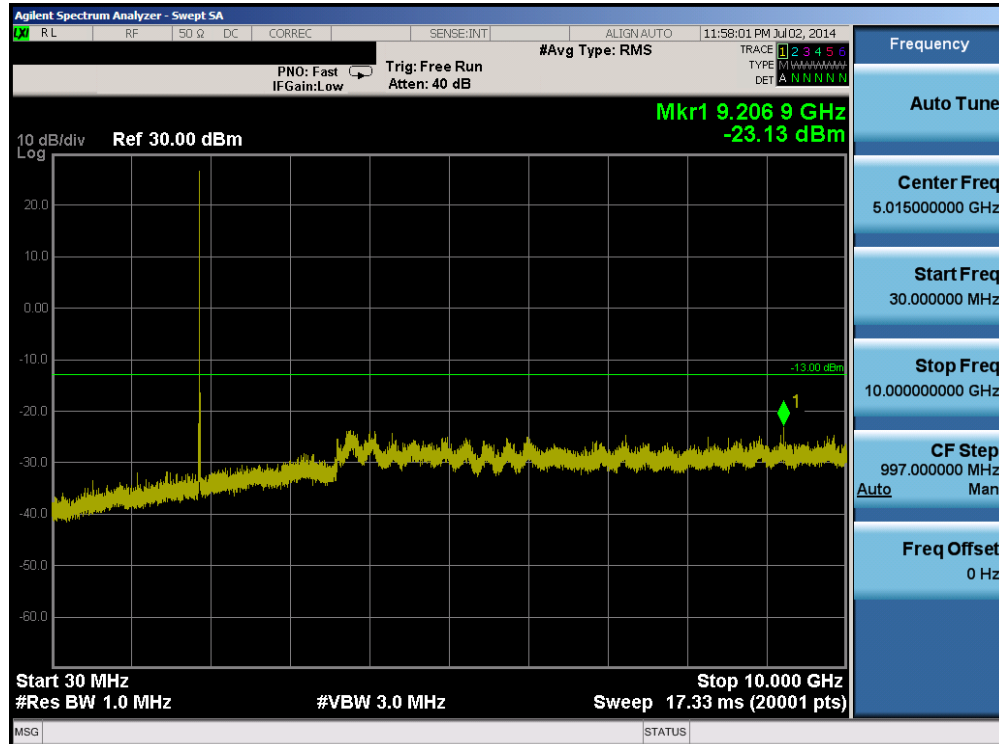
Plot 6-9. Conducted Spurious Plot (Band 25 – 15.0MHz QPSK – RB Size 1, RB Offset 0 – Mid Channel)
