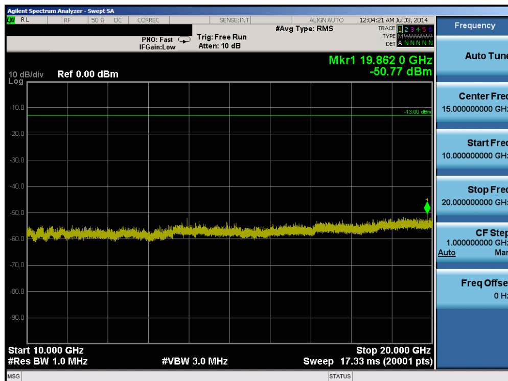
Plot 6-12. Conducted Spurious Plot (Band 25 – 15.0MHz QPSK – RB Size 1, RB Offset 0 – High Channel)
