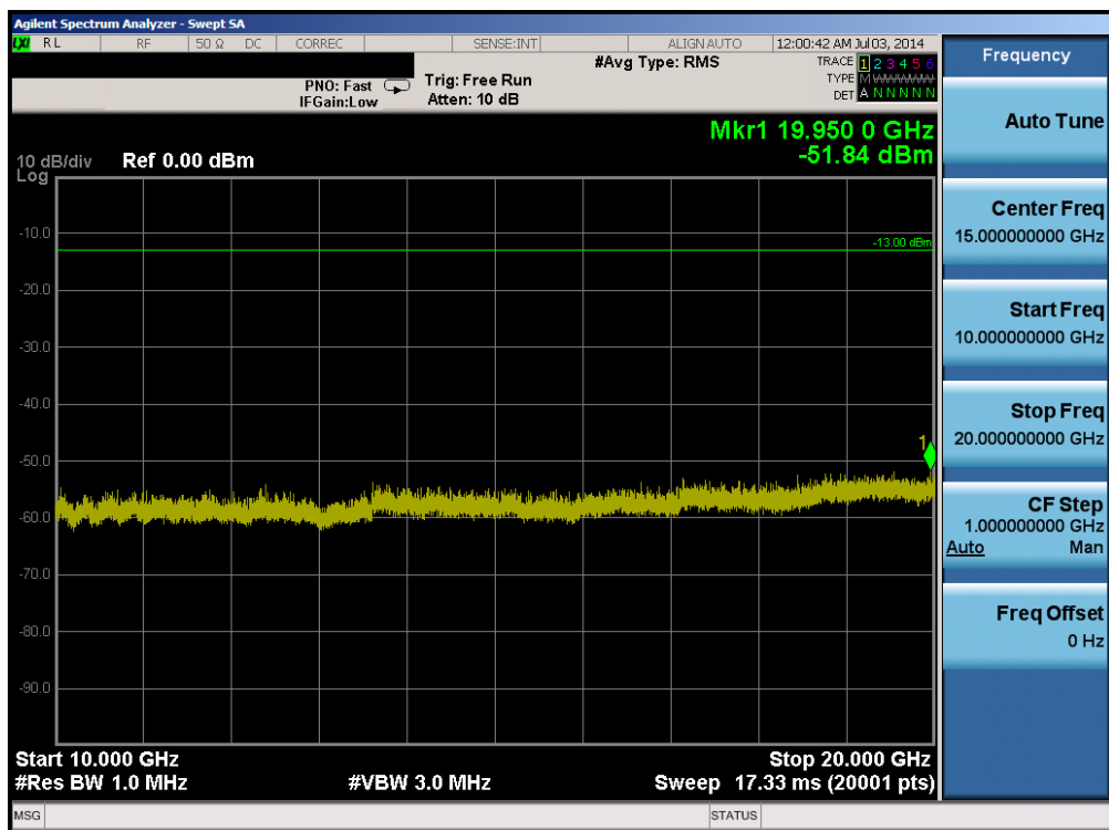
Plot 6-8. Conducted Spurious Plot (Band 25 – 15.0MHz QPSK – RB Size 1, RB Offset 0 – Low Channel)
