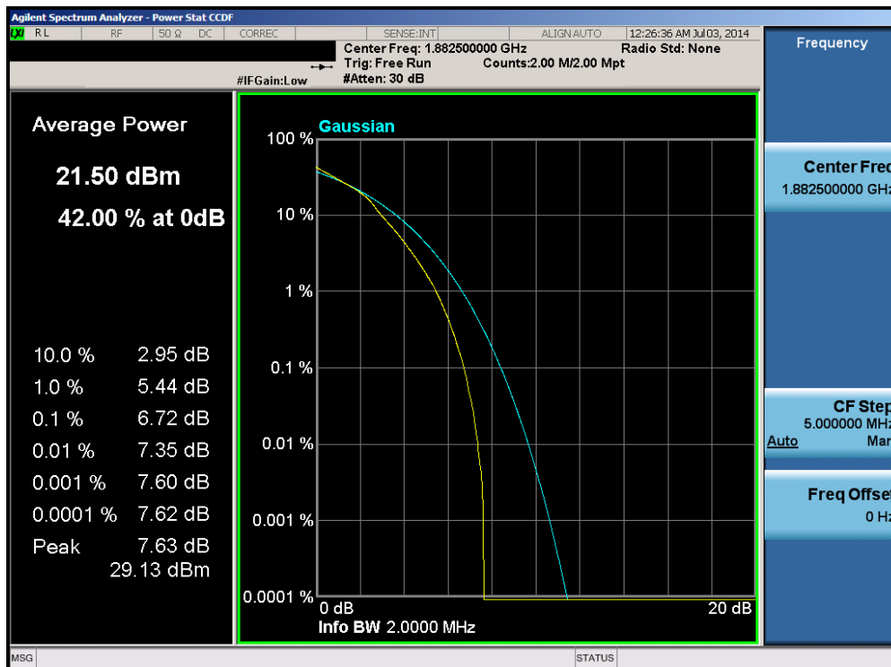
Plot 6-26. PAR Plot (Band 25 – 1.4MHz 16-QAM – RB Size 6)
