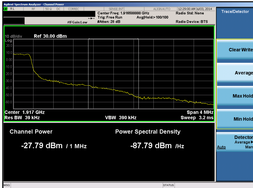
Plot 6-16. Upper Extended Band Edge Plot (Band 25 – 1.4MHz QPSK – RB Size 6)
