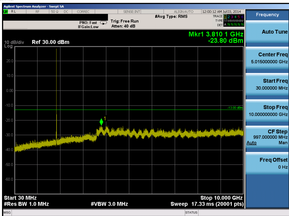
Plot 6-7. Conducted Spurious Plot (Band 25 – 15.0MHz QPSK – RB Size 1, RB Offset 0 – Low Channel)
