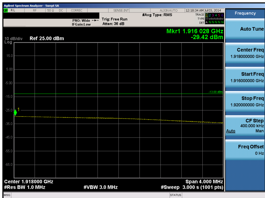
Plot 6-24. Upper Extended Band Edge Plot (Band 25 – 20.0MHz QPSK – RB Size 100)
