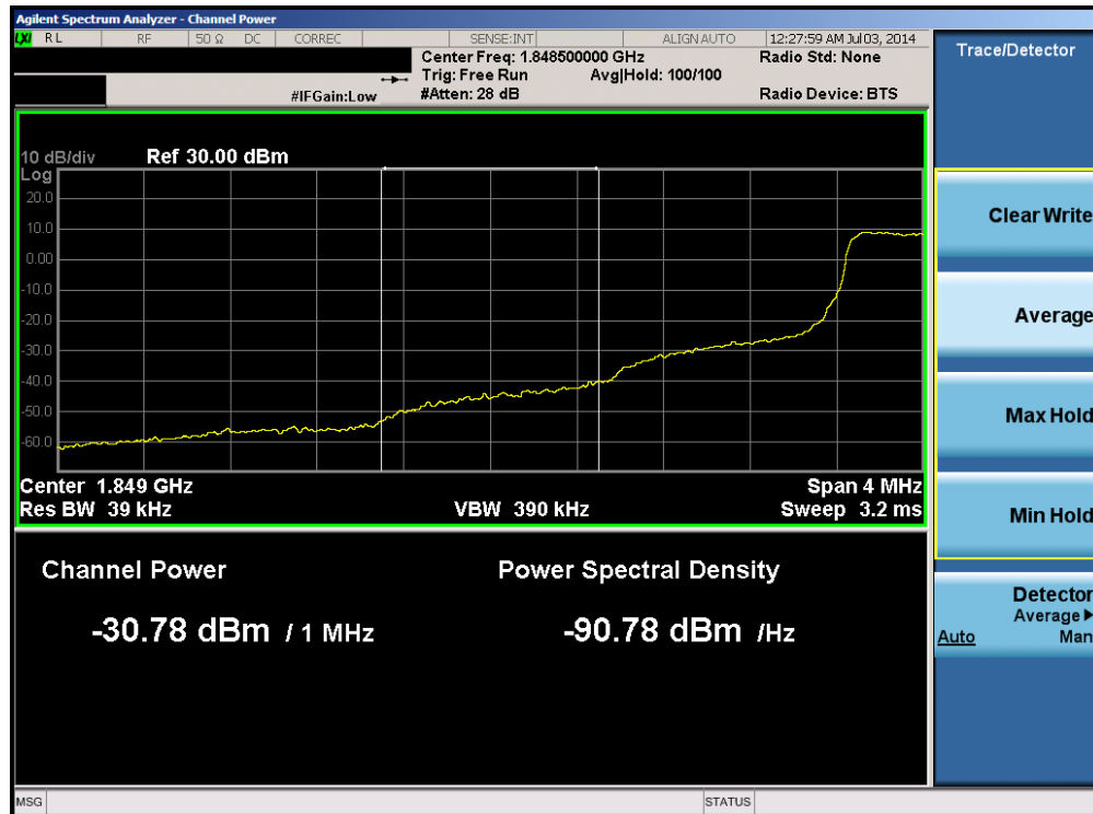
Plot 6-14. Lower Extended Band Edge Plot (Band 25 – 1.4MHz QPSK – RB Size 6)
