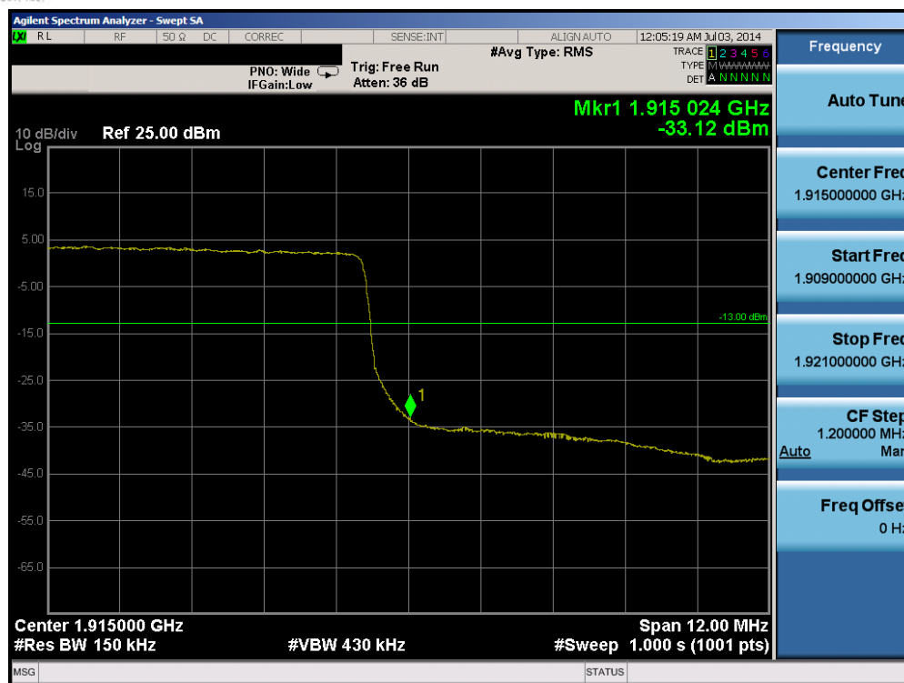
Plot 6-19. Upper Band Edge Plot (Band 25 – 15.0MHz QPSK – RB Size 75)
