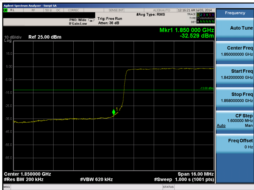
Plot 6-21. Lower Band Edge Plot (Band 25 – 20.0MHz QPSK – RB Size 100)
