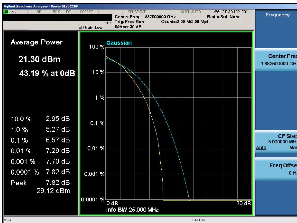
Plot 6-28. PAR Plot (Band 25 – 15.0MHz 16-QAM – RB Size 75)
