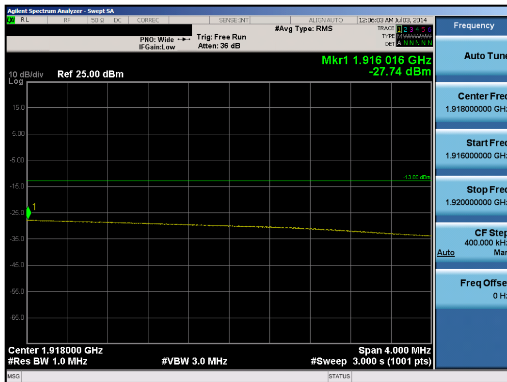
Plot 6-20. Upper Extended Band Edge Plot (Band 25 – 15.0MHz QPSK – RB Size 75)
