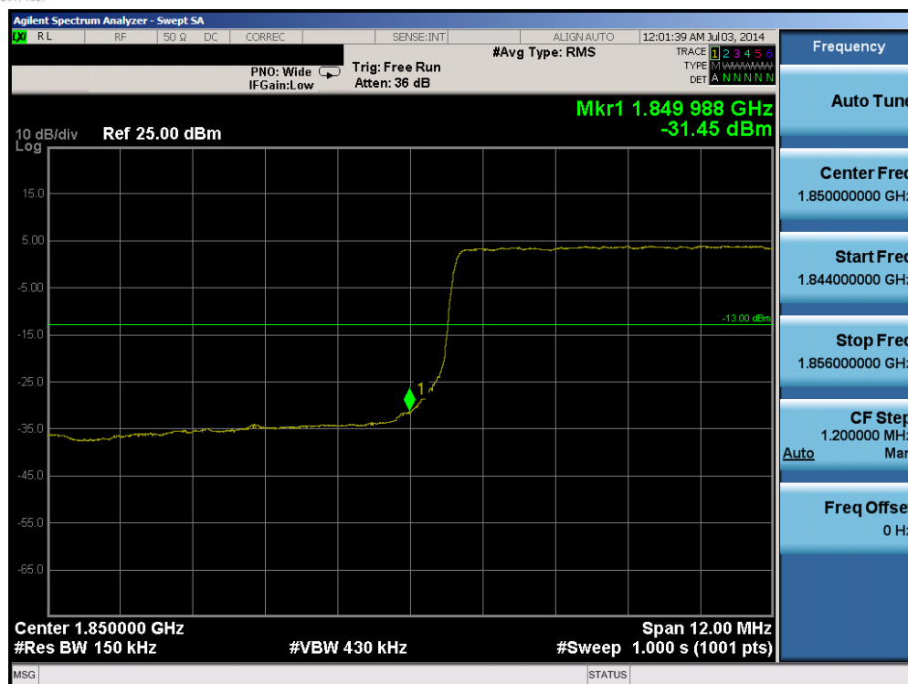
Plot 6-17. Lower Band Edge Plot (Band 25 – 15.0MHz QPSK – RB Size 75)
