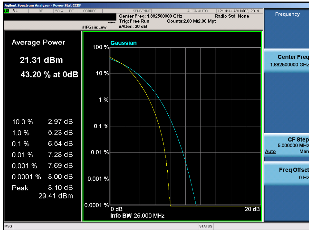
Plot 6-30. PAR Plot (Band 25 – 20.0MHz 16-QAM – RB Size 100)
