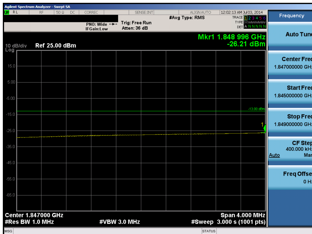
Plot 6-18. Lower Extended Band Edge Plot (Band 25 – 15.0MHz QPSK – RB Size 75)
