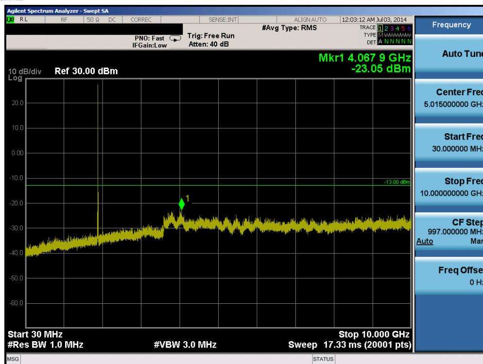
Plot 6-11. Conducted Spurious Plot (Band 25 – 15.0MHz QPSK – RB Size 1, RB Offset 0 – High Channel)
