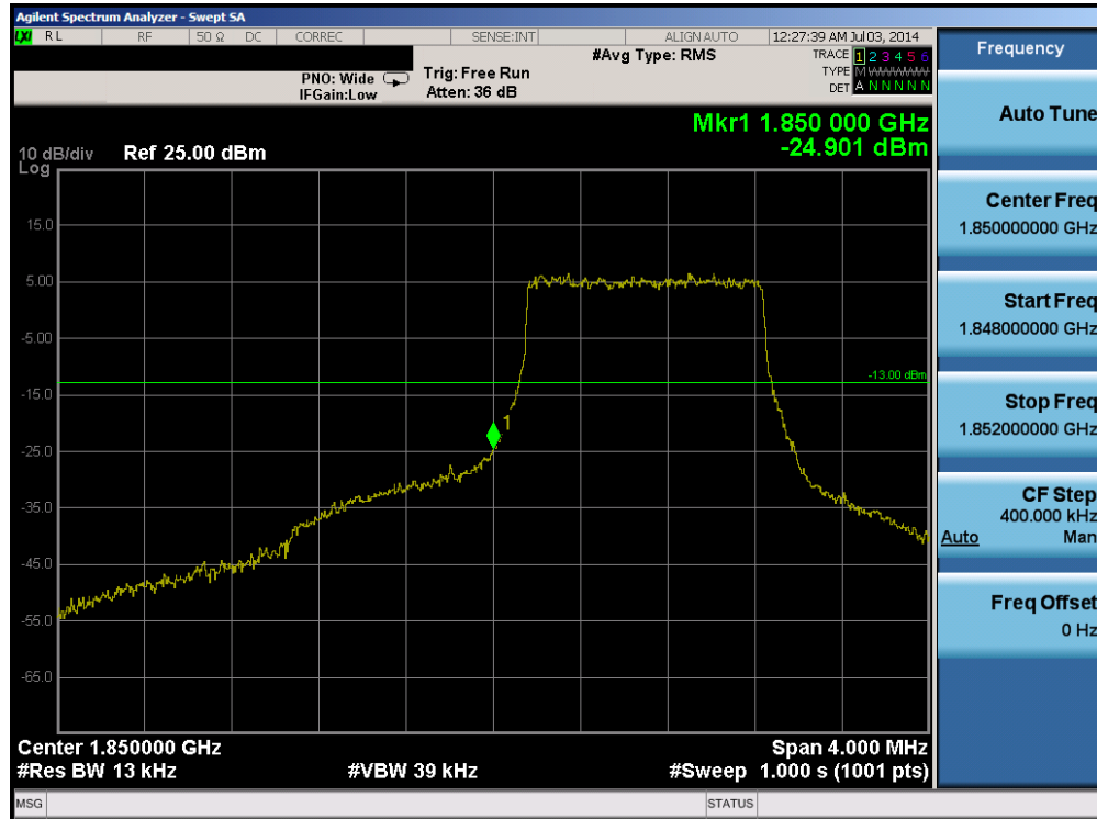
Plot 6-13. Lower Band Edge Plot (Band 25 – 1.4MHz QPSK – RB Size 6)
